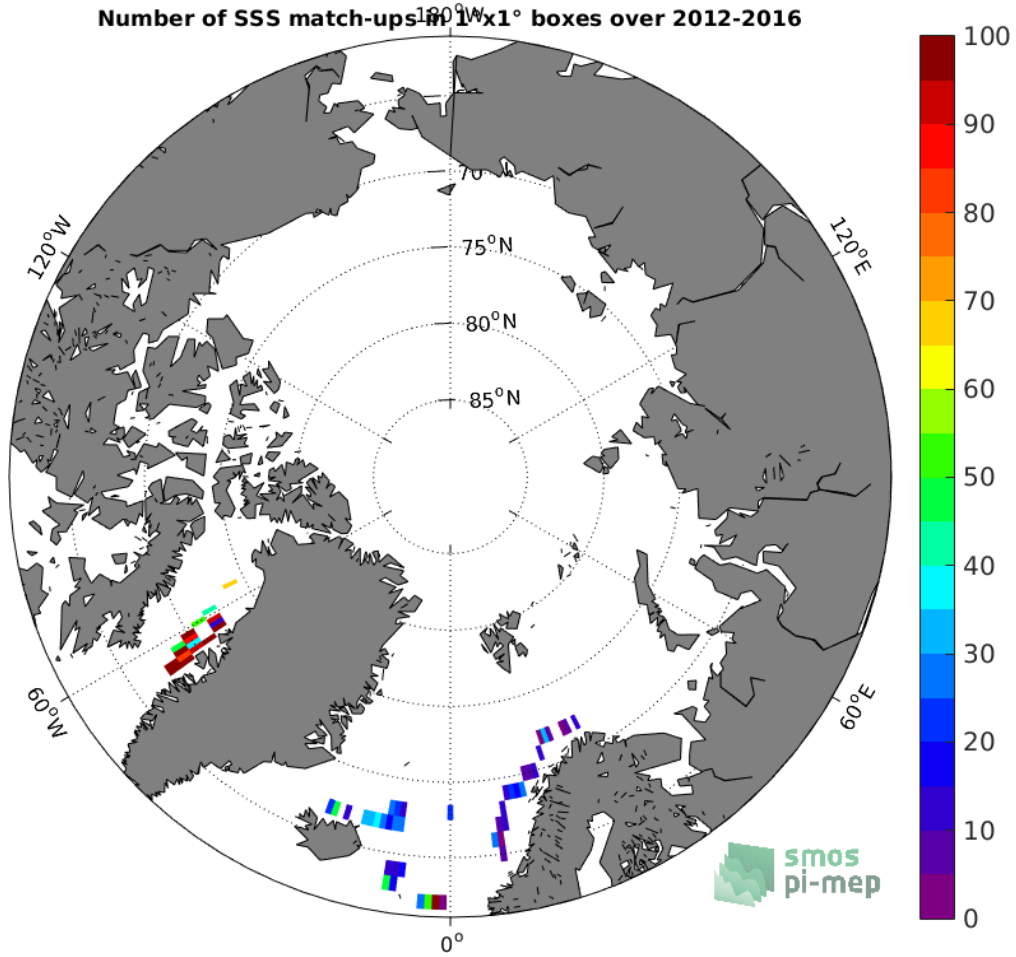
Figure 4: Number of SSS match-ups between TSG (LEGOS-DM) SSS and the SMOS SSS L2Q v321 - 0.25 Deg (CATDS-CPDC) SSS product for the Arctic Ocean Pi-MEP region over 1°x1° boxes and for the full satellite product period.
