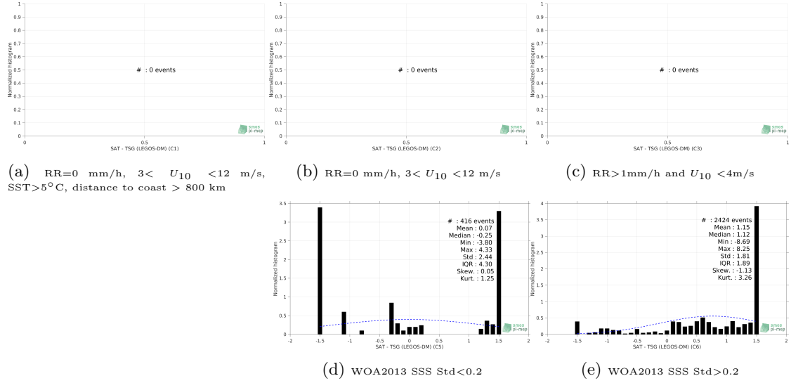
Figure 13: Normalized histogram of \Delta\text{SSS} (SMOS SSS L2Q v321 - 0.25 Deg (CATDS-CPDC) - TSG (LEGOS-DM)) for 5 different subdatasets corresponding to: RR=0 mm/h, 3 < U_{10} < 12 m/s, SST > 5^\circ\text{C} , distance to coast > 800 km (a), RR=0 mm/h, 3 < U_{10} < 12 m/s (b), RR > 1\text{mm/h} and U_{10} < 4\text{m/s} (c), WOA2013 SSS Std<0.2 (d), WOA2013 SSS Std>0.2 (e).
