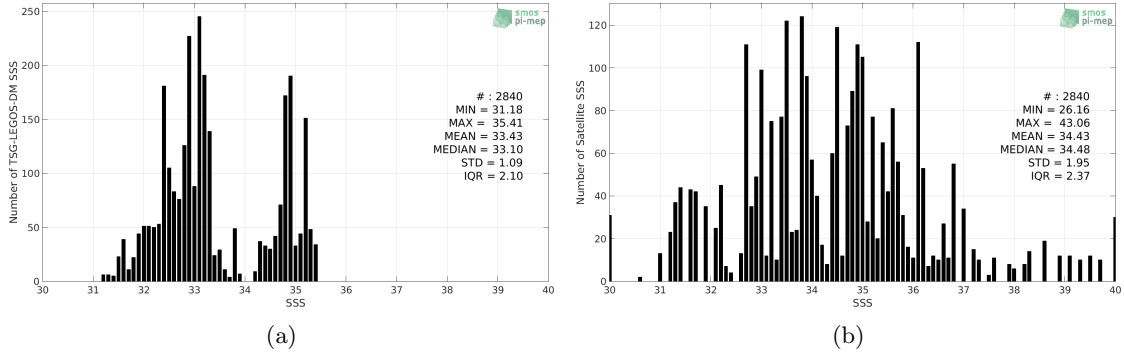
Figure 2: Histograms of SSS from TSG-LEGOS-DM (a) and SMOS L2Q v321 - 0.25 Deg (CATDS-CPDC) (b) considering all match-up pairs per bins of 0.1 over the Arctic Ocean Pi-MEP region and for the full satellite product period.
