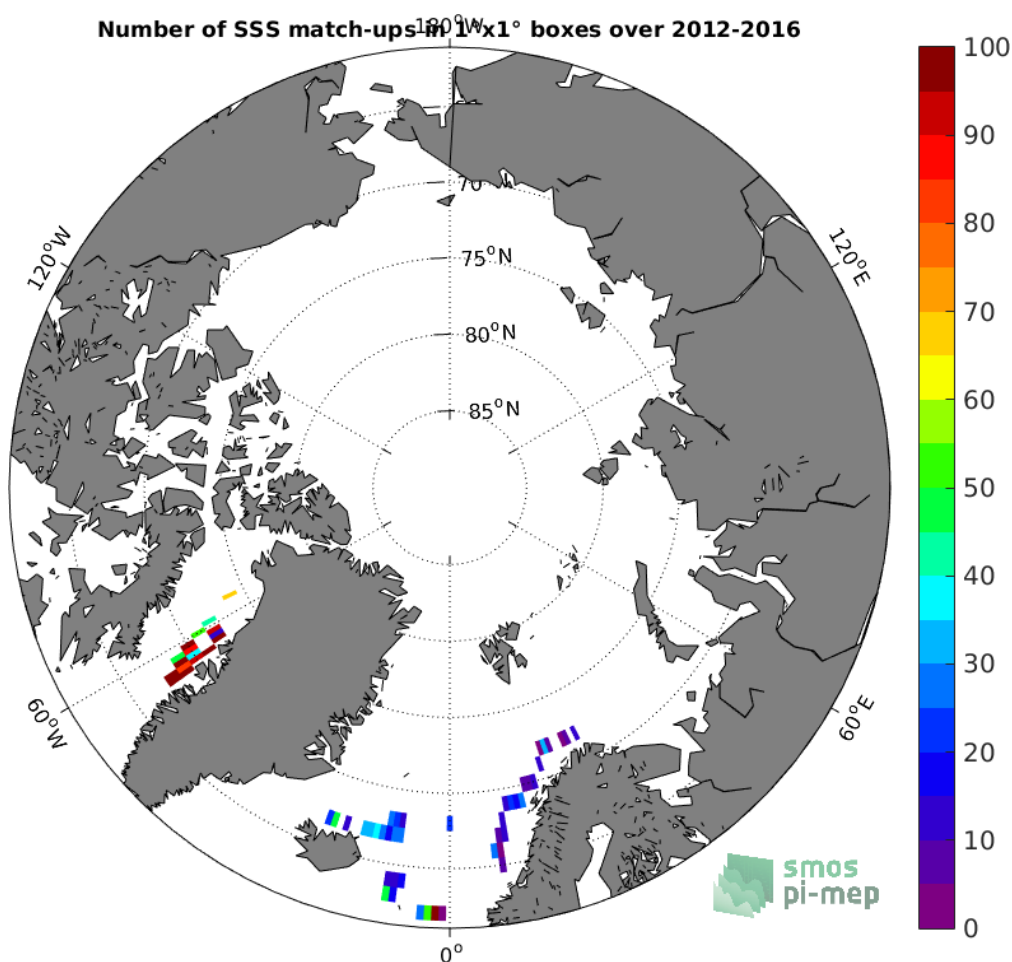
Figure 4: Number of SSS match-ups between TSG-LEGOS-DM SSS and the SMOS L2Q v321 - 0.25 Deg (CATDS-CPDC) SSS product for the Arctic Ocean Pi-MEP region over 1^\circ \times 1^\circ boxes and for the full satellite product period.
