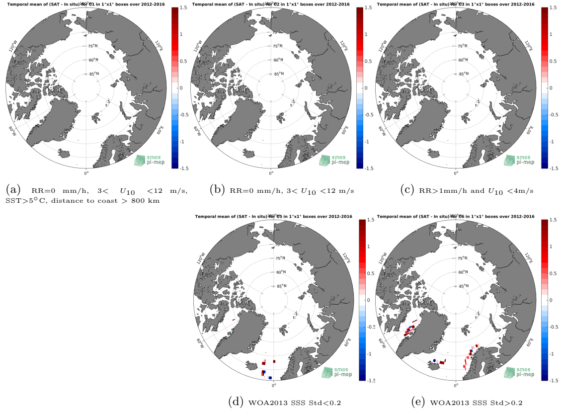
Figure 12: Temporal mean gridded over spatial boxes of size 1^{\circ}\times 1^{\circ} of \Delta\text{SSS} (SMOS L2Q v321 - 0.25 Deg (CATDS-CPDC) - TSG-LEGOS-DM) for 5 different subdatasets corresponding to: RR=0 mm/h, 3 < U_{10} < 12 m/s, SST >5^{\circ}\text{C} , distance to coast > 800 km (a), RR=0 mm/h, 3 < U_{10} < 12 m/s (b), RR >1 mm/h and U_{10} < 4 m/s (c), WOA2013 SSS Std <0.2 (d), WOA2013 SSS Std >0.2 (e).
