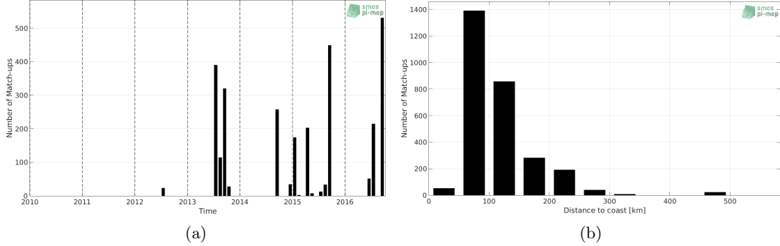
Figure 1: Number of match-ups between TSG-LEGOS-DM and SMOS L2Q v321 - 0.25 Deg (CATDS-CPDC) SSS as a function of time (a) and as function of the distance to coast (b) over the Arctic Ocean Pi-MEP region and for the full satellite product period.
