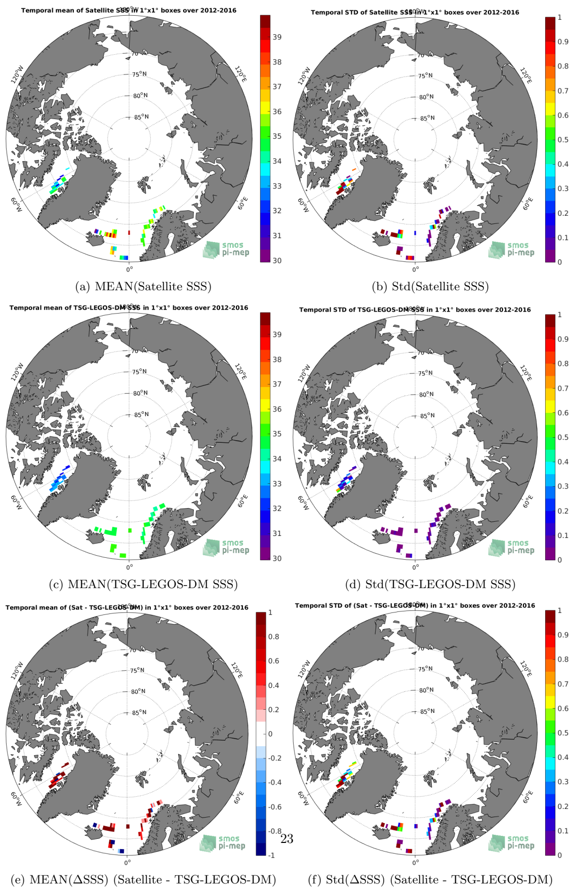
Figure 6: Temporal mean (left) and Std (right) of SSS from SMOS L2Q v321 - 0.25 Deg (CATDS-CPDC) (top), TSG-LEGOS-DM (middle), and of \Delta SSS (Satellite - TSG-LEGOS-DM). Only match-up pairs are used to generate these maps.
