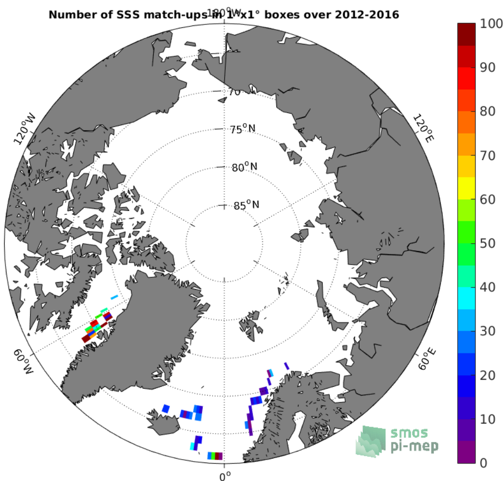
Figure 4: Number of SSS match-ups between TSG-LEGOS-DM SSS and the SMOS-L3-CATDS-CPDC-V321-L2Q SSS product for the Arctic Ocean Pi-MEP region over 1^\circ \times 1^\circ boxes and for the full satellite product period.
