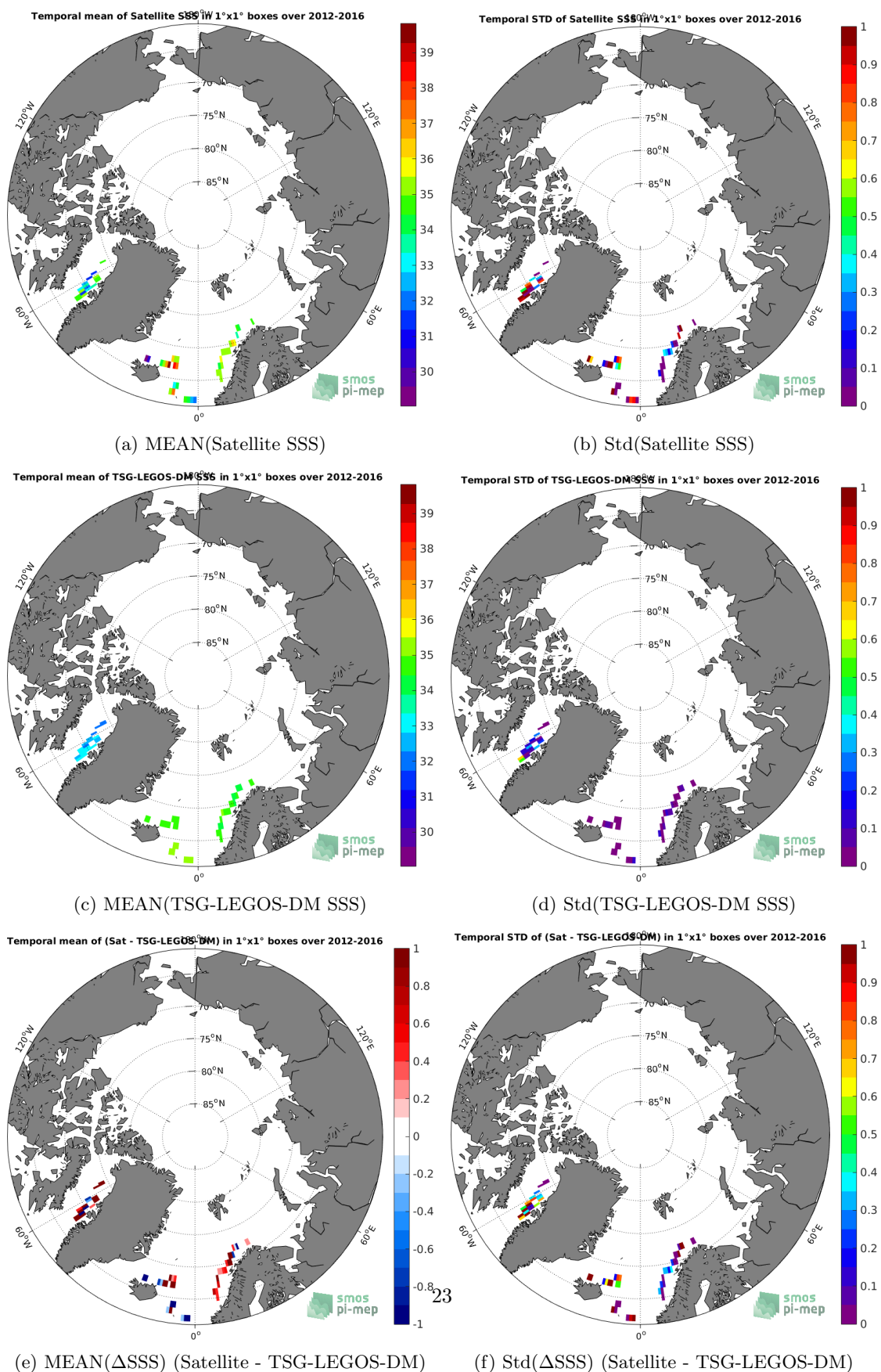
Figure 6: Temporal mean (left) and Std (right) of SSS from SMOS-L3-CATDS-CPDC-V321-L2Q (top), TSG-LEGOS-DM (middle), and of \Delta SSS (Satellite - TSG-LEGOS-DM). Only match-up pairs are used to generate these maps.
