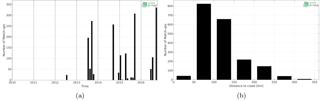
Figure 1: Number of match-ups between TSG-LEGOS-DM and SMOS-L3-CATDS-CPDC-V321-L2Q SSS as a function of time (a) and as function of the distance to coast (b) over the Arctic Ocean Pi-MEP region and for the full satellite product period.
