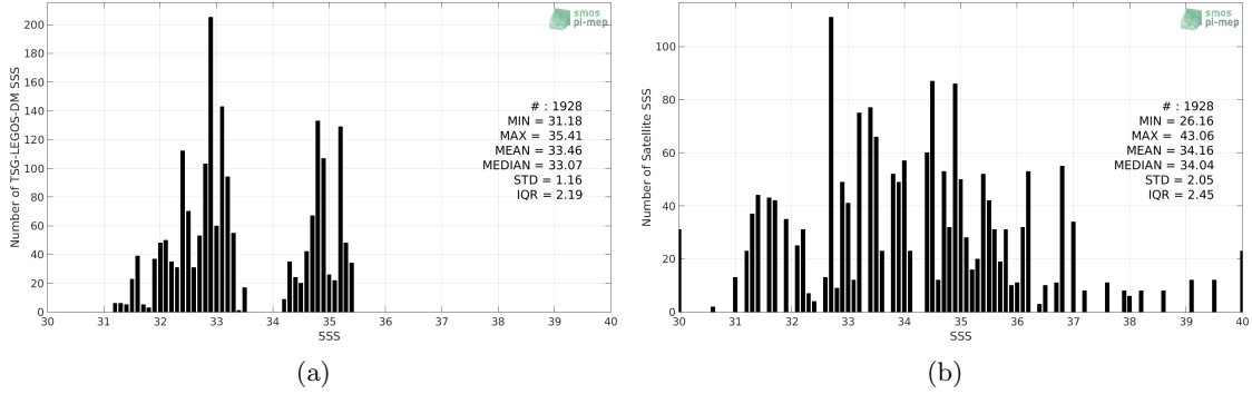
Figure 2: Histograms of SSS from TSG-LEGOS-DM (a) and SMOS-L3-CATDS-CPDC-V321-L2Q (b) considering all match-up pairs per bins of 0.1 over the Arctic Ocean Pi-MEP region and for the full satellite product period.
