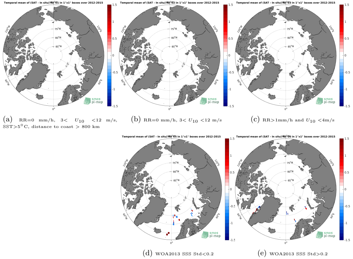
Figure 12: Temporal mean gridded over spatial boxes of size 1^{\circ} \times 1^{\circ} of \Delta\text{SSS} (SMOS SSS L2Q v321 - 0.25 Deg (CATDS-CPDC) - TSG (GOSUD-Sailing-ship)) for 5 different subdatasets corresponding to: RR=0 mm/h, 3 < U_{10} < 12 m/s, SST > 5^{\circ}\text{C} , distance to coast > 800 km (a), RR=0 mm/h, 3 < U_{10} < 12 m/s (b), RR > 1 mm/h and U_{10} < 4 m/s (c), WOA2013 SSS Std < 0.2 (d), WOA2013 SSS Std > 0.2 (e).
