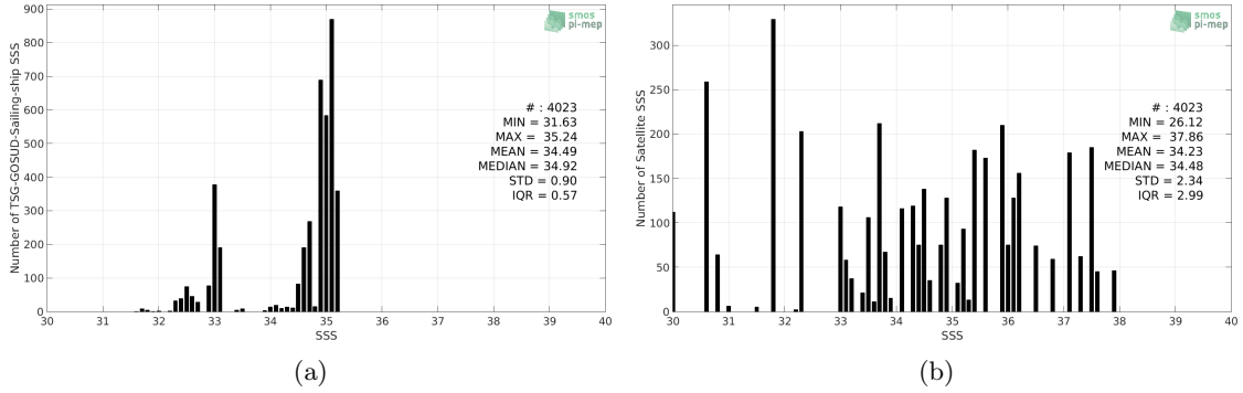
Figure 2: Histograms of SSS from TSG-GOSUD-Sailing-ship (a) and SMOS L2Q v321 - 0.25 Deg (CATDS-CPDC) (b) considering all match-up pairs per bins of 0.1 over the Arctic Ocean Pi-MEP region and for the full satellite product period.
