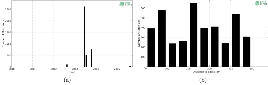
Figure 1: Number of match-ups between TSG-GOSUD-Sailing-ship and SMOS L2Q v321 - 0.25 Deg (CATDS-CPDC) SSS as a function of time (a) and as function of the distance to coast (b) over the Arctic Ocean Pi-MEP region and for the full satellite product period.
