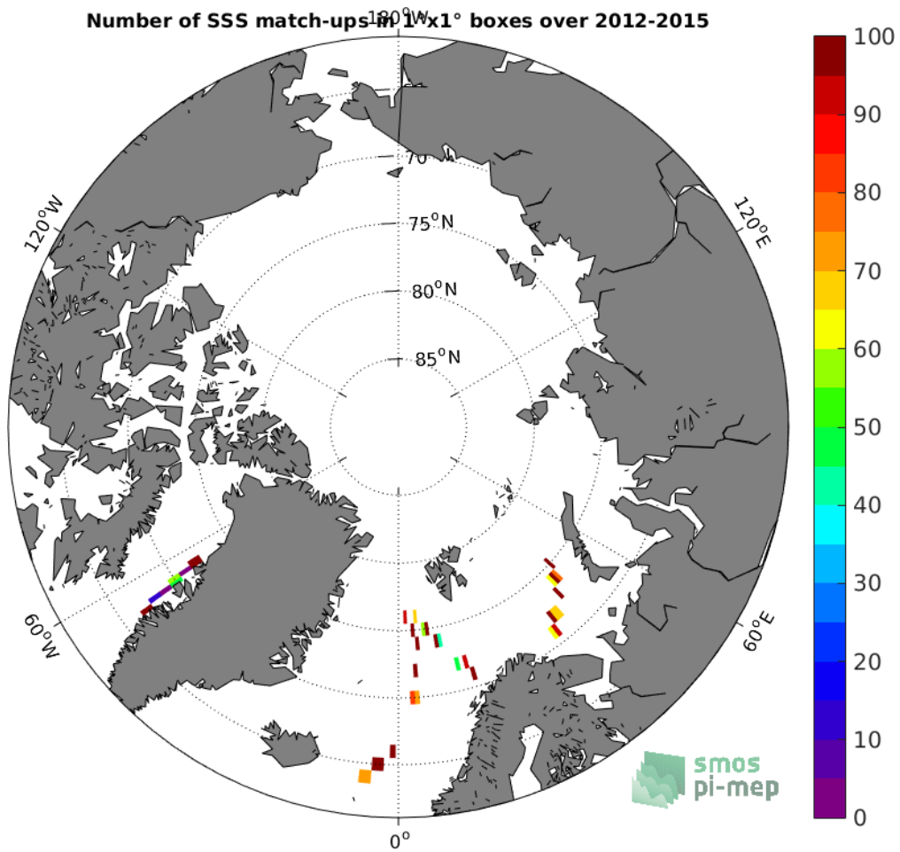
Figure 4: Number of SSS match-ups between TSG-GOSUD-Sailing-ship SSS and the SMOS L2Q v321 - 0.25 Deg (CATDS-CPDC) SSS product for the Arctic Ocean Pi-MEP region over 1^\circ \times 1^\circ boxes and for the full satellite product period.
