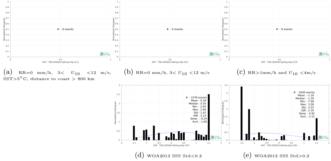
Figure 13: Normalized histogram of \Delta\text{SSS} (SMOS L2Q v321 - 0.25 Deg (CATDS-CPDC) - TSG-GOSUD-Sailing-ship) for 5 different subdatasets corresponding to: RR=0 mm/h, 3 < U_{10} < 12 m/s, SST > 5^{\circ}\text{C} , distance to coast > 800 km (a), RR=0 mm/h, 3 < U_{10} < 12 m/s (b), RR > 1\text{mm/h} and U_{10} < 4\text{m/s} (c), WOA2013 SSS Std < 0.2 (d), WOA2013 SSS Std > 0.2 (e).
