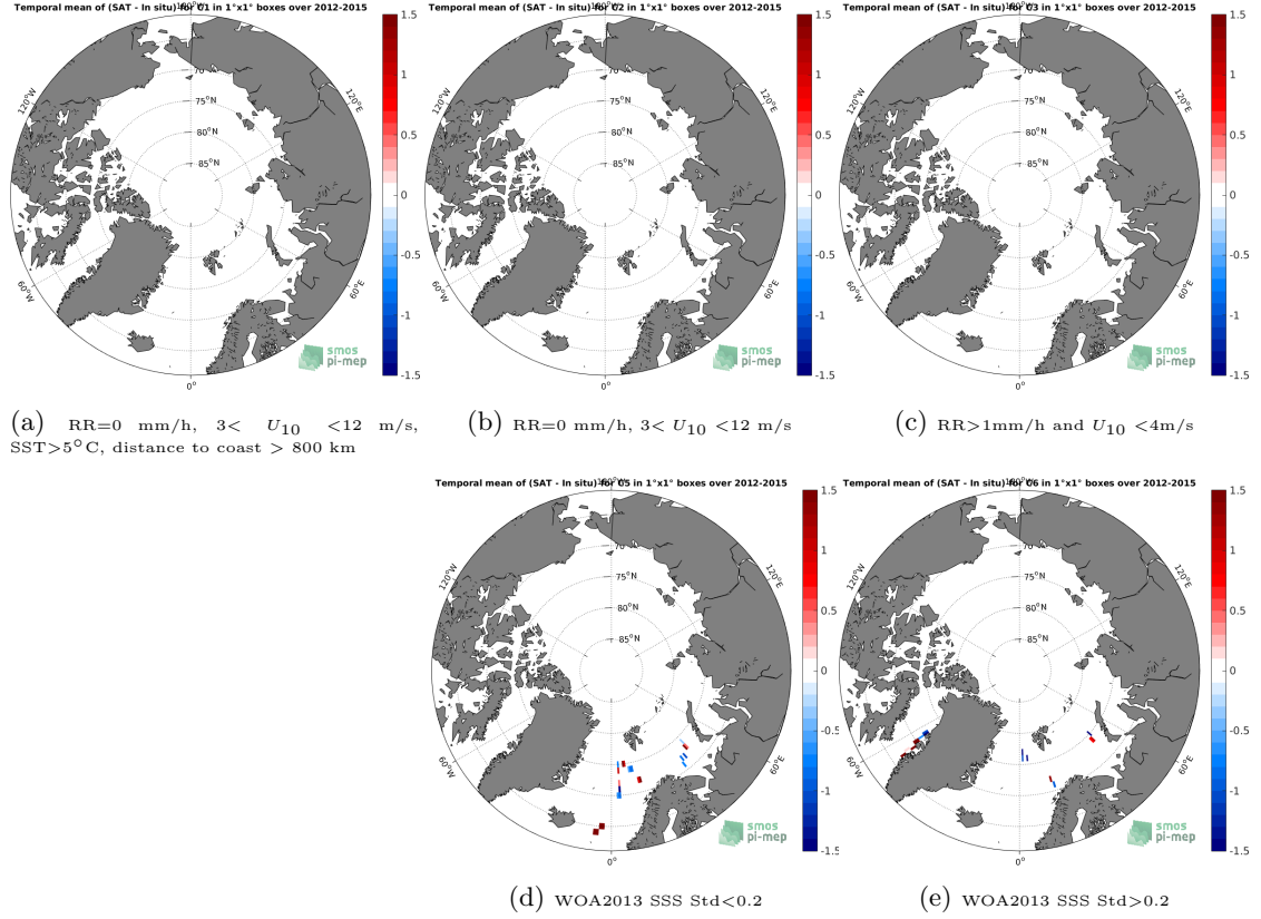
Figure 12: Temporal mean gridded over spatial boxes of size 1^{\circ} \times 1^{\circ} of \Delta\text{SSS} (SMOS L2Q v321 - 0.25 Deg (CATDS-CPDC) - TSG-GOSUD-Sailing-ship) for 5 different subdatasets corresponding to: RR=0 mm/h, 3 < U_{10} < 12 m/s, SST > 5^{\circ}\text{C} , distance to coast > 800 km (a), RR=0 mm/h, 3 < U_{10} < 12 m/s (b), RR > 1\text{mm/h} and U_{10} < 4\text{m/s} (c), WOA2013 SSS Std < 0.2 (d), WOA2013 SSS Std > 0.2 (e).
