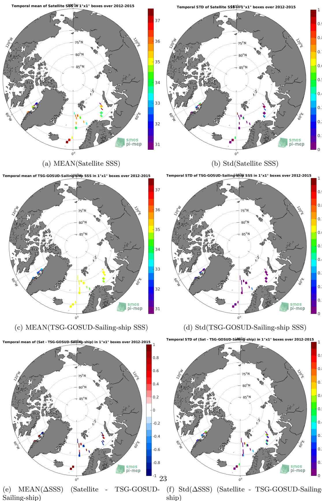
Figure 6: Temporal mean (left) and Std (right) of SSS from SMOS-L3-CATDS-CPDC-V321-L2Q (top), TSG-GOSUD-Sailing-ship (middle), and of \Delta SSS (Satellite - TSG-GOSUD-Sailing-ship). Only match-up pairs are used to generate these maps.
