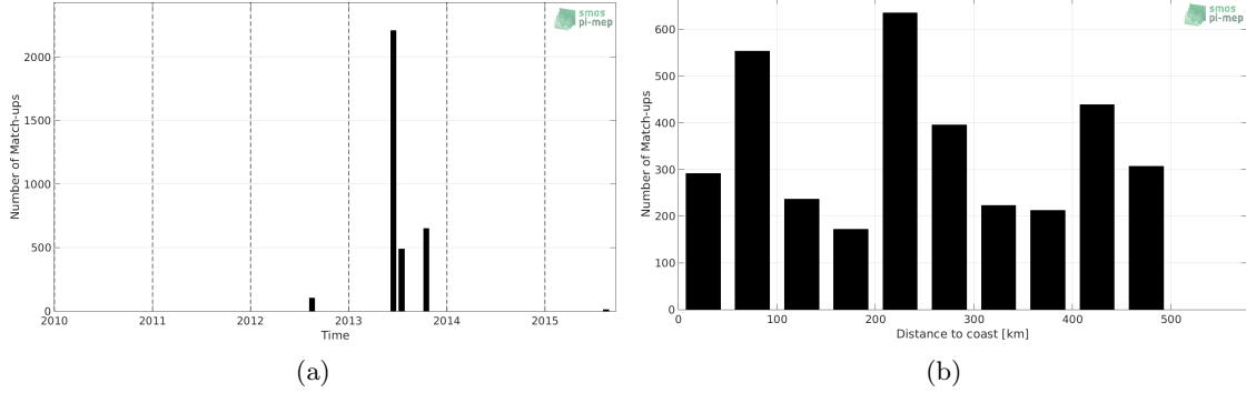
Figure 1: Number of match-ups between TSG-GOSUD-Sailing-ship and SMOS-L3-CATDS-CPDC-V321-L2Q SSS as a function of time (a) and as function of the distance to coast (b) over the Arctic Ocean Pi-MEP region and for the full satellite product period.
