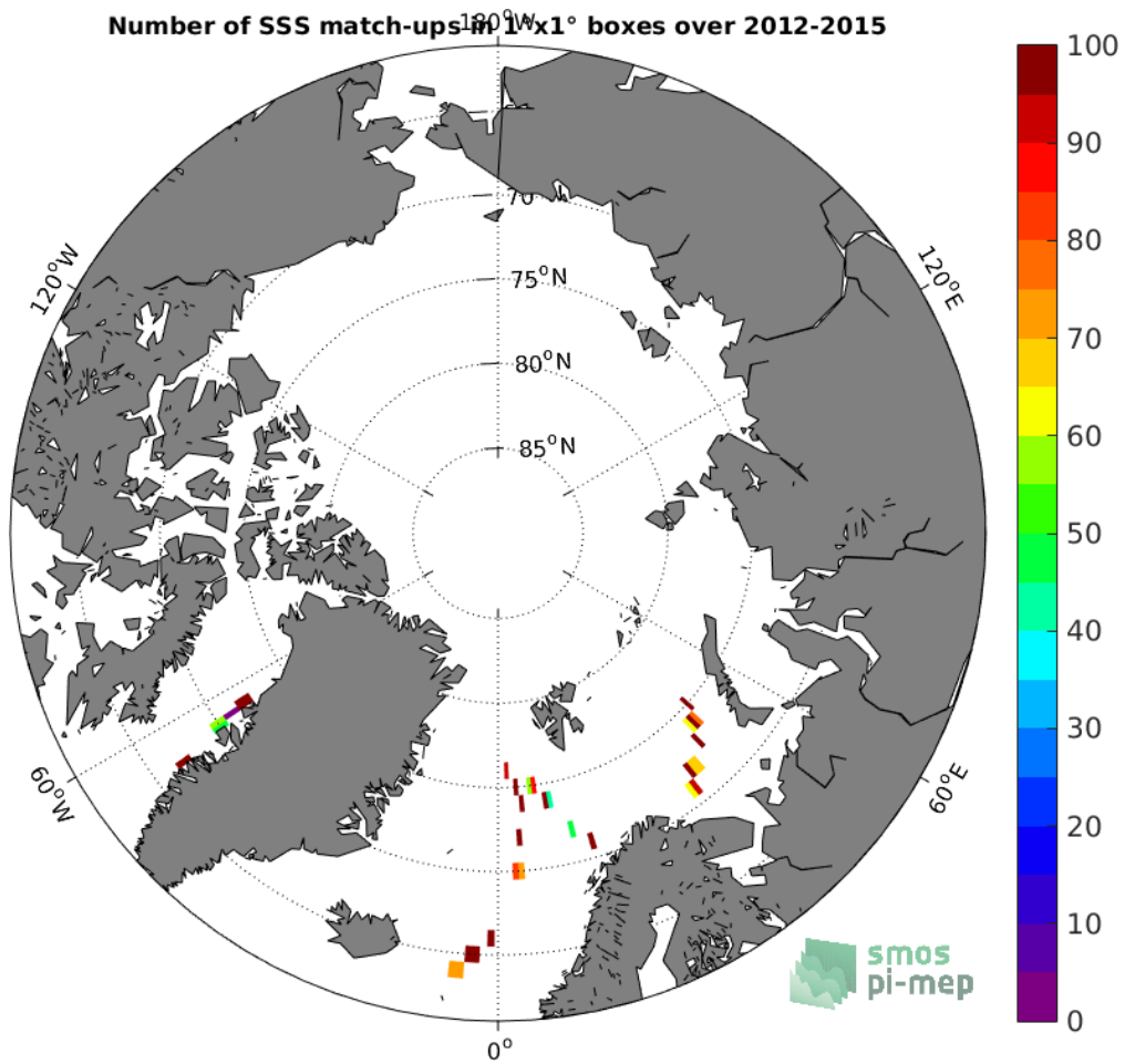
Figure 4: Number of SSS match-ups between TSG-GOSUD-Sailing-ship SSS and the SMOS-L3-CATDS-CPDC-V321-L2Q SSS product for the Arctic Ocean Pi-MEP region over 1^\circ \times 1^\circ boxes and for the full satellite product period.
