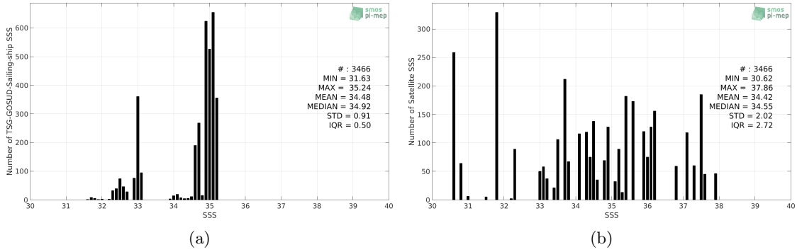
Figure 2: Histograms of SSS from TSG-GOSUD-Sailing-ship (a) and SMOS-L3-CATDS-CPDC-V321-L2Q (b) considering all match-up pairs per bins of 0.1 over the Arctic Ocean Pi-MEP region and for the full satellite product period.
