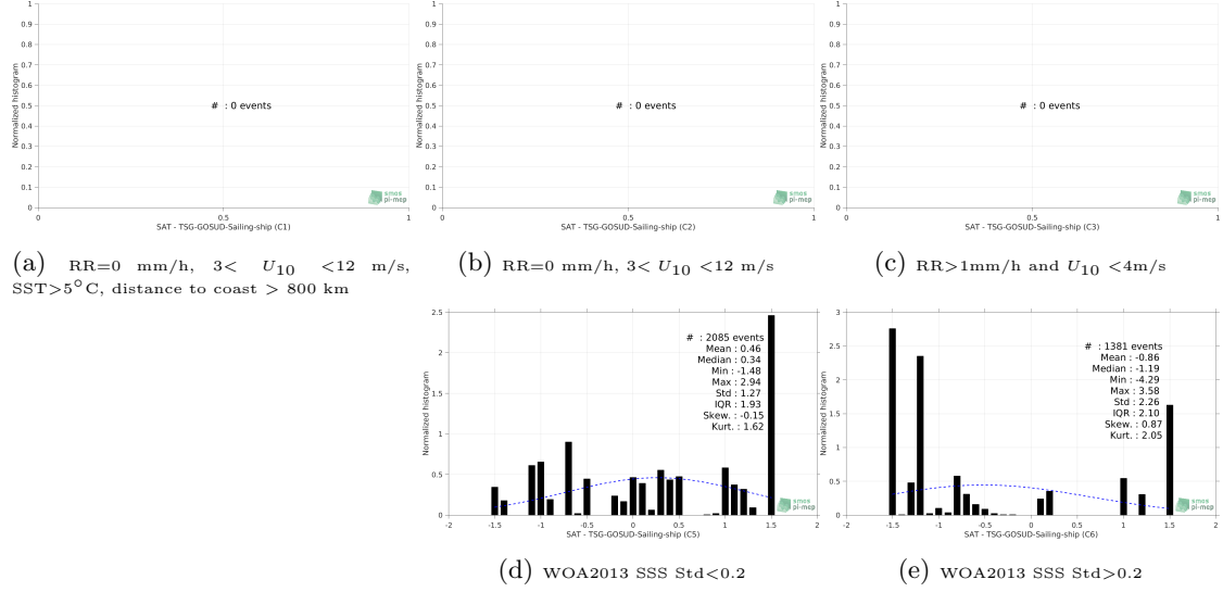
Figure 13: Normalized histogram of \Delta\text{SSS} (SMOS-L3-CATDS-CPDC-V321-L2Q - TSG-GOSUD-Sailing-ship) for 5 different subdatasets corresponding to: RR=0 mm/h, 3 < U_{10} < 12 m/s, SST > 5^{\circ}\text{C} , distance to coast > 800 km (a), RR=0 mm/h, 3 < U_{10} < 12 m/s (b), RR > 1 mm/h and U_{10} < 4 m/s (c), WOA2013 SSS Std < 0.2 (d), WOA2013 SSS Std > 0.2 (e).
