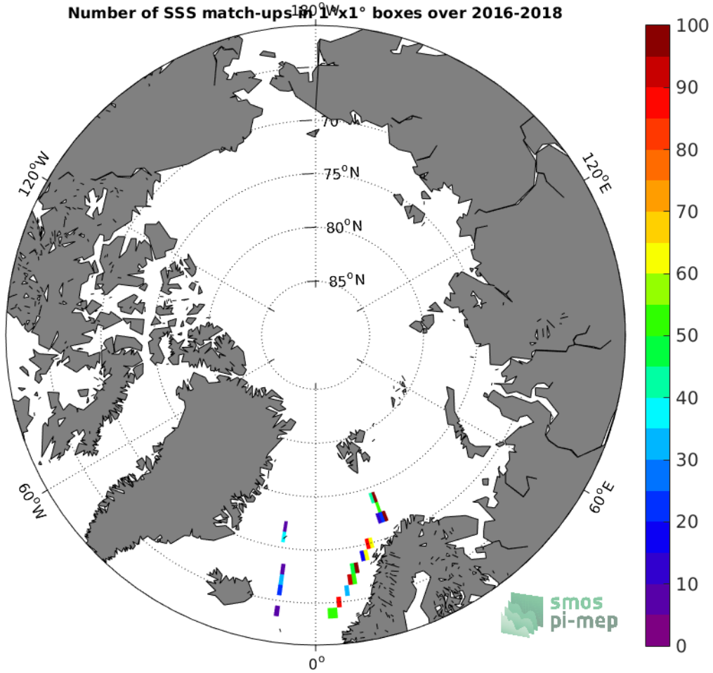
Figure 4: Number of SSS match-ups between TSG (GOSUD-Research-vessel) SSS and the SMOS SSS L2Q v321 - 0.25 Deg (CATDS-CPDC) SSS product for the Arctic Ocean Pi-MEP region over 1^\circ \times 1^\circ boxes and for the full satellite product period.
