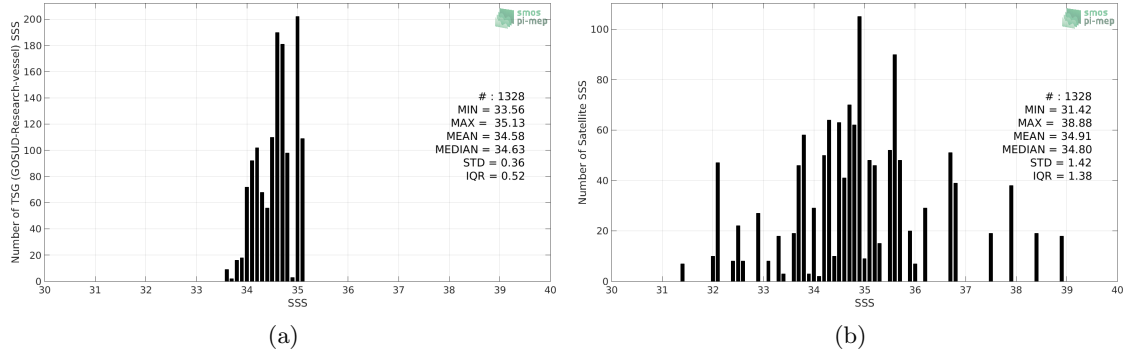
Figure 2: Histograms of SSS from TSG (GOSUD-Research-vessel) (a) and SMOS SSS L2Q v321 - 0.25 Deg (CATDS-CPDC) (b) considering all match-up pairs per bins of 0.1 over the Arctic Ocean Pi-MEP region and for the full satellite product period.
