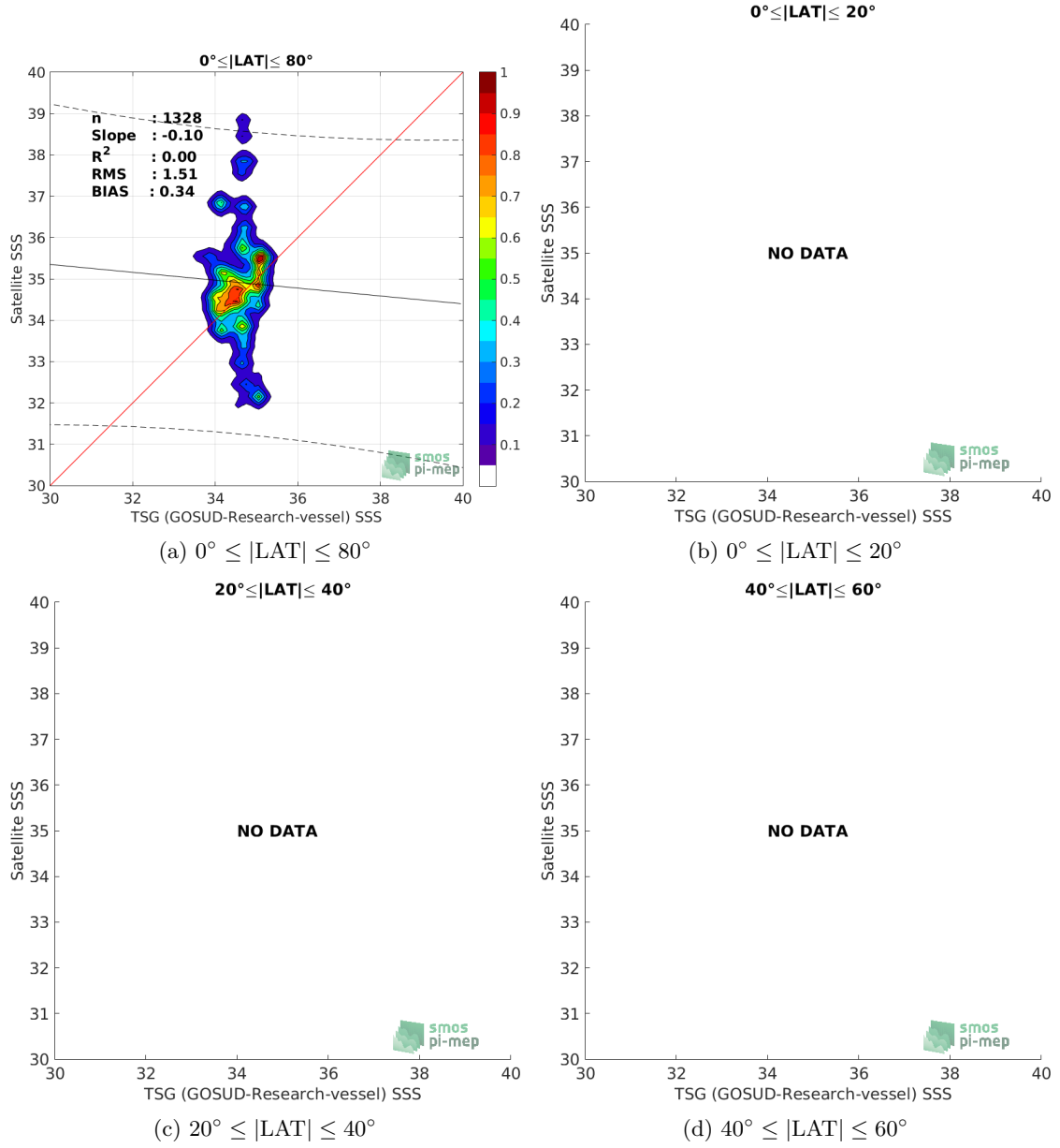
Figure 9: Contour maps of the concentration of SMOS SSS L2Q v321 - 0.25 Deg (CATDS-CPDC) SSS (y-axis) versus TSG (GOSUD-Research-vessel) SSS (x-axis) at match-up pairs for different latitude bands. For each plot, the red line shows x=y . The black thin and dashed lines indicate a linear fit through the data cloud and the \pm 95\% confidence levels, respectively. The number match-up pairs n , the slope and R^2 coefficient of the linear fit, the root mean square (RMS) and the mean bias between satellite and in situ data are indicated for each latitude band in each plots.
