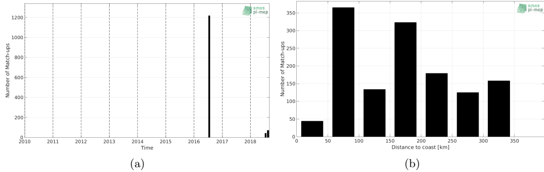
Figure 1: Number of match-ups between TSG (GOSUD-Research-vessel) and SMOS SSS L2Q v321 - 0.25 Deg (CATDS-CPDC) SSS as a function of time (a) and as function of the distance to coast (b) over the Arctic Ocean Pi-MEP region and for the full satellite product period.
