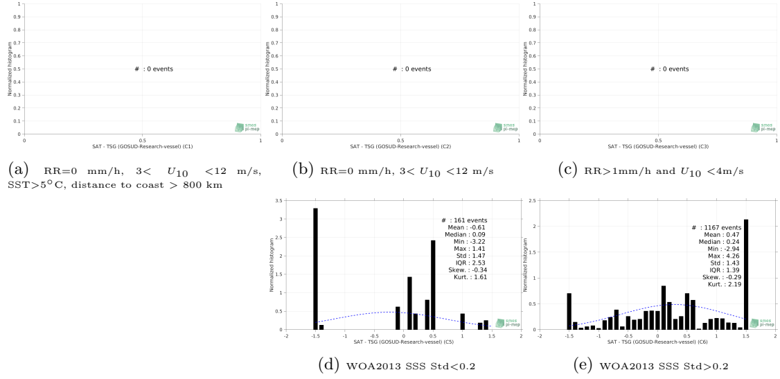
Figure 13: Normalized histogram of \Delta\text{SSS} (SMOS SSS L2Q v321 - 0.25 Deg (CATDS-CPDC) - TSG (GOSUD-Research-vessel)) for 5 different subdatasets corresponding to: RR=0 mm/h, 3 < U_{10} < 12 m/s, SST > 5^\circ\text{C} , distance to coast > 800 km (a), RR=0 mm/h, 3 < U_{10} < 12 m/s (b), RR > 1\text{mm/h} and U_{10} < 4\text{m/s} (c), WOA2013 SSS Std<0.2 (d), WOA2013 SSS Std>0.2 (e).
