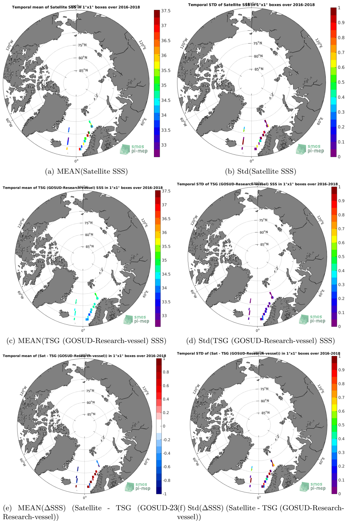
Figure 6: Temporal mean (left) and Std (right) of SSS from SMOS SSS L2Q v321 - 0.25 Deg (CATDS-CPDC) (top), TSG (GOSUD-Research-vessel) (middle), and of \Delta SSS (Satellite - TSG (GOSUD-Research-vessel)). Only match-up pairs are used to generate these maps.
