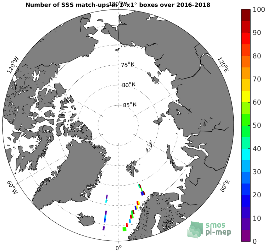
Figure 4: Number of SSS match-ups between TSG (GOSUD-Research-vessel) SSS and the SMOS SSS L2Q v321 - 0.25 Deg (CATDS-CPDC) SSS product for the Arctic Ocean Pi-MEP region over 1°x1° boxes and for the full satellite product period.
