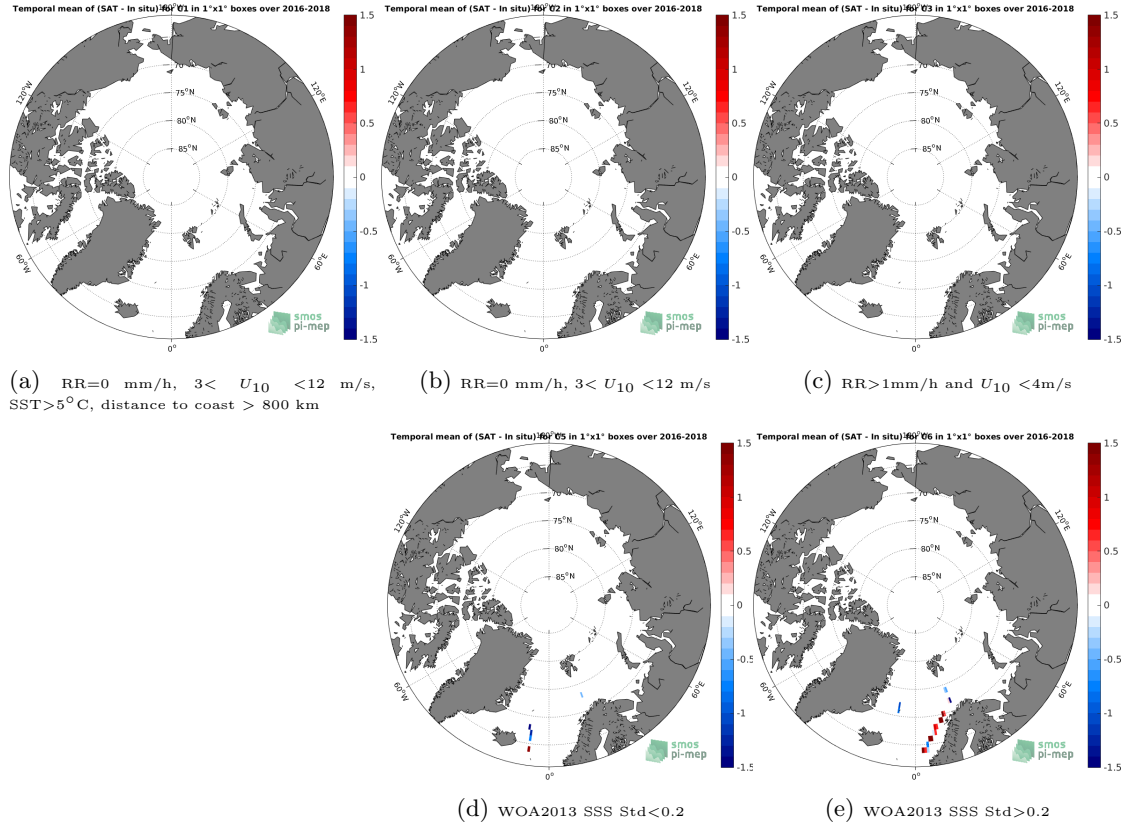
Figure 12: Temporal mean gridded over spatial boxes of size 1°x1° of \Delta SSS (SMOS SSS L2Q v321 - 0.25 Deg (CATDS-CPDC) - TSG (GOSUD-Research-vessel)) for 5 different subdatasets corresponding to: RR=0 mm/h, 3 < U_{10} < 12 m/s, SST>5°C, distance to coast > 800 km (a), RR=0 mm/h, 3 < U_{10} < 12 m/s (b), RR>1mm/h and U_{10} < 4 m/s (c), WOA2013 SSS Std<0.2 (d), WOA2013 SSS Std>0.2 (e).
