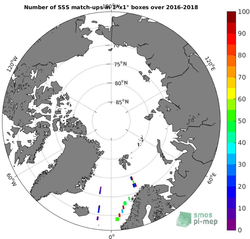
Figure 4: Number of SSS match-ups between TSG-GOSUD-Research-vessel SSS and the SMOS-L3-CATDS-CPDC-V321-L2Q SSS product for the Arctic Ocean Pi-MEP region over 1^\circ \times 1^\circ boxes and for the full satellite product period.
