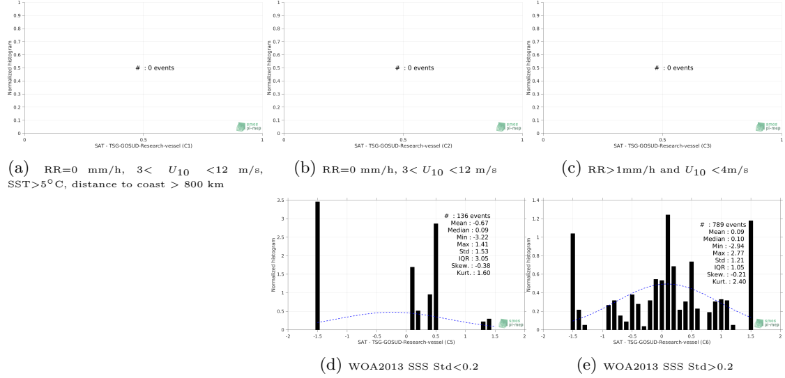
Figure 13: Normalized histogram of \Delta\text{SSS} (SMOS-L3-CATDS-CPDC-V321-L2Q - TSG-GOSUD-Research-vessel) for 5 different subdatasets corresponding to: RR=0 mm/h, 3 < U_{10} < 12 m/s, SST > 5^\circ\text{C} , distance to coast > 800 km (a), RR=0 mm/h, 3 < U_{10} < 12 m/s (b), RR > 1 mm/h and U_{10} < 4 m/s (c), WOA2013 SSS Std < 0.2 (d), WOA2013 SSS Std > 0.2 (e).
