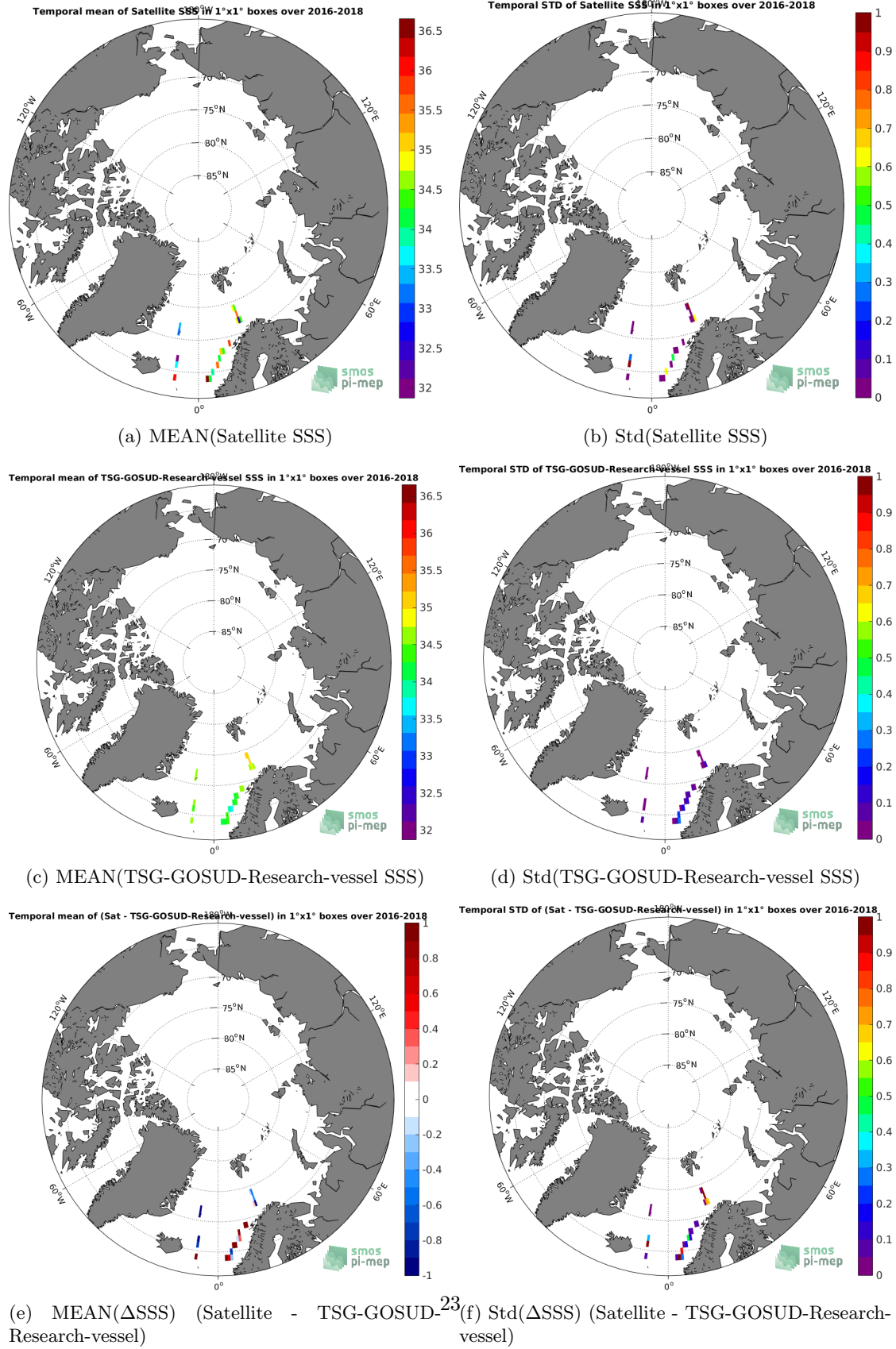
Figure 6: Temporal mean (left) and Std (right) of SSS from SMOS-L3-CATDS-CPDC-V321-L2Q (top), TSG-GOSUD-Research-vessel (middle), and of \Delta SSS (Satellite - TSG-GOSUD-Research-vessel). Only match-up pairs are used to generate these maps.
