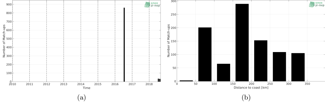
Figure 1: Number of match-ups between TSG-GOSUD-Research-vessel and SMOS-L3-CATDS-CPDC-V321-L2Q SSS as a function of time (a) and as function of the distance to coast (b) over the Arctic Ocean Pi-MEP region and for the full satellite product period.
