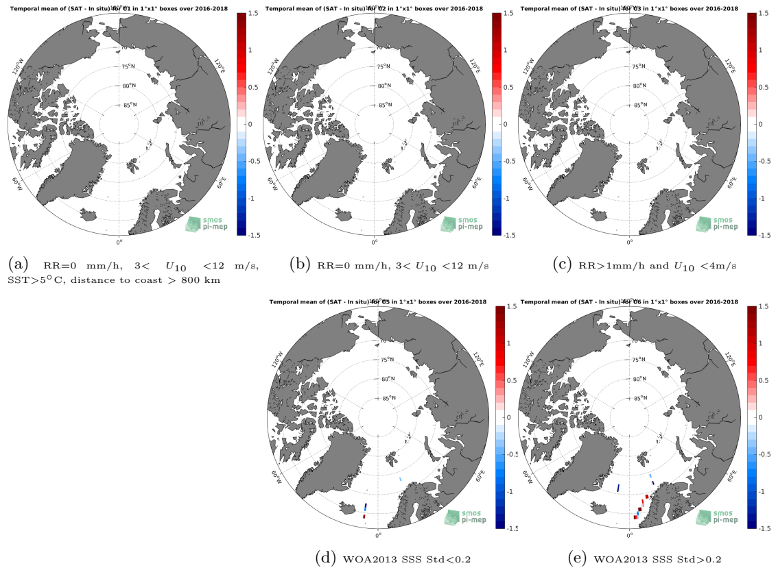
Figure 12: Temporal mean gridded over spatial boxes of size 1^\circ \times 1^\circ of \Delta SSS (SMOS-L3-CATDS-CPDC-V321-L2Q - TSG-GOSUD-Research-vessel) for 5 different subdatasets corresponding to: RR=0 mm/h, 3 < U_{10} < 12 m/s, SST > 5^\circ\text{C} , distance to coast > 800 km (a), RR=0 mm/h, 3 < U_{10} < 12 m/s (b), RR > 1 mm/h and U_{10} < 4 m/s (c), WOA2013 SSS Std < 0.2 (d), WOA2013 SSS Std > 0.2 (e).
