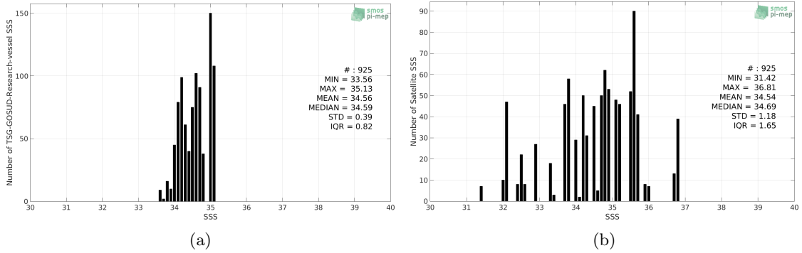
Figure 2: Histograms of SSS from TSG-GOSUD-Research-vessel (a) and SMOS-L3-CATDS-CPDC-V321-L2Q (b) considering all match-up pairs per bins of 0.1 over the Arctic Ocean Pi-MEP region and for the full satellite product period.
