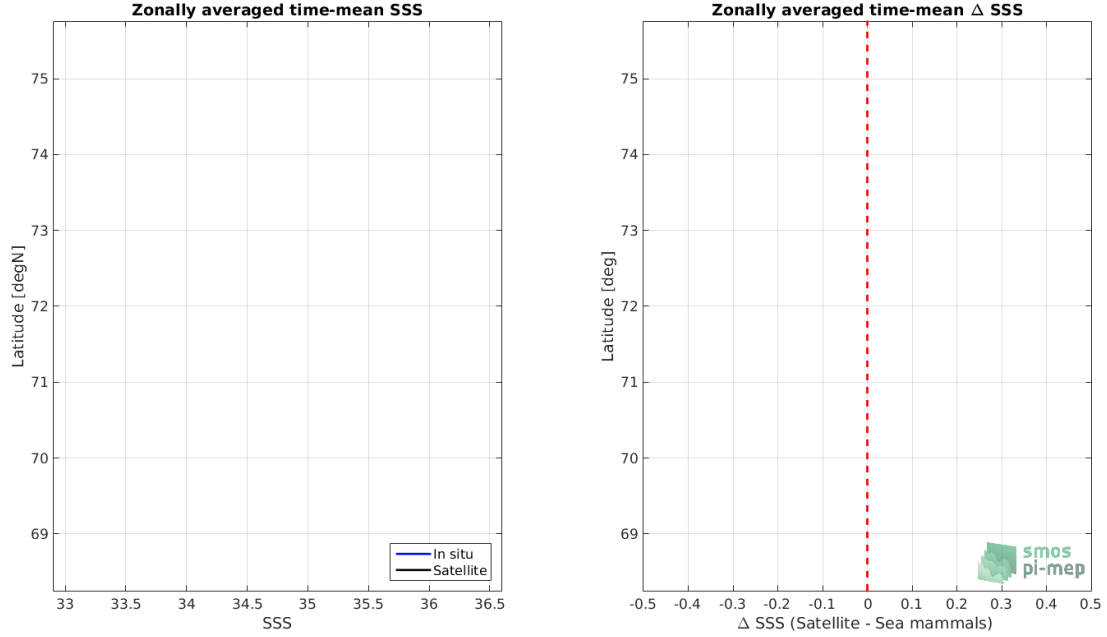
Figure 8: Left panel: Zonal mean SSS from SMOS SSS L2Q v321 - 0.25 Deg (CATDS-CPDC) satellite product (black) and from Marine mammals (blue). Right panel: Zonal mean of \Delta SSS (Satellite - Marine mammals) for all the collected Pi-MEP match-up pairs estimated over the full satellite product period.
