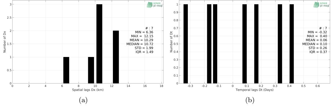
Figure 5: Histograms of the spatial (a) and temporal (b) lags between the location/time of the Marine mammals measurement and the date of the corresponding SMOS SSS L2Q v321 - 0.25 Deg (CATDS-CPDC) SSS pixel.
