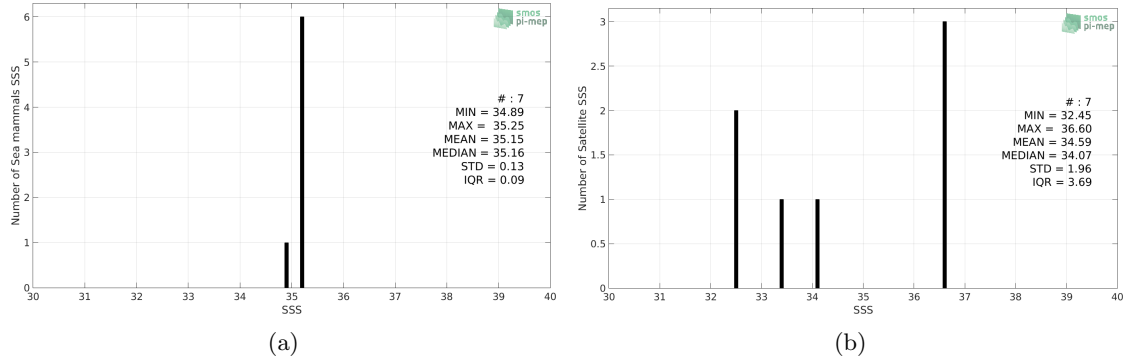
Figure 2: Histograms of SSS from Marine mammals (a) and SMOS SSS L2Q v321 - 0.25 Deg (CATDS-CPDC) (b) considering all match-up pairs per bins of 0.1 over the Arctic Ocean Pi-MEP region and for the full satellite product period.
