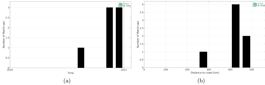
Figure 1: Number of match-ups between Marine mammals and SMOS SSS L2Q v321 - 0.25 Deg (CATDS-CPDC) SSS as a function of time (a) and as function of the distance to coast (b) over the Arctic Ocean Pi-MEP region and for the full satellite product period.
