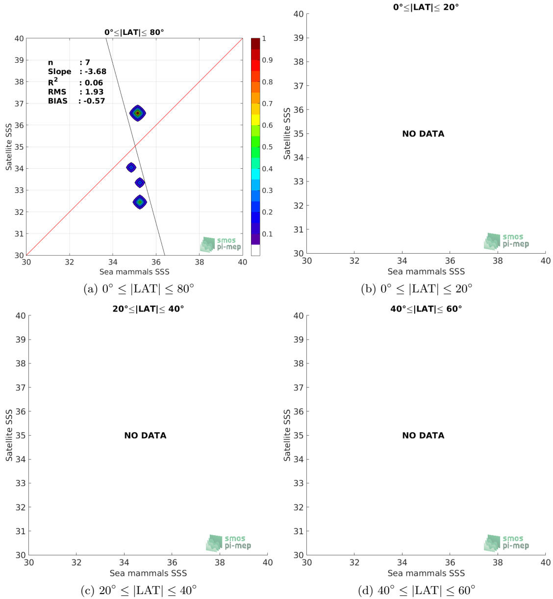
Figure 9: Contour maps of the concentration of SMOS SSS L2Q v321 - 0.25 Deg (CATDS-CPDC) SSS (y-axis) versus Marine mammals SSS (x-axis) at match-up pairs for different latitude bands. For each plot, the red line shows x=y . The black thin and dashed lines indicate a linear fit through the data cloud and the \pm 95\% confidence levels, respectively. The number match-up pairs n , the slope and R^2 coefficient of the linear fit, the root mean square (RMS) and the mean bias between satellite and in situ data are indicated for each latitude band in each plots.
