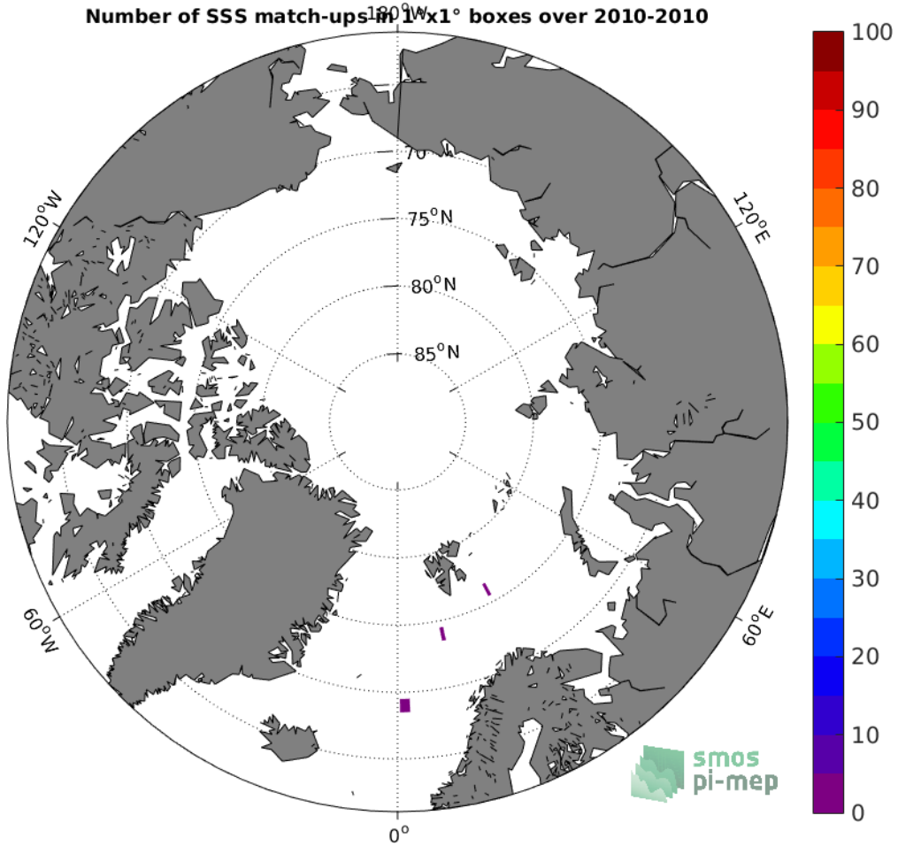
Figure 4: Number of SSS match-ups between Marine mammals SSS and the SMOS SSS L2Q v321 - 0.25 Deg (CATDS-CPDC) SSS product for the Arctic Ocean Pi-MEP region over 1^\circ \times 1^\circ boxes and for the full satellite product period.
