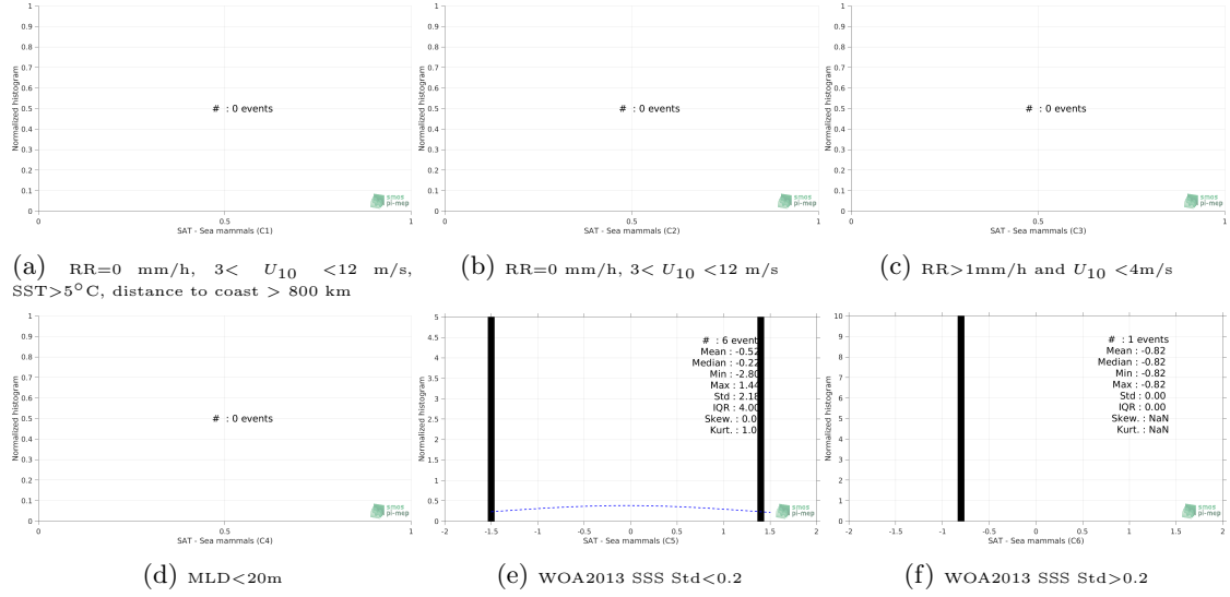
Figure 13: Normalized histogram of \Delta\text{SSS} (SMOS SSS L2Q v321 - 0.25 Deg (CATDS-CPDC) - Marine mammals) for 6 different subdatasets corresponding to: RR=0 mm/h, 3 < U_{10} < 12 m/s, SST > 5^\circ\text{C} , distance to coast > 800 km (a), RR=0 mm/h, 3 < U_{10} < 12 m/s (b), RR > 1 mm/h and U_{10} < 4 m/s (c), MLD < 20 m (d), WOA2013 SSS Std < 0.2 (e), WOA2013 SSS Std > 0.2 (f).
