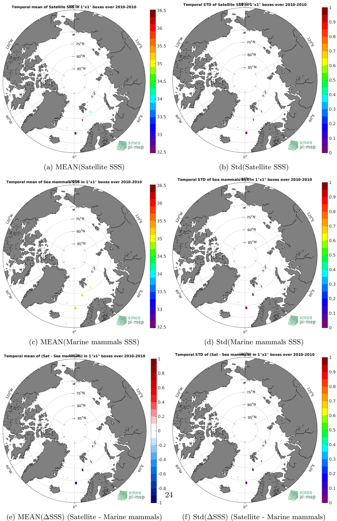
Figure 6: Temporal mean (left) and Std (right) of SSS from SMOS SSS L2Q v321 - 0.25 Deg (CATDS-CPDC) (top), Marine mammals (middle), and of \Delta SSS (Satellite - Marine mammals). Only match-up pairs are used to generate these maps.
