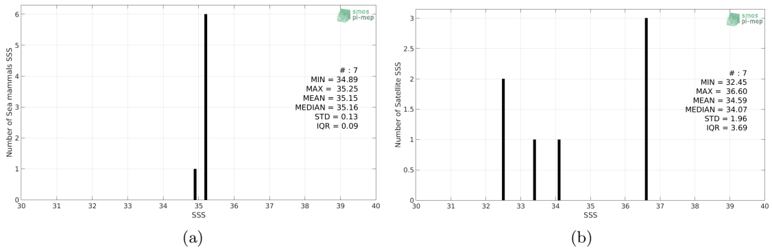
Figure 2: Histograms of SSS from Sea mammals (a) and SMOS SSS L2Q v321 - 0.25 Deg (CATDS-CPDC) (b) considering all match-up pairs per bins of 0.1 over the Arctic Ocean Pi-MEP region and for the full satellite product period.
