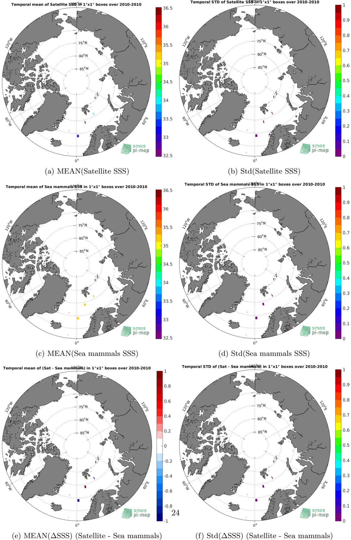
Figure 6: Temporal mean (left) and Std (right) of SSS from SMOS SSS L2Q v321 - 0.25 Deg (CATDS-CPDC) (top), Sea mammals (middle), and of \Delta SSS (Satellite - Sea mammals). Only match-up pairs are used to generate these maps.
