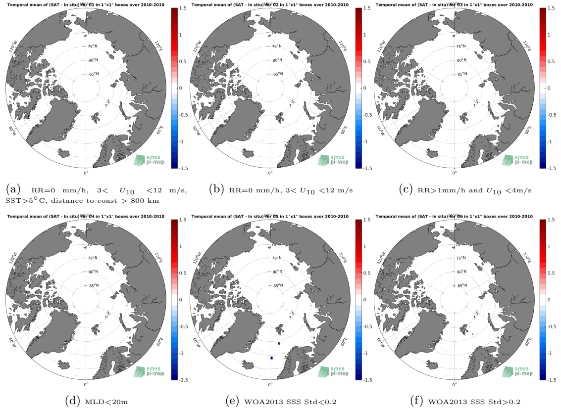
Figure 12: Temporal mean gridded over spatial boxes of size 1^{\circ}\times 1^{\circ} of \Delta\text{SSS} (SMOS SSS L2Q v321 - 0.25 Deg (CATDS-CPDC) - Sea mammals) for 6 different subdatasets corresponding to: \text{RR}=0 mm/h, 3 < U_{10} < 12 m/s, \text{SST}>5^{\circ}\text{C} , distance to coast > 800 km (a), \text{RR}=0 mm/h, 3 < U_{10} < 12 m/s (b), \text{RR}>1\text{mm/h} and U_{10} < 4\text{m/s} (c), \text{MLD}<20\text{m} (d), \text{WOA2013 SSS Std}<0.2 (e), \text{WOA2013 SSS Std}>0.2 (f).
