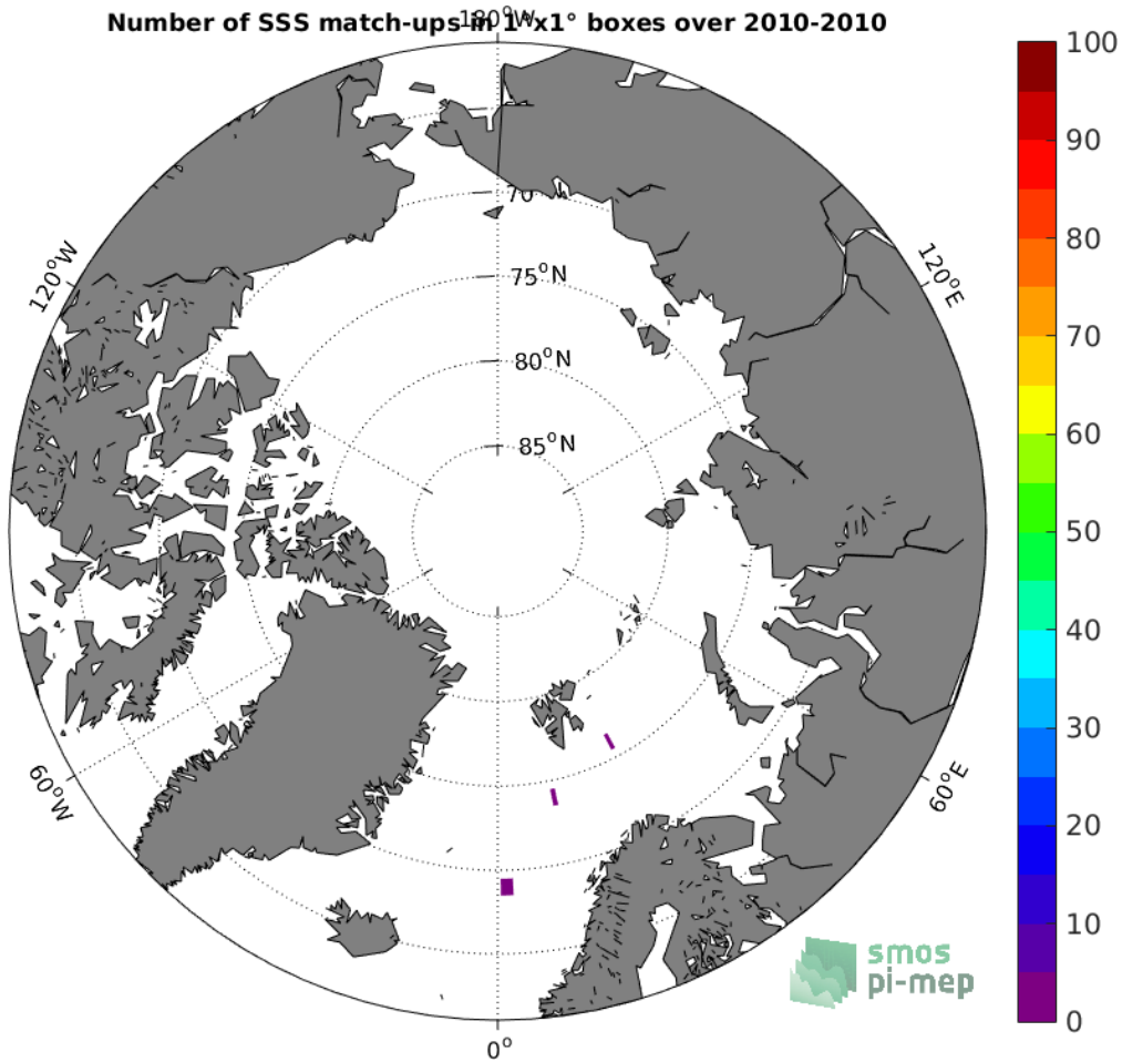
Figure 4: Number of SSS match-ups between Sea mammals SSS and the SMOS SSS L2Q v321 - 0.25 Deg (CATDS-CPDC) SSS product for the Arctic Ocean Pi-MEP region over 1°x1° boxes and for the full satellite product period.
