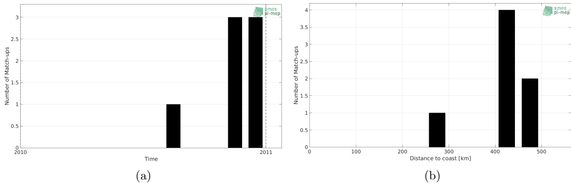
Figure 1: Number of match-ups between Sea mammals and SMOS SSS L2Q v321 - 0.25 Deg (CATDS-CPDC) SSS as a function of time (a) and as function of the distance to coast (b) over the Arctic Ocean Pi-MEP region and for the full satellite product period.
