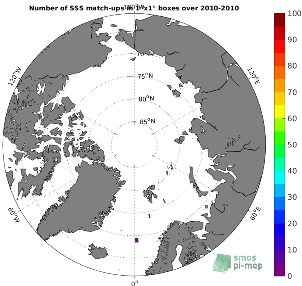
Figure 4: Number of SSS match-ups between Sea mammals SSS and the SMOS-L3-CATDS-CPDC-V321-L2Q SSS product for the Arctic Ocean Pi-MEP region over 1^\circ \times 1^\circ boxes and for the full satellite product period.
