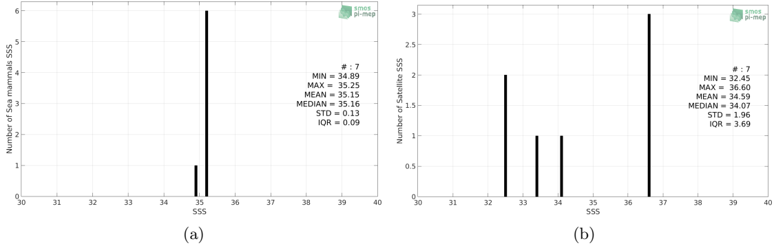
Figure 2: Histograms of SSS from Sea mammals (a) and SMOS-L3-CATDS-CPDC-V321-L2Q (b) considering all match-up pairs per bins of 0.1 over the Arctic Ocean Pi-MEP region and for the full satellite product period.
