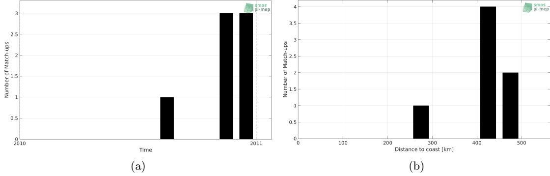
Figure 1: Number of match-ups between Sea mammals and SMOS-L3-CATDS-CPDC-V321-L2Q SSS as a function of time (a) and as function of the distance to coast (b) over the Arctic Ocean Pi-MEP region and for the full satellite product period.
