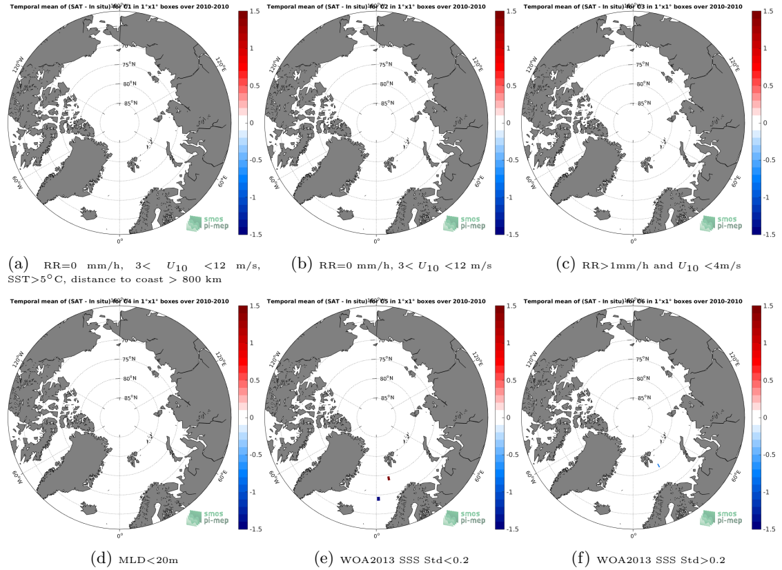
Figure 12: Temporal mean gridded over spatial boxes of size 1^\circ \times 1^\circ of \Delta SSS (SMOS-L3-CATDS-CPDC-V321-L2Q - Sea mammals) for 6 different subdatasets corresponding to: RR=0 mm/h, 3 < U_{10} < 12 m/s, SST > 5^\circ C , distance to coast > 800 km (a), RR=0 mm/h, 3 < U_{10} < 12 m/s (b), RR > 1 mm/h and U_{10} < 4 m/s (c), MLD < 20 m (d), WOA2013 SSS Std < 0.2 (e), WOA2013 SSS Std > 0.2 (f).
