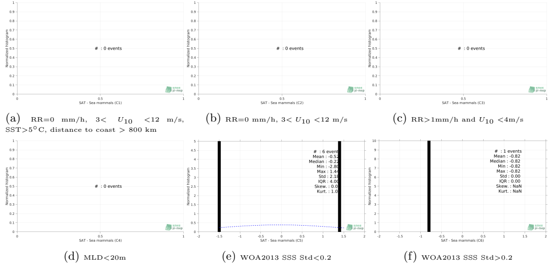
Figure 13: Normalized histogram of \Delta SSS (SMOS-L3-CATDS-CPDC-V321-L2Q - Sea mammals) for 6 different subdatasets corresponding to: RR=0 mm/h, 3 < U_{10} < 12 m/s, SST > 5^\circ\text{C} , distance to coast > 800 km (a), RR=0 mm/h, 3 < U_{10} < 12 m/s (b), RR > 1 mm/h and U_{10} < 4 m/s (c), MLD < 20 m (d), WOA2013 SSS Std < 0.2 (e), WOA2013 SSS Std > 0.2 (f).
