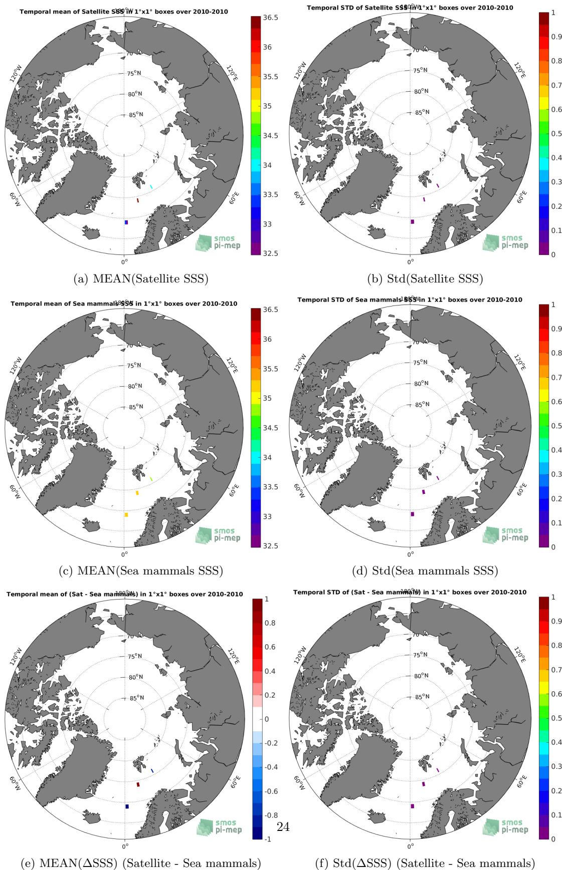
Figure 6: Temporal mean (left) and Std (right) of SSS from SMOS-L3-CATDS-CPDC-V321-L2Q (top), Sea mammals (middle), and of \Delta SSS (Satellite - Sea mammals). Only match-up pairs are used to generate these maps.
