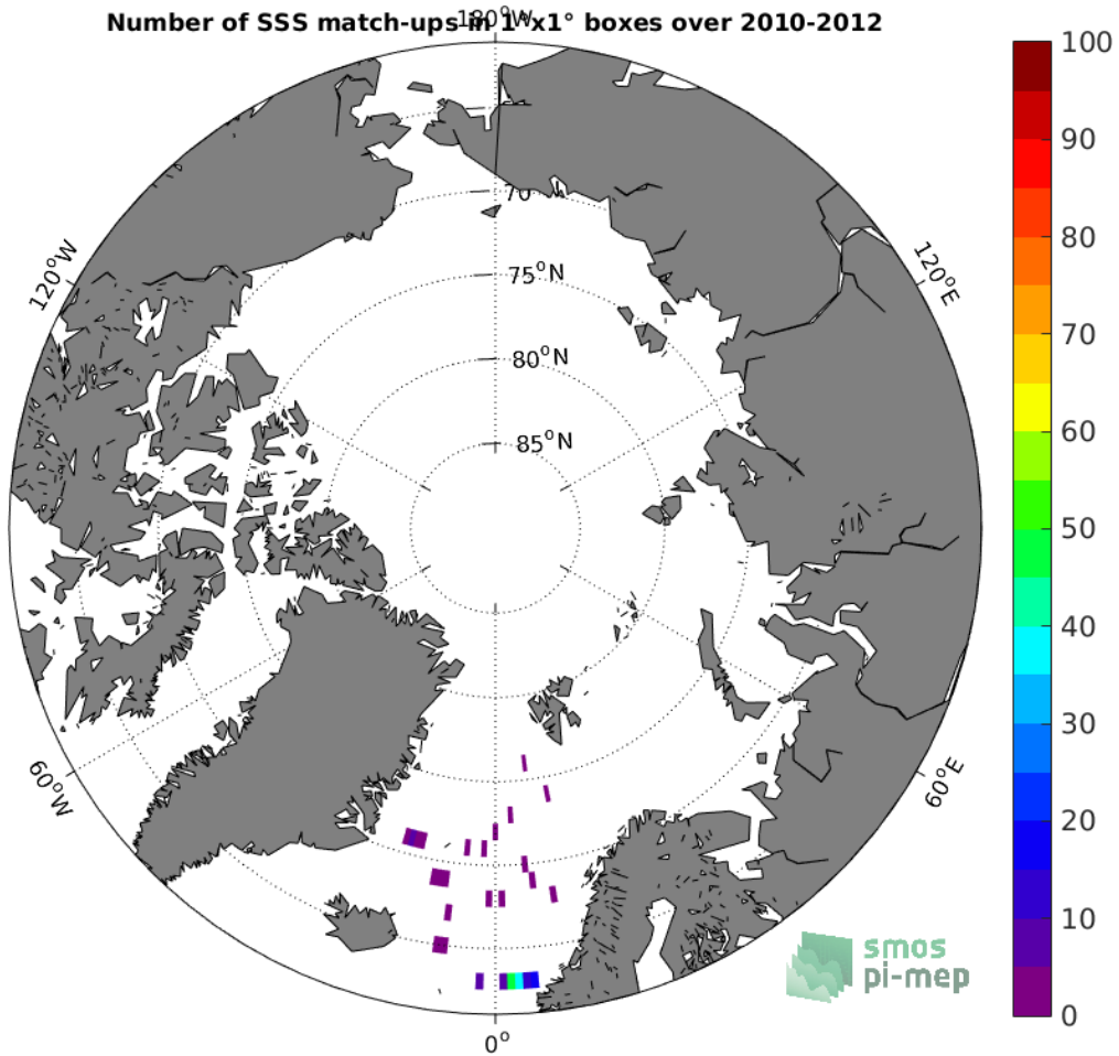
Figure 3: Number of SSS match-ups between Surface drifters SSS and the SMOS SSS L2Q v321 - 0.25 Deg (CATDS-CPDC) SSS product for the Arctic Ocean Pi-MEP region over 1^\circ \times 1^\circ boxes and for the full satellite product period.
