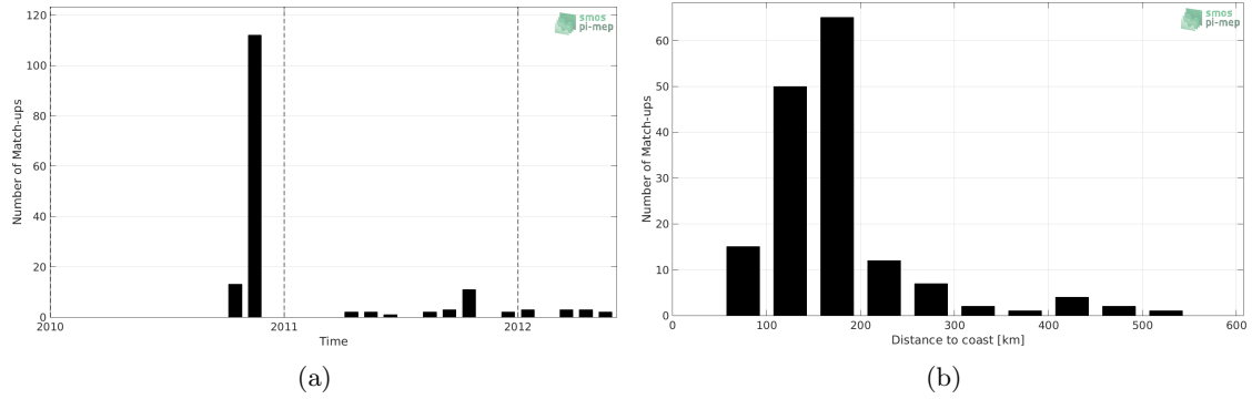
Figure 1: Number of match-ups between Surface drifters and SMOS SSS L2Q v321 - 0.25 Deg (CATDS-CPDC) SSS as a function of time (a) and as function of the distance to coast (b) over the Arctic Ocean Pi-MEP region and for the full satellite product period.
