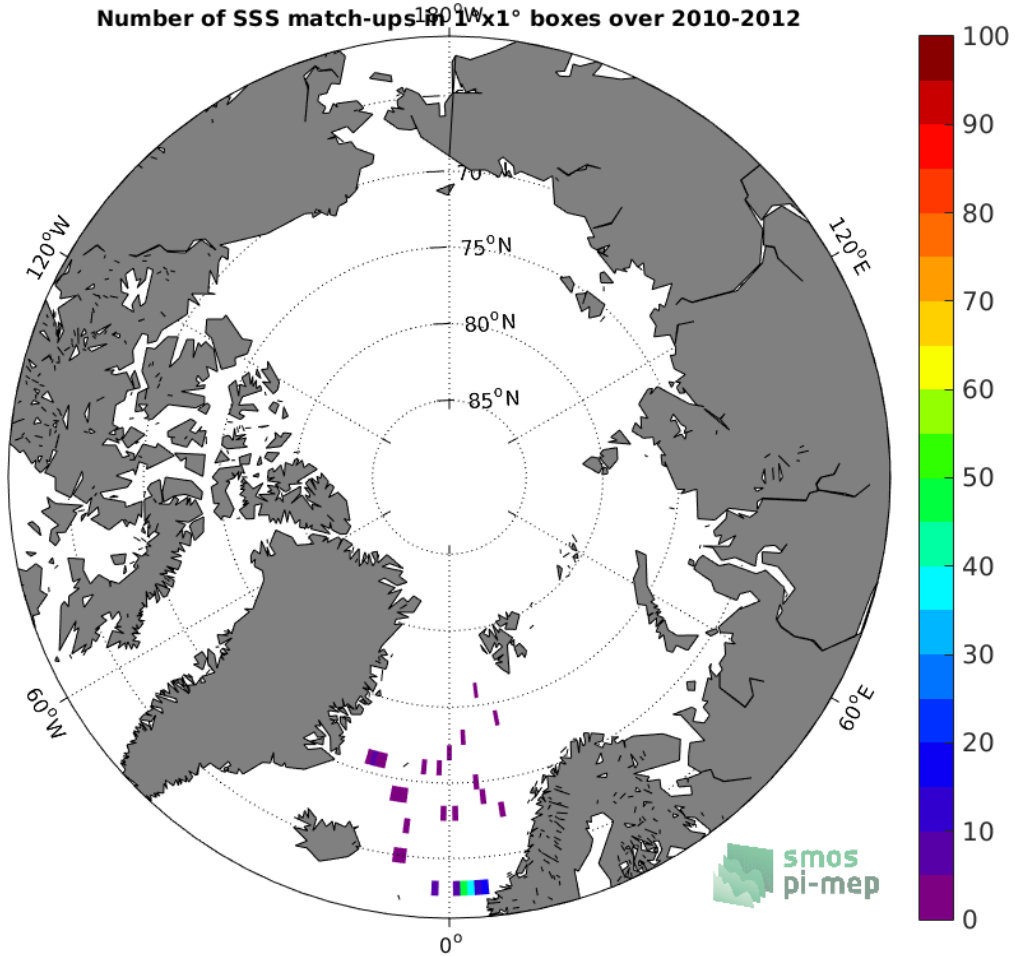
Figure 3: Number of SSS match-ups between Surface drifters SSS and the SMOS SSS L2Q v321 - 0.25 Deg (CATDS-CPDC) SSS product for the Arctic Ocean Pi-MEP region over 1°x1° boxes and for the full satellite product period.
