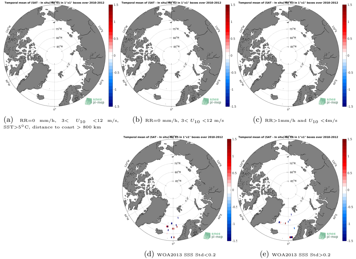
Figure 11: Temporal mean gridded over spatial boxes of size 1^{\circ}\times 1^{\circ} of \Delta\text{SSS} (SMOS SSS L2Q v321 - 0.25 Deg (CATDS-CPDC) - Surface drifters) for 5 different subdatasets corresponding to: RR=0 mm/h, 3 < U_{10} < 12 m/s, SST > 5^{\circ}\text{C} , distance to coast > 800 km (a), RR=0 mm/h, 3 < U_{10} < 12 m/s (b), RR > 1 mm/h and U_{10} < 4 m/s (c), WOA2013 SSS Std < 0.2 (d), WOA2013 SSS Std > 0.2 (e).
