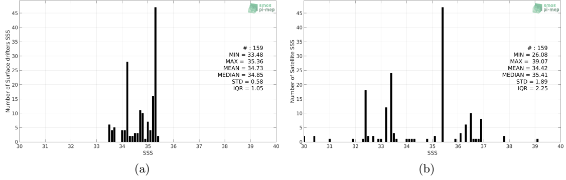
Figure 2: Histograms of SSS from Surface drifters (a) and SMOS SSS L2Q v321 - 0.25 Deg (CATDS-CPDC) (b) considering all match-up pairs per bins of 0.1 over the Arctic Ocean Pi-MEP region and for the full satellite product period.
