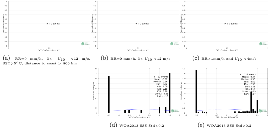
Figure 12: Normalized histogram of \Delta\text{SSS} (SMOS SSS L2Q v321 - 0.25 Deg (CATDS-CPDC) - Surface drifters) for 5 different subdatasets corresponding to: RR=0 mm/h, 3 < U_{10} < 12 m/s, SST > 5^\circ\text{C} , distance to coast > 800 km (a), RR=0 mm/h, 3 < U_{10} < 12 m/s (b), RR > 1 mm/h and U_{10} < 4 m/s (c), WOA2013 SSS Std < 0.2 (d), WOA2013 SSS Std > 0.2 (e).
