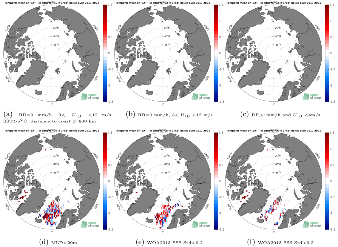
Figure 12: Temporal mean gridded over spatial boxes of size 1^{\circ} \times 1^{\circ} of \Delta\text{SSS} (SMOS SSS L2Q v321 - 0.25 Deg (CATDS-CPDC) - Argo) for 6 different subdatasets corresponding to:RR=0 mm/h, 3 < U_{10} < 12 m/s, SST >5^{\circ}\text{C} , distance to coast > 800 km (a), RR=0 mm/h, 3 < U_{10} < 12 m/s (b), RR >1 mm/h and U_{10} < 4 m/s (c),MLD <20 m (d),WOA2013 SSS Std <0.2 (e),WOA2013 SSS Std >0.2 (f).
