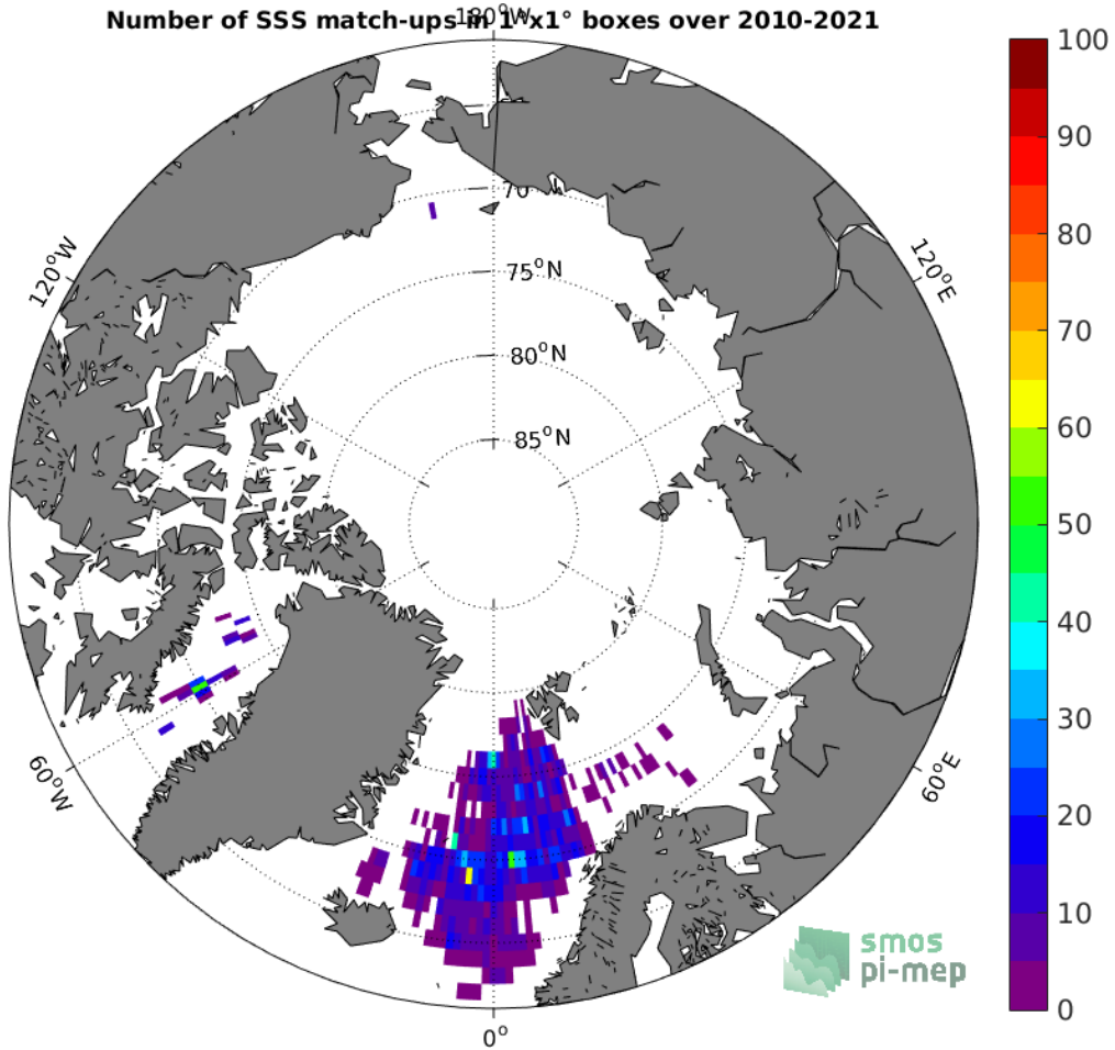
Figure 4: Number of SSS match-ups between Argo SSS and the SMOS SSS L2Q v321 - 0.25 Deg (CATDS-CPDC) SSS product for the Arctic Ocean Pi-MEP region over 1^\circ \times 1^\circ boxes and for the full satellite product period.
