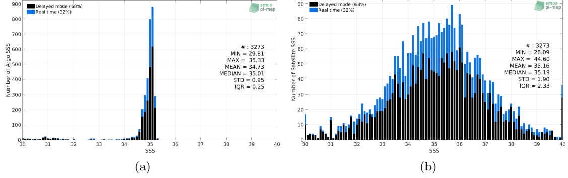
Figure 2: Histograms of SSS from Argo (a) and SMOS SSS L2Q v321 - 0.25 Deg (CATDS-CPDC) (b) considering all match-up pairs per bins of 0.1 over the Arctic Ocean Pi-MEP region and for the full satellite product period.
