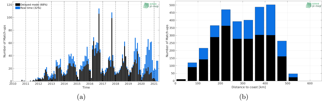
Figure 1: Number of match-ups between Argo and SMOS SSS L2Q v321 - 0.25 Deg (CATDS-CPDC) SSS as a function of time (a) and as function of the distance to coast (b) over the Arctic Ocean Pi-MEP region and for the full satellite product period.
