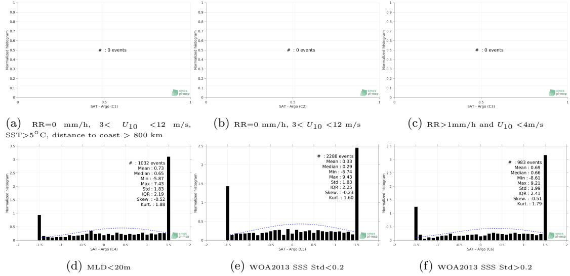
Figure 13: Normalized histogram of \Delta\text{SSS} (SMOS SSS L2Q v321 - 0.25 Deg (CATDS-CPDC) - Argo) for 6 different subdatasets corresponding to: RR=0 mm/h, 3 < U_{10} < 12 m/s, SST > 5^\circ\text{C} , distance to coast > 800 km (a), RR=0 mm/h, 3 < U_{10} < 12 m/s (b), RR > 1 mm/h and U_{10} < 4 m/s (c), MLD < 20 m (d), WOA2013 SSS Std < 0.2 (e), WOA2013 SSS Std > 0.2 (f).
