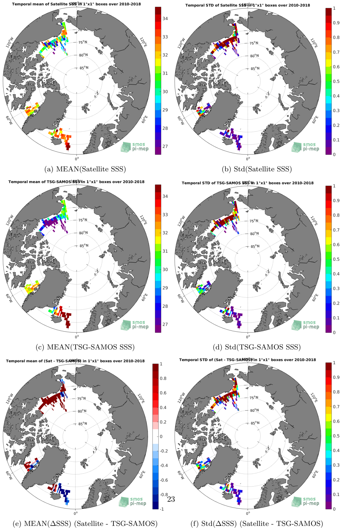
Figure 6: Temporal mean (left) and Std (right) of SSS from SMOS-L3-CATDS-CPDC-V317-MONTHLY-25KM (top), TSG-SAMOS (middle), and of \Delta SSS (Satellite - TSG-SAMOS). Only match-up pairs are used to generate these maps.
