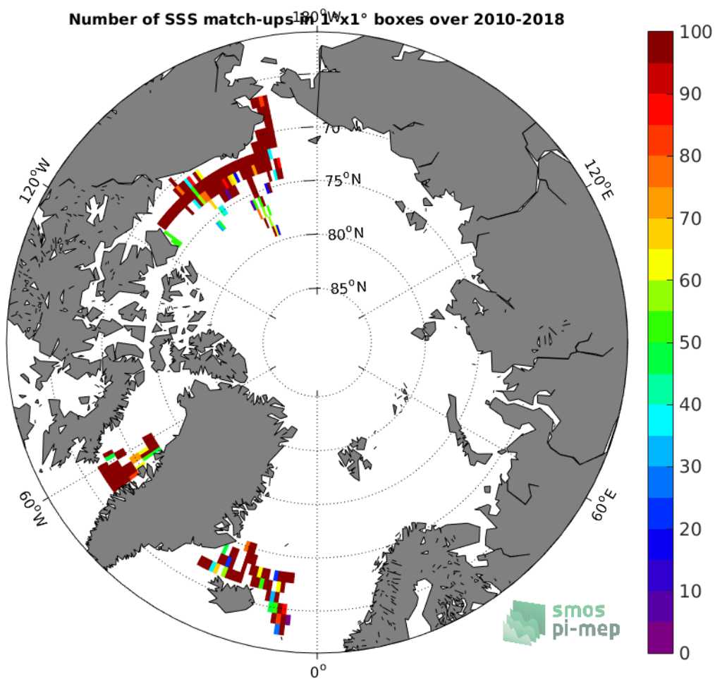
Figure 4: Number of SSS match-ups between TSG-SAMOS SSS and the SMOS-L3-CATDS-CPDC-V317-MONTHLY-25KM SSS product for the Arctic Ocean Pi-MEP region over 1^\circ \times 1^\circ boxes and for the full satellite product period.
