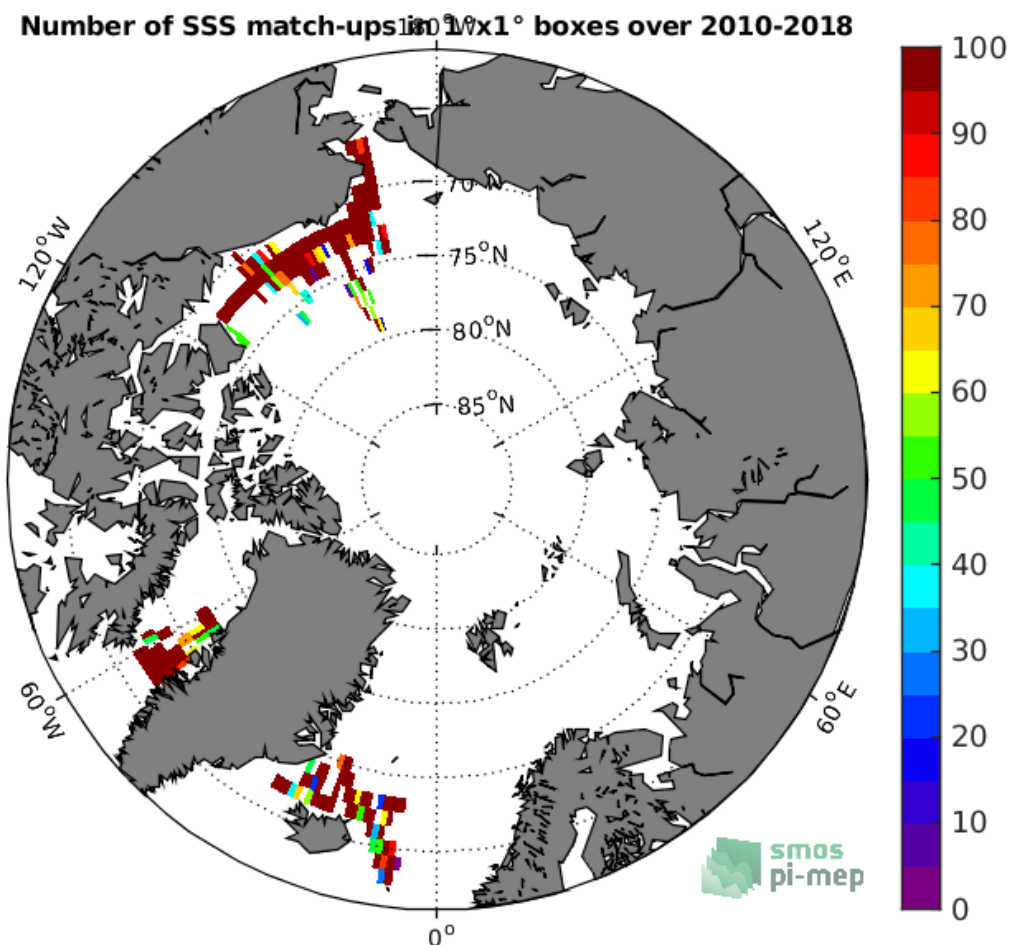
Figure 4: Number of SSS match-ups between TSG-SAMOS SSS and the SMOS-L3-CATDS-CPDC-V317-MONTHLY-25KM SSS product for the Arctic Ocean Pi-MEP region over 1°x1° boxes and for the full satellite product period.
