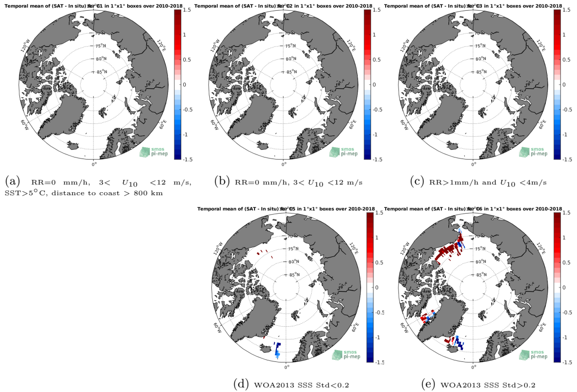
Figure 12: Temporal mean gridded over spatial boxes of size 1^\circ \times 1^\circ of \Delta SSS (SMOS-L3-CATDS-CPDC-V317-MONTHLY-25KM - TSG-SAMOS) for 5 different subdatasets corresponding to: RR=0 mm/h, 3 < U_{10} < 12 m/s, SST > 5^\circ\text{C} , distance to coast > 800 km (a), RR=0 mm/h, 3 < U_{10} < 12 m/s (b), RR > 1 mm/h and U_{10} < 4 m/s (c), WOA2013 SSS Std < 0.2 (d), WOA2013 SSS Std > 0.2 (e).
