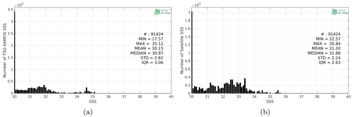
Figure 2: Histograms of SSS from TSG-SAMOS (a) and SMOS-L3-CATDS-CPDC-V317-MONTHLY-25KM (b) considering all match-up pairs per bins of 0.1 over the Arctic Ocean Pi-MEP region and for the full satellite product period.
