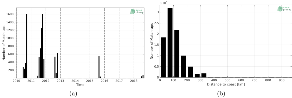
Figure 1: Number of match-ups between TSG-SAMOS and SMOS-L3-CATDS-CPDC-V317-MONTHLY-25KM SSS as a function of time (a) and as function of the distance to coast (b) over the Arctic Ocean Pi-MEP region and for the full satellite product period.
