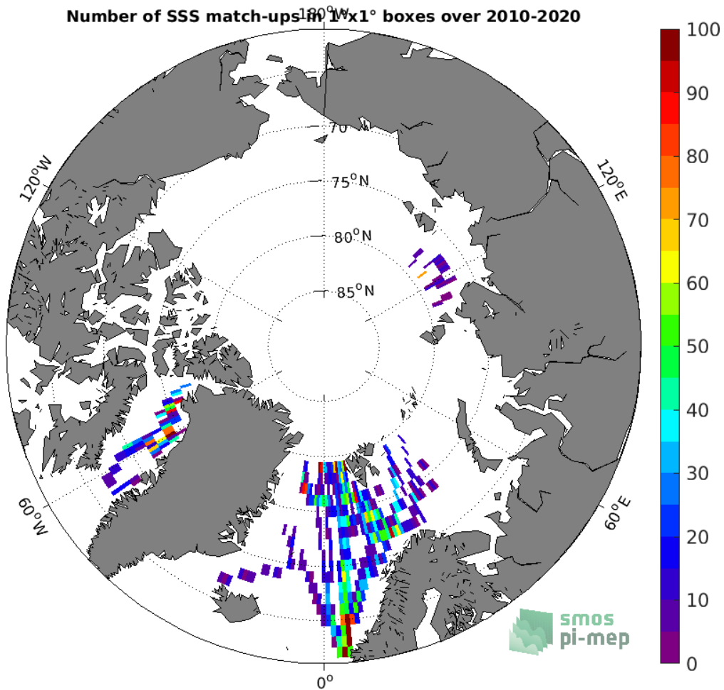
Figure 4: Number of SSS match-ups between TSG (Polarstern) SSS and the SMOS SSS L3 v317 - Monthly - 25 km (CATDS-CPDC) SSS product for the Arctic Ocean Pi-MEP region over 1^\circ \times 1^\circ boxes and for the full satellite product period.
