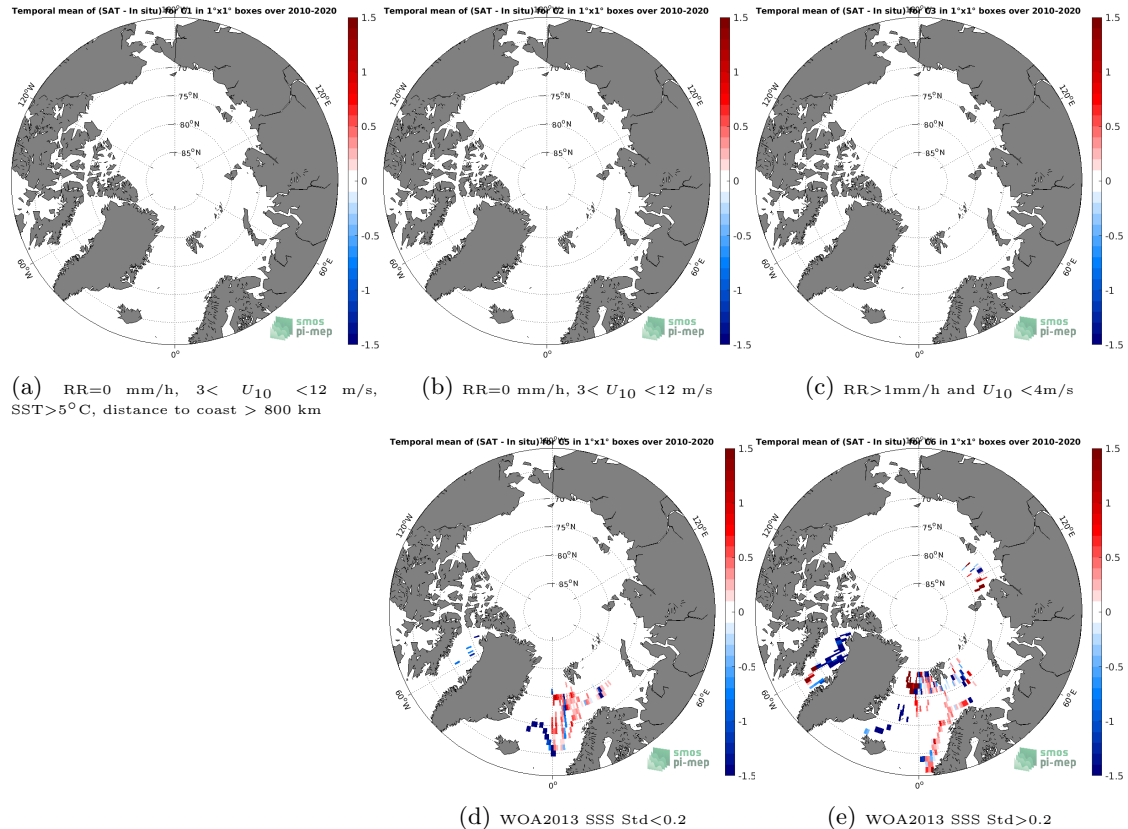
Figure 12: Temporal mean gridded over spatial boxes of size 1^{\circ}\times 1^{\circ} of \Delta\text{SSS} (SMOS SSS L3 v317 - Monthly - 25 km (CATDS-CPDC) - TSG (Polarstern)) for 5 different subdatasets corresponding to:RR=0 mm/h, 3 < U_{10} < 12 m/s, SST >5^{\circ}\text{C} , distance to coast > 800 km (a), RR=0 mm/h, 3 < U_{10} < 12 m/s (b), RR >1 mm/h and U_{10} < 4 m/s (c), WOA2013 SSS Std <0.2 (d), WOA2013 SSS Std >0.2 (e).
