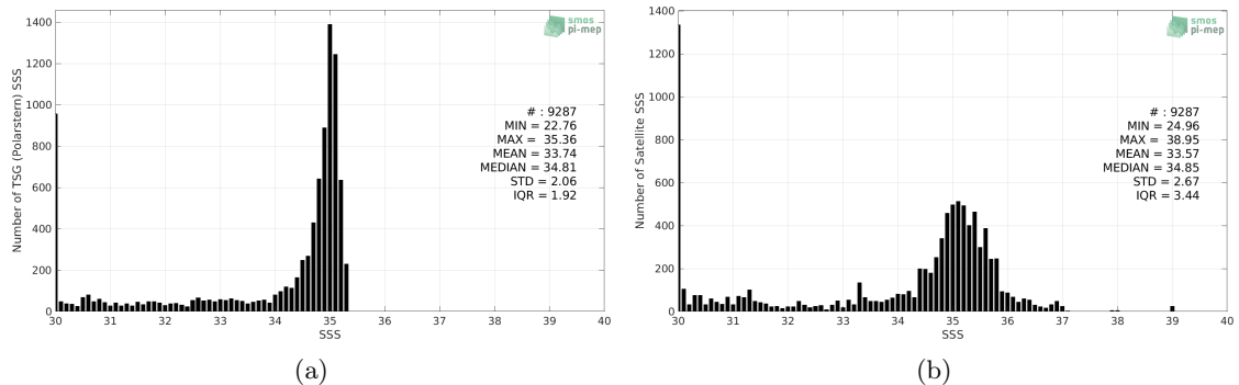
Figure 2: Histograms of SSS from TSG (Polarstern) (a) and SMOS SSS L3 v317 - Monthly - 25 km (CATDS-CPDC) (b) considering all match-up pairs per bins of 0.1 over the Arctic Ocean Pi-MEP region and for the full satellite product period.
