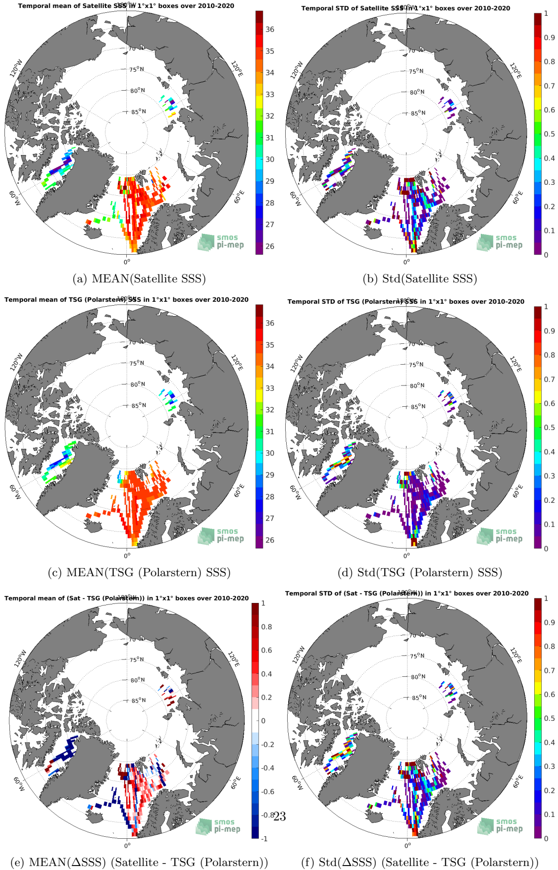
Figure 6: Temporal mean (left) and Std (right) of SSS from SMOS SSS L3 v317 - Monthly - 25 km (CATDS-CPDC) (top), TSG (Polarstern) (middle), and of \Delta SSS (Satellite - TSG (Polarstern)). Only match-up pairs are used to generate these maps.
