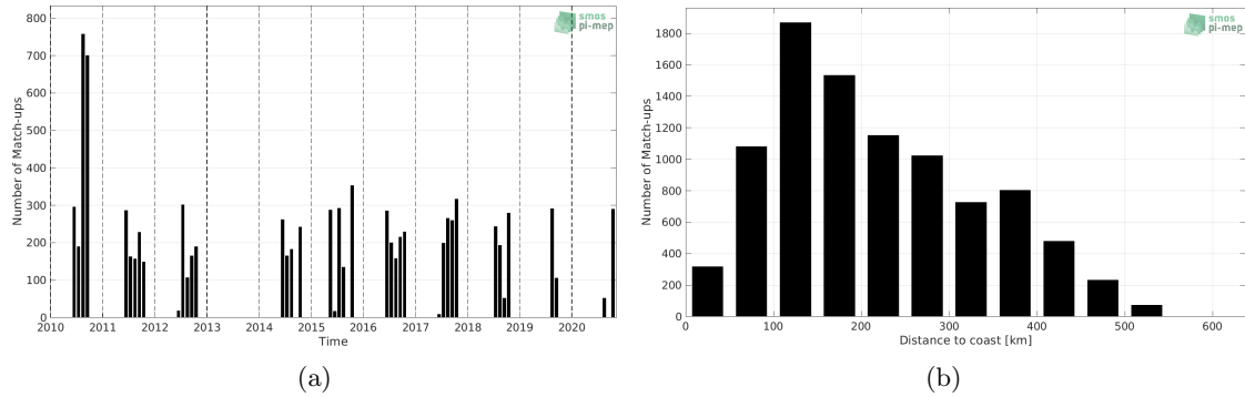
Figure 1: Number of match-ups between TSG (Polarstern) and SMOS SSS L3 v317 - Monthly - 25 km (CATDS-CPDC) SSS as a function of time (a) and as function of the distance to coast (b) over the Arctic Ocean Pi-MEP region and for the full satellite product period.
