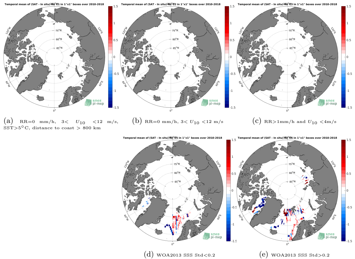
Figure 12: Temporal mean gridded over spatial boxes of size 1^{\circ}\times 1^{\circ} of \Delta\text{SSS} (SMOS L3 v317 - Monthly - 25 km (CATDS-CPDC) - TSG-POLARSTERN) for 5 different subdatasets corresponding to:RR=0 mm/h, 3 < U_{10} < 12 m/s, SST > 5^{\circ}\text{C} , distance to coast > 800 km (a), RR=0 mm/h, 3 < U_{10} < 12 m/s (b), RR > 1 mm/h and U_{10} < 4 m/s (c), WOA2013 SSS Std < 0.2 (d), WOA2013 SSS Std > 0.2 (e).
