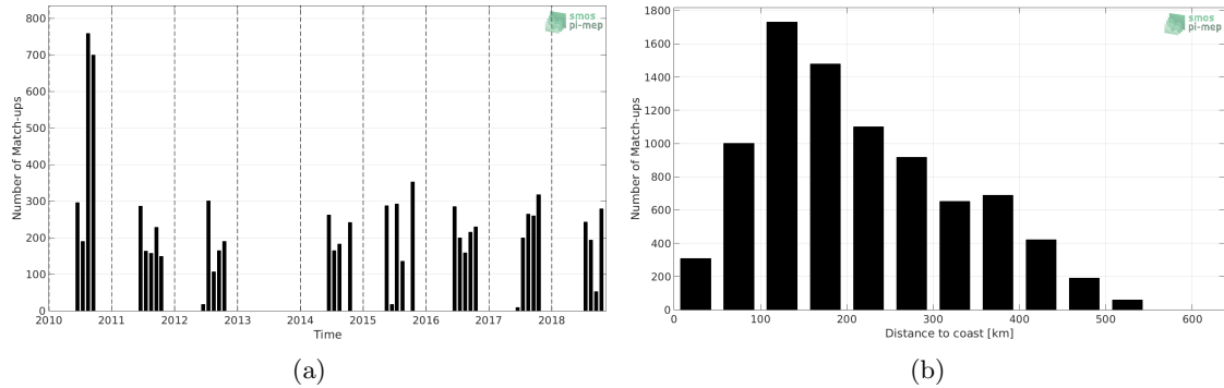
Figure 1: Number of match-ups between TSG-POLARSTERN and SMOS L3 v317 - Monthly - 25 km (CATDS-CPDC) SSS as a function of time (a) and as function of the distance to coast (b) over the Arctic Ocean Pi-MEP region and for the full satellite product period.
