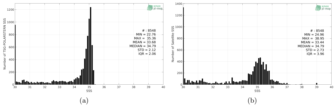
Figure 2: Histograms of SSS from TSG-POLARSTERN (a) and SMOS L3 v317 - Monthly - 25 km (CATDS-CPDC) (b) considering all match-up pairs per bins of 0.1 over the Arctic Ocean Pi-MEP region and for the full satellite product period.
