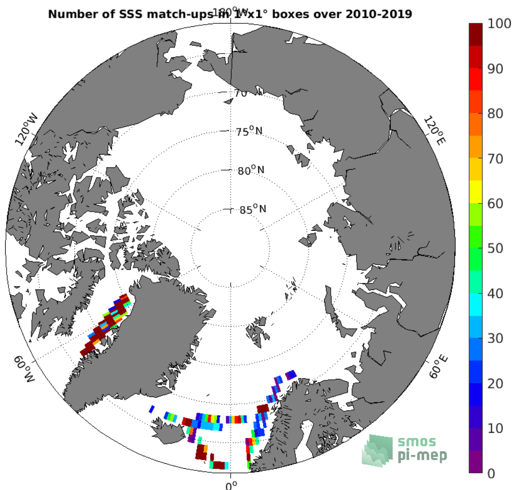
Figure 4: Number of SSS match-ups between TSG (LEGOS-DM) SSS and the SMOS SSS L3 v317 - Monthly - 25 km (CATDS-CPDC) SSS product for the Arctic Ocean Pi-MEP region over 1°x1° boxes and for the full satellite product period.
