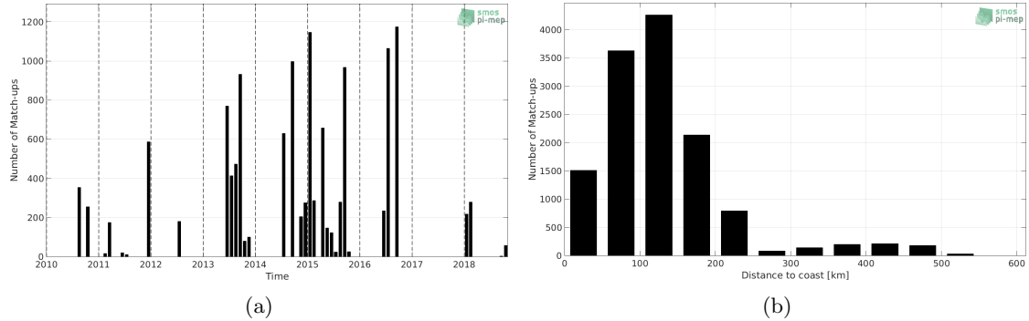
Figure 1: Number of match-ups between TSG-LEGOS-DM and SMOS L3 v317 - Monthly - 25 km (CATDS-CPDC) SSS as a function of time (a) and as function of the distance to coast (b) over the Arctic Ocean Pi-MEP region and for the full satellite product period.
