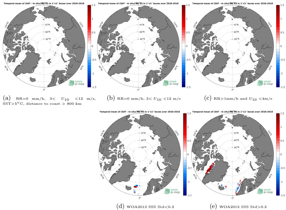
Figure 12: Temporal mean gridded over spatial boxes of size 1^{\circ}\times 1^{\circ} of \Delta\text{SSS} (SMOS L3 v317 - Monthly - 25 km (CATDS-CPDC) - TSG-LEGOS-DM) for 5 different subdatasets corresponding to: RR=0 mm/h, 3 < U_{10} < 12 m/s, SST > 5^{\circ}\text{C} , distance to coast > 800 km (a), RR=0 mm/h, 3 < U_{10} < 12 m/s (b), RR > 1 mm/h and U_{10} < 4 m/s (c), WOA2013 SSS Std < 0.2 (d), WOA2013 SSS Std > 0.2 (e).
