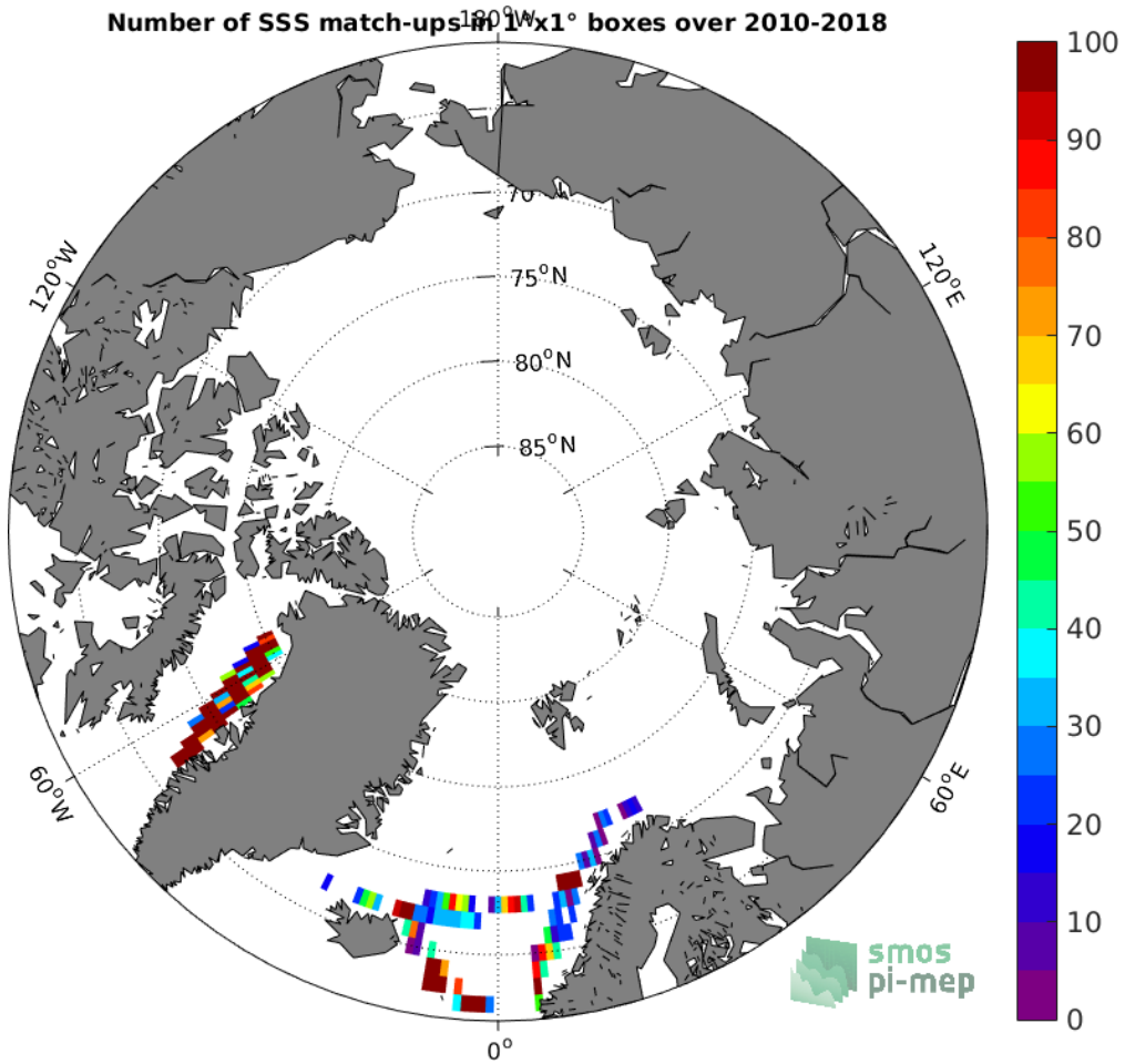
Figure 4: Number of SSS match-ups between TSG-LEGOS-DM SSS and the SMOS L3 v317 - Monthly - 25 km (CATDS-CPDC) SSS product for the Arctic Ocean Pi-MEP region over 1°x1° boxes and for the full satellite product period.
