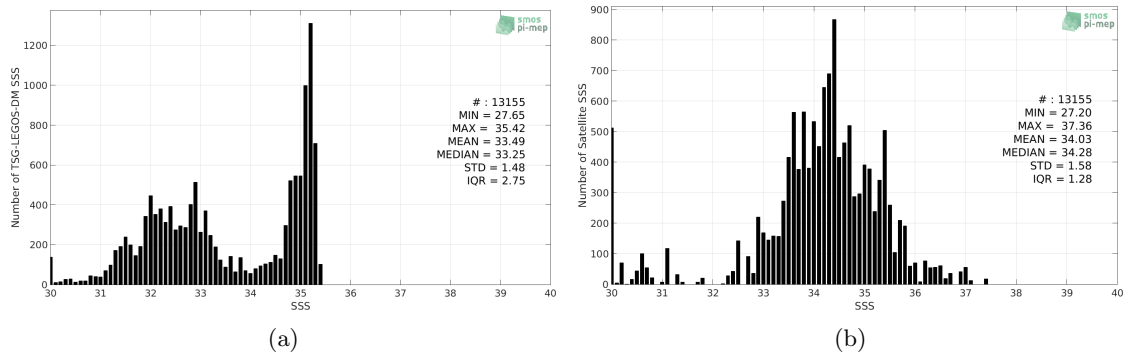
Figure 2: Histograms of SSS from TSG-LEGOS-DM (a) and SMOS L3 v317 - Monthly - 25 km (CATDS-CPDC) (b) considering all match-up pairs per bins of 0.1 over the Arctic Ocean Pi-MEP region and for the full satellite product period.
