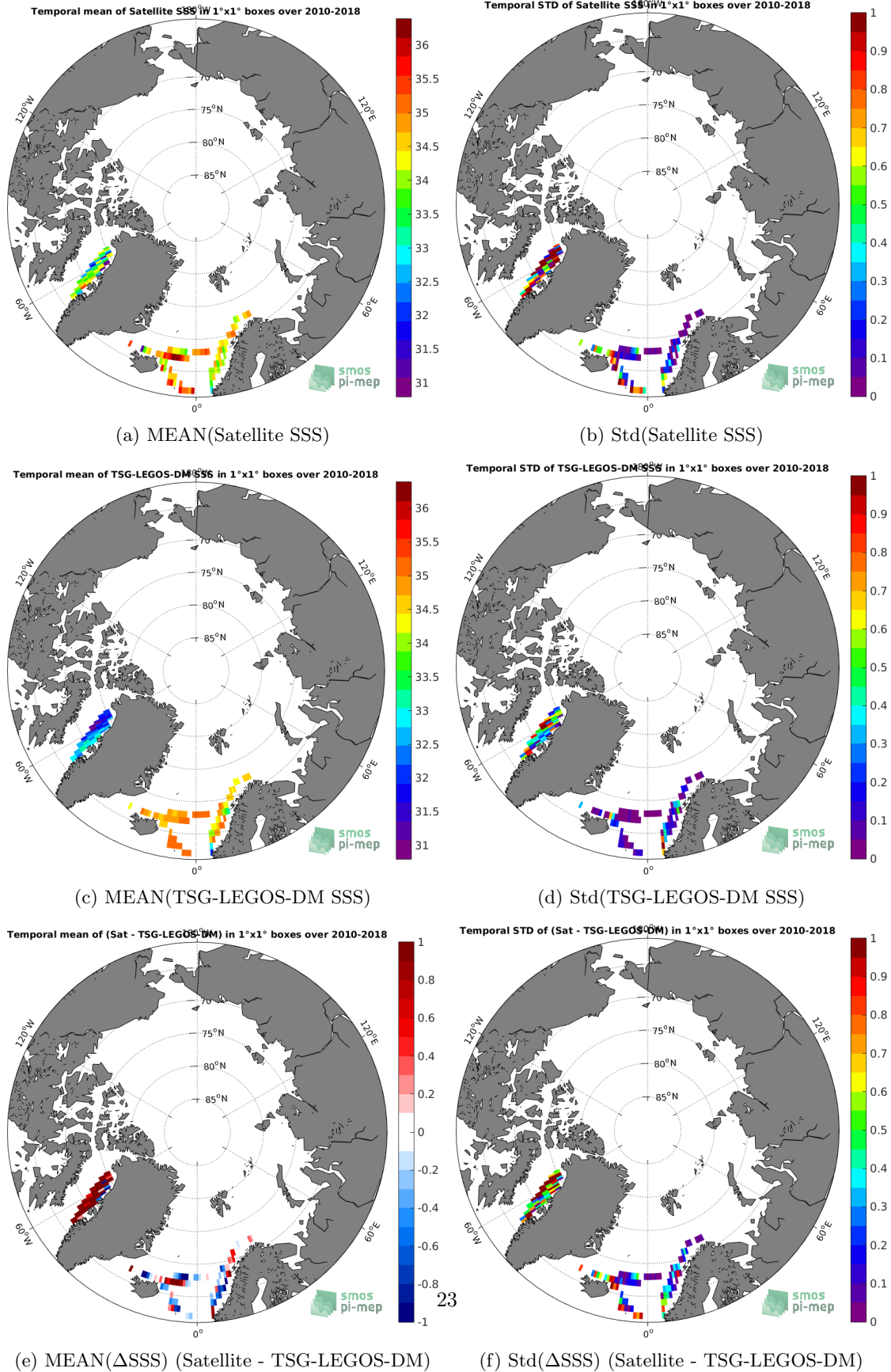
Figure 6: Temporal mean (left) and Std (right) of SSS from SMOS L3 v317 - Monthly - 25 km (CATDS-CPDC) (top), TSG-LEGOS-DM (middle), and of \Delta SSS (Satellite - TSG-LEGOS-DM). Only match-up pairs are used to generate these maps.
