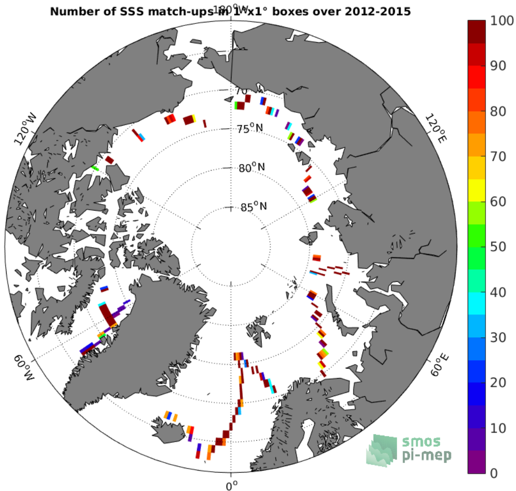
Figure 4: Number of SSS match-ups between TSG (GOSUD-Sailing-ship) SSS and the SMOS SSS L3 v317 - Monthly - 25 km (CATDS-CPDC) SSS product for the Arctic Ocean Pi-MEP region over 1^\circ \times 1^\circ boxes and for the full satellite product period.
