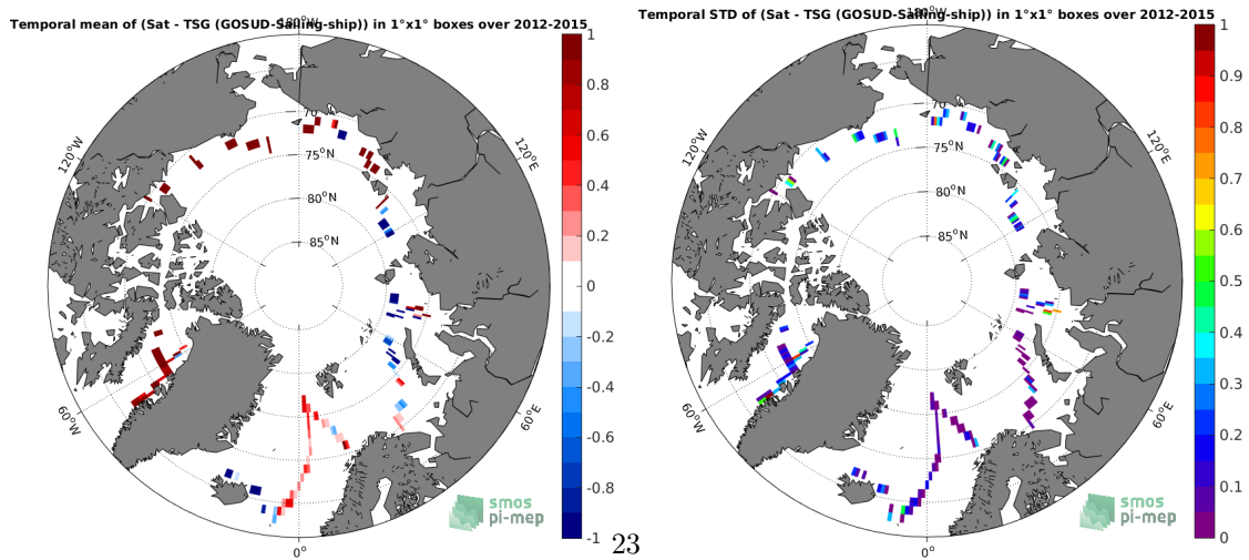
(e) MEAN( \Delta SSS) (Satellite - TSG (GOSUD-Sailing-ship))
