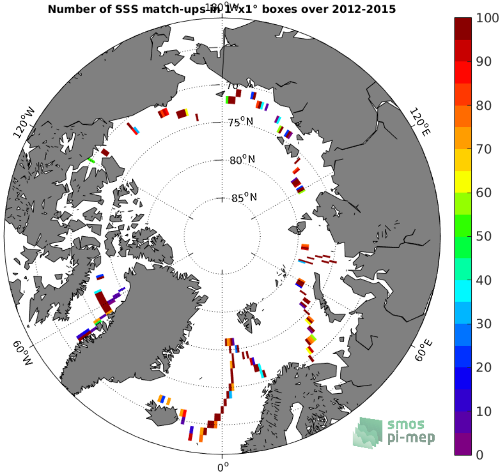
Figure 4: Number of SSS match-ups between TSG (GOSUD-Sailing-ship) SSS and the SMOS SSS L3 v317 - Monthly - 25 km (CATDS-CPDC) SSS product for the Arctic Ocean Pi-MEP region over 1°x1° boxes and for the full satellite product period.
