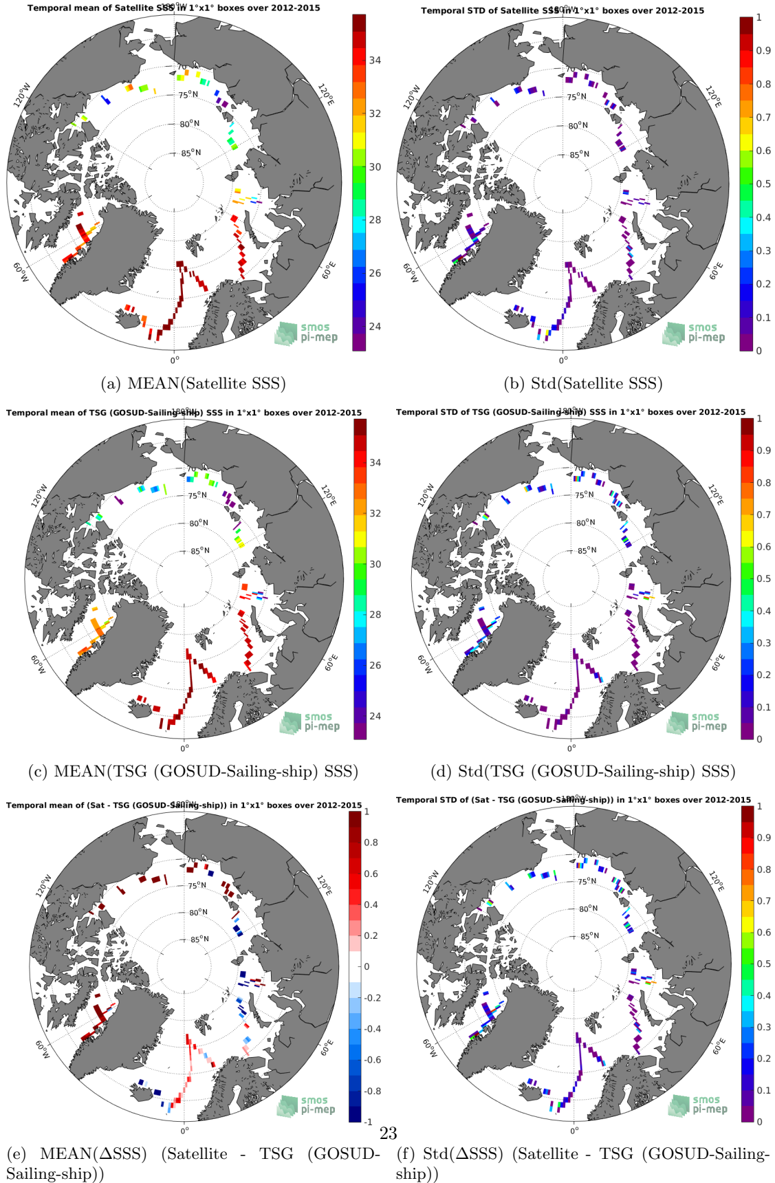
Figure 6: Temporal mean (left) and Std (right) of SSS from SMOS SSS L3 v317 - Monthly - 25 km (CATDS-CPDC) (top), TSG (GOSUD-Sailing-ship) (middle), and of \Delta SSS (Satellite - TSG (GOSUD-Sailing-ship)). Only match-up pairs are used to generate these maps.
