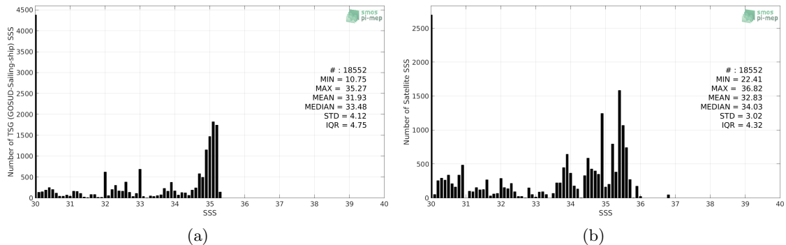
Figure 2: Histograms of SSS from TSG (GOSUD-Sailing-ship) (a) and SMOS SSS L3 v317 - Monthly - 25 km (CATDS-CPDC) (b) considering all match-up pairs per bins of 0.1 over the Arctic Ocean Pi-MEP region and for the full satellite product period.
