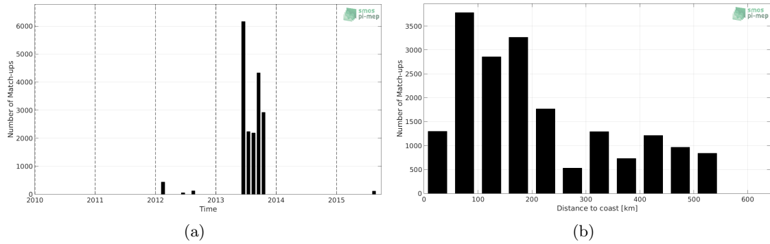
Figure 1: Number of match-ups between TSG (GOSUD-Sailing-ship) and SMOS SSS L3 v317 - Monthly - 25 km (CATDS-CPDC) SSS as a function of time (a) and as function of the distance to coast (b) over the Arctic Ocean Pi-MEP region and for the full satellite product period.
