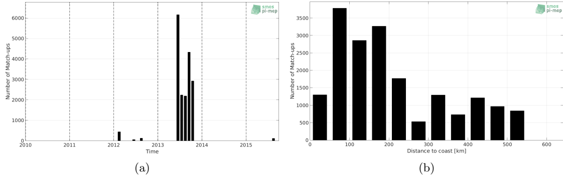
Figure 1: Number of match-ups between TSG-GOSUD-Sailing-ship and SMOS L3 v317 - Monthly - 25 km (CATDS-CPDC) SSS as a function of time (a) and as function of the distance to coast (b) over the Arctic Ocean Pi-MEP region and for the full satellite product period.
