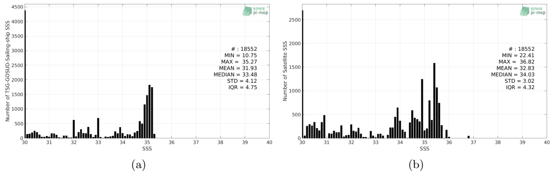
Figure 2: Histograms of SSS from TSG-GOSUD-Sailing-ship (a) and SMOS L3 v317 - Monthly - 25 km (CATDS-CPDC) (b) considering all match-up pairs per bins of 0.1 over the Arctic Ocean Pi-MEP region and for the full satellite product period.
