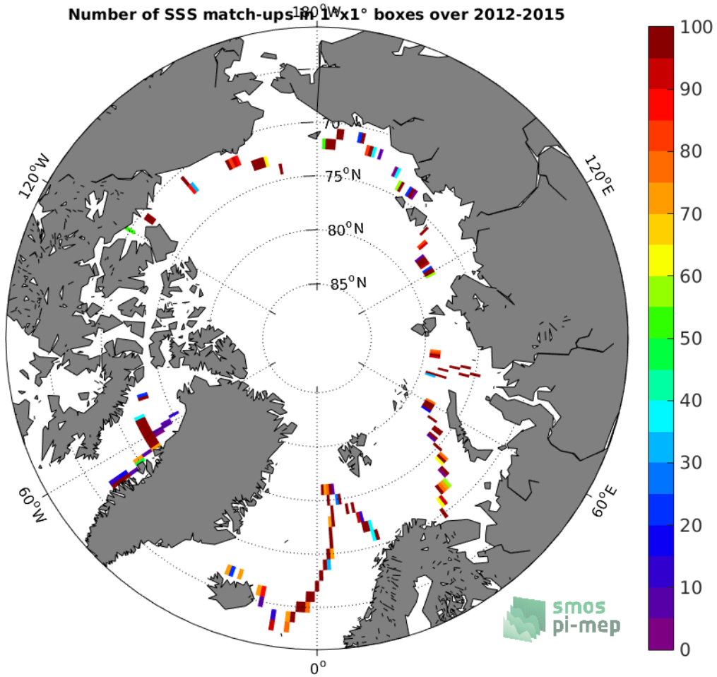
Figure 4: Number of SSS match-ups between TSG-GOSUD-Sailing-ship SSS and the SMOS L3 v317 - Monthly - 25 km (CATDS-CPDC) SSS product for the Arctic Ocean Pi-MEP region over 1°x1° boxes and for the full satellite product period.
