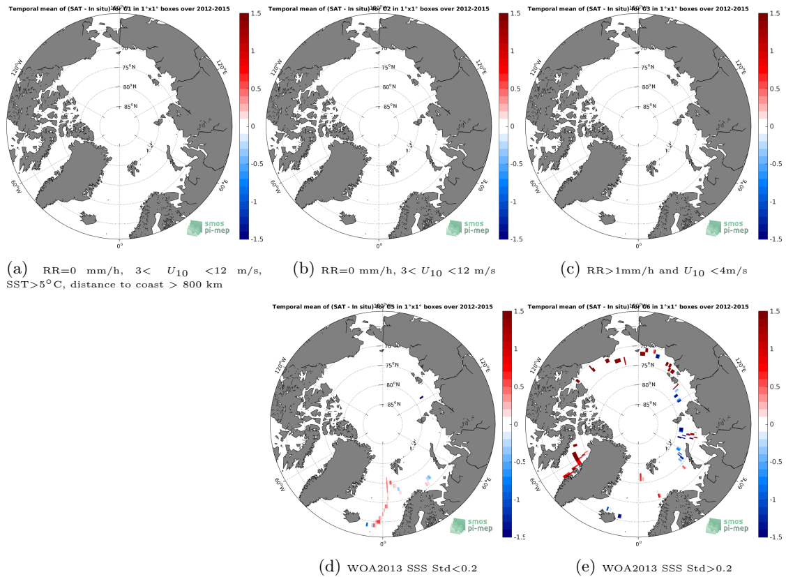
Figure 12: Temporal mean gridded over spatial boxes of size 1°x1° of \Delta SSS (SMOS L3 v317 - Monthly - 25 km (CATDS-CPDC) - TSG-GOSUD-Sailing-ship) for 5 different subdatasets corresponding to: RR=0 mm/h, 3 < U_{10} < 12 m/s, SST > 5°C, distance to coast > 800 km (a), RR=0 mm/h, 3 < U_{10} < 12 m/s (b), RR > 1mm/h and U_{10} < 4 m/s (c), WOA2013 SSS Std < 0.2 (d), WOA2013 SSS Std > 0.2 (e).
