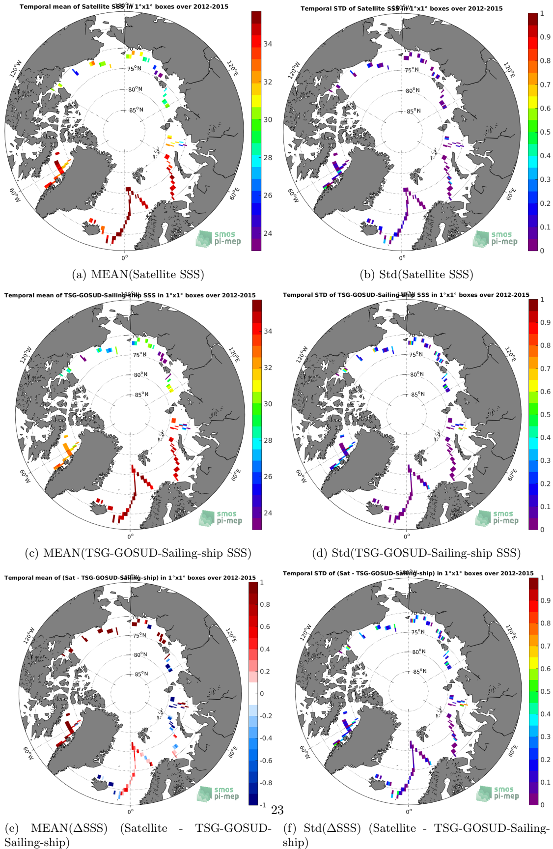
Figure 6: Temporal mean (left) and Std (right) of SSS from SMOS-L3-CATDS-CPDC-V317-MONTHLY-25KM (top), TSG-GOSUD-Sailing-ship (middle), and of \Delta SSS (Satellite - TSG-GOSUD-Sailing-ship). Only match-up pairs are used to generate these maps.
