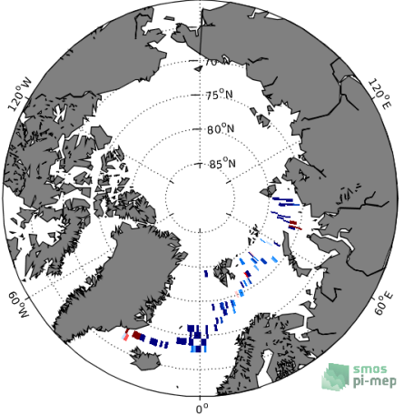
(e) MEAN( \Delta SSS) (Satellite - Sea mammals)
