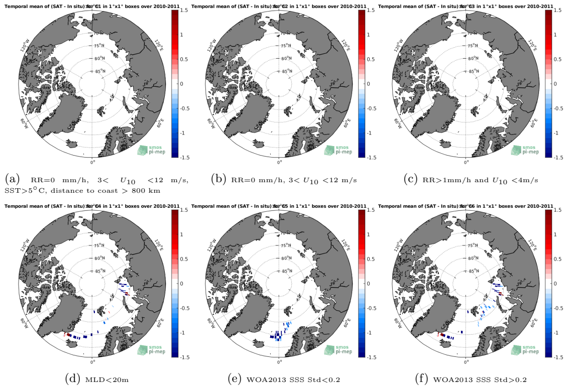
Figure 12: Temporal mean gridded over spatial boxes of size 1^\circ \times 1^\circ of \Delta SSS (SMOS-L3-CATDS-CPDC-V317-MONTHLY-25KM - Sea mammals) for 6 different subdatasets corresponding to:RR=0 mm/h, 3 < U_{10} < 12 m/s, SST >5^\circ C, distance to coast > 800 km (a), RR=0 mm/h, 3 < U_{10} < 12 m/s (b), RR >1 mm/h and U_{10} < 4 m/s (c),MLD <20 m (d),WOA2013 SSS Std <0.2 (e),WOA2013 SSS Std >0.2 (f).
