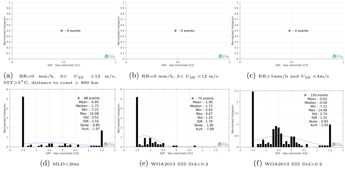
Figure 13: Normalized histogram of \Delta SSS (SMOS-L3-CATDS-CPDC-V317-MONTHLY-25KM - Sea mammals) for 6 different subdatasets corresponding to: RR=0 mm/h, 3 < U_{10} < 12 m/s, SST>5°C, distance to coast > 800 km (a), RR=0 mm/h, 3 < U_{10} < 12 m/s (b), RR>1mm/h and U_{10} < 4 m/s (c), MLD<20m (d), WOA2013 SSS Std<0.2 (e), WOA2013 SSS Std>0.2 (f).
