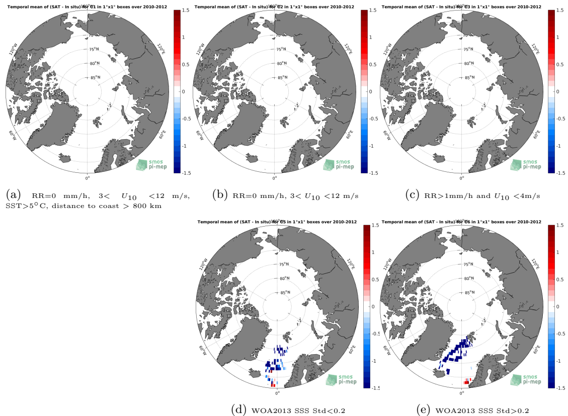
Figure 11: Temporal mean gridded over spatial boxes of size 1^{\circ}\times 1^{\circ} of \Delta\text{SSS} (SMOS L3 v317 - Monthly - 25 km (CATDS-CPDC) - Surface drifters) for 5 different subdatasets corresponding to: RR=0 mm/h, 3 < U_{10} < 12 m/s, SST > 5^{\circ}\text{C} , distance to coast > 800 km (a), RR=0 mm/h, 3 < U_{10} < 12 m/s (b), RR > 1 mm/h and U_{10} < 4 m/s (c), WOA2013 SSS Std < 0.2 (d), WOA2013 SSS Std > 0.2 (e).
