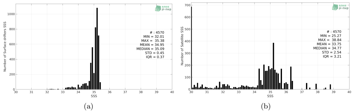
Figure 2: Histograms of SSS from Surface drifters (a) and SMOS L3 v317 - Monthly - 25 km (CATDS-CPDC) (b) considering all match-up pairs per bins of 0.1 over the Arctic Ocean Pi-MEP region and for the full satellite product period.
