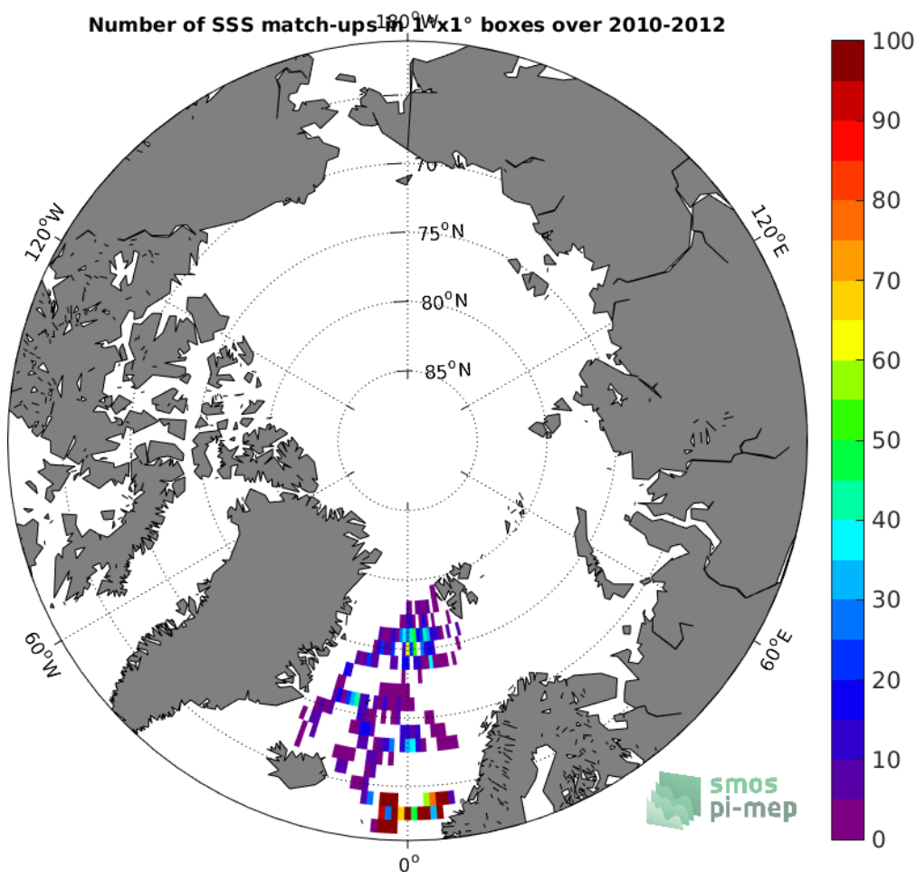
Figure 3: Number of SSS match-ups between Surface drifters SSS and the SMOS L3 v317 - Monthly - 25 km (CATDS-CPDC) SSS product for the Arctic Ocean Pi-MEP region over 1°x1° boxes and for the full satellite product period.
