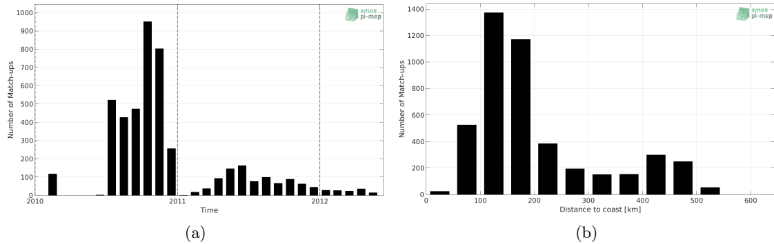
Figure 1: Number of match-ups between Surface drifters and SMOS L3 v317 - Monthly - 25 km (CATDS-CPDC) SSS as a function of time (a) and as function of the distance to coast (b) over the Arctic Ocean Pi-MEP region and for the full satellite product period.
