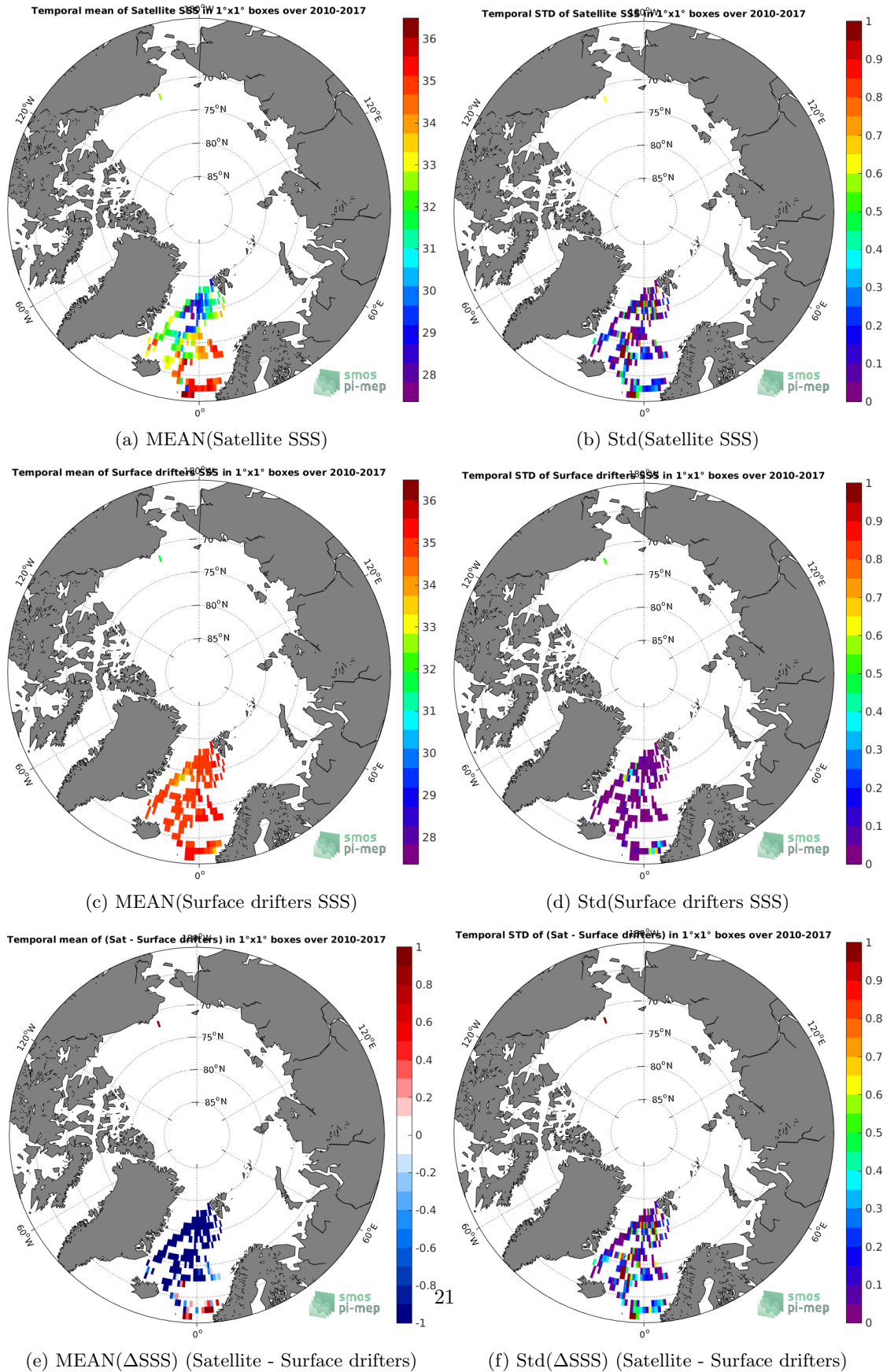
Figure 5: Temporal mean (left) and Std (right) of SSS from SMOS-L3-CATDS-CPDC-V317-MONTHLY-25KM (top), Surface drifters (middle), and of \Delta SSS (Satellite - Surface drifters). Only match-up pairs are used to generate these maps.
