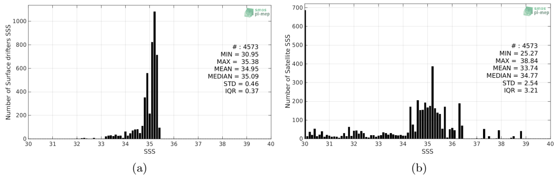
Figure 2: Histograms of SSS from Surface drifters (a) and SMOS-L3-CATDS-CPDC-V317-MONTHLY-25KM (b) considering all match-up pairs per bins of 0.1 over the Arctic Ocean Pi-MEP region and for the full satellite product period.
