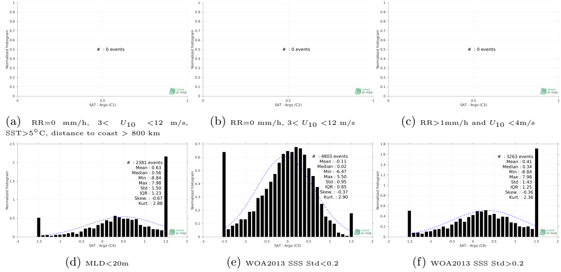
Figure 13: Normalized histogram of \Delta SSS (SMOS SSS L3 v317 - Monthly - 25 km (CATDS-CPDC) - Argo) for 6 different subdatasets corresponding to: RR=0 mm/h, 3 < U_{10} < 12 m/s, SST > 5°C, distance to coast > 800 km (a), RR=0 mm/h, 3 < U_{10} < 12 m/s (b), RR > 1mm/h and U_{10} < 4 m/s (c), MLD < 20m (d), WOA2013 SSS Std < 0.2 (e), WOA2013 SSS Std > 0.2 (f).
