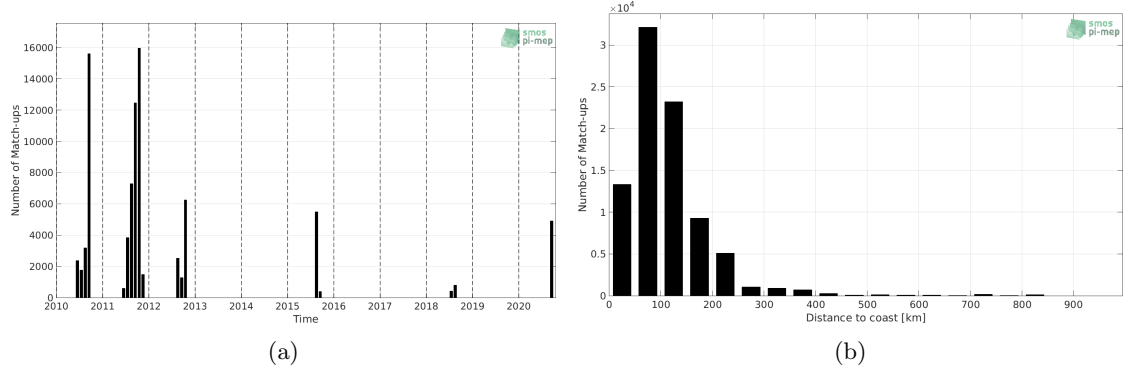
Figure 1: Number of match-ups between TSG (SAMOS) and SMOS SSS L3 v317 - 10 Days - 25 km (CATDS-CPDC) SSS as a function of time (a) and as function of the distance to coast (b) over the Arctic Ocean Pi-MEP region and for the full satellite product period.
