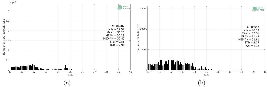
Figure 2: Histograms of SSS from TSG (SAMOS) (a) and SMOS SSS L3 v317 - 10 Days - 25 km (CATDS-CPDC) (b) considering all match-up pairs per bins of 0.1 over the Arctic Ocean Pi-MEP region and for the full satellite product period.
