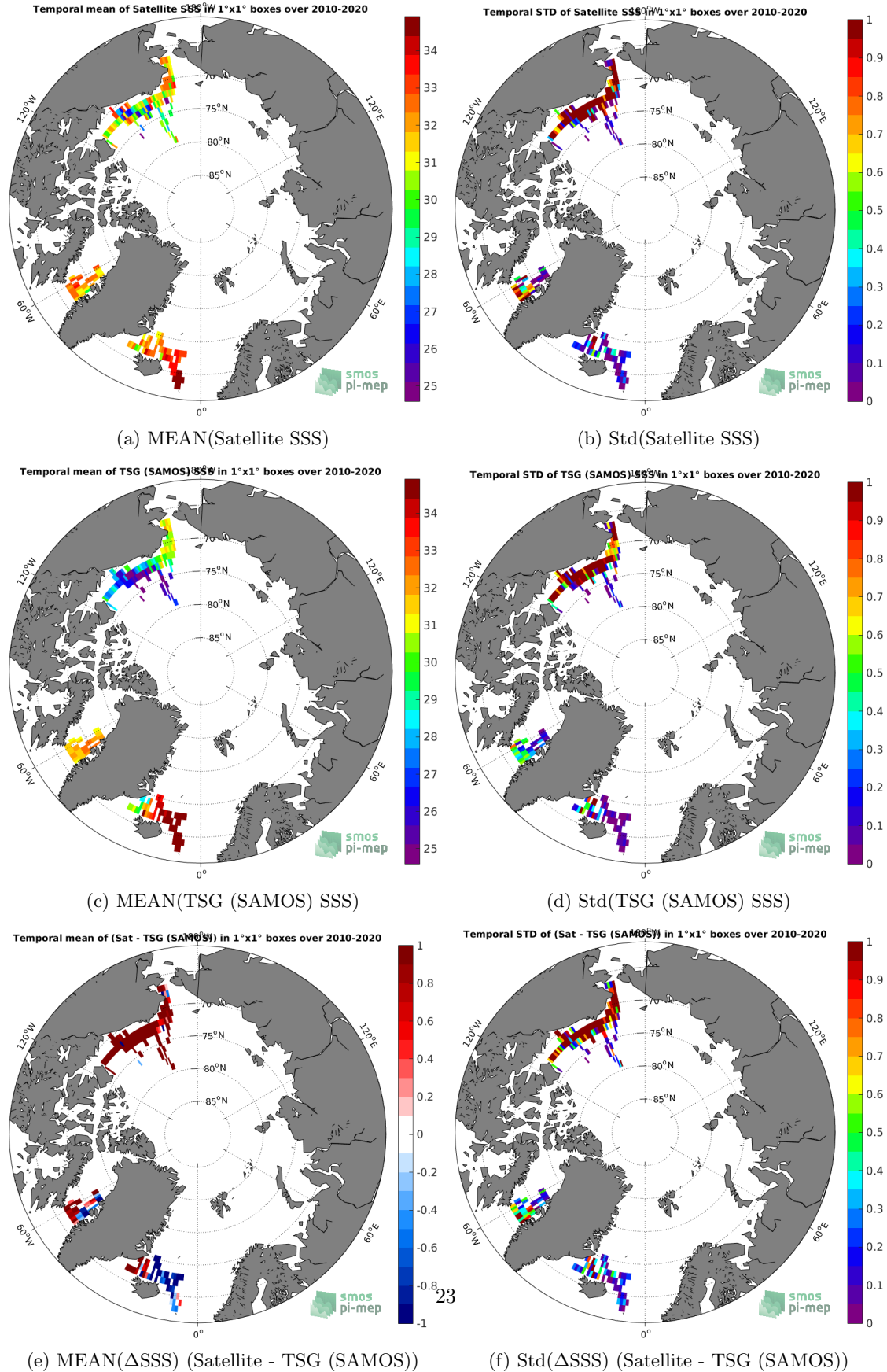
Figure 6: Temporal mean (left) and Std (right) of SSS from SMOS SSS L3 v317 - 10 Days - 25 km (CATDS-CPDC) (top), TSG (SAMOS) (middle), and of \Delta SSS (Satellite - TSG (SAMOS)). Only match-up pairs are used to generate these maps.
