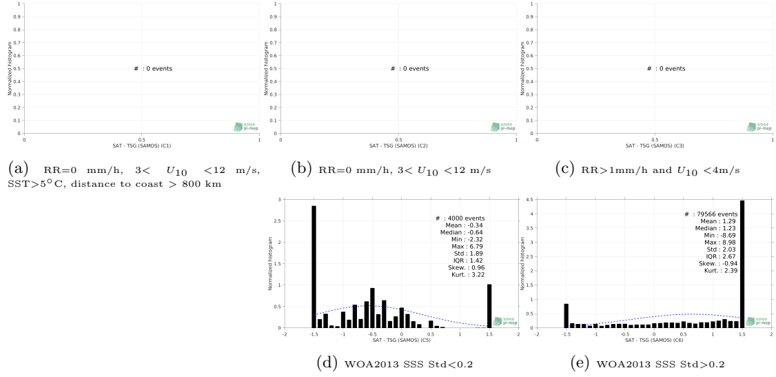
Figure 13: Normalized histogram of \Delta\text{SSS} (SMOS SSS L3 v317 - 10 Days - 25 km (CATDS-CPDC) - TSG (SAMOS)) for 5 different subdatasets corresponding to: RR=0 mm/h, 3 < U_{10} < 12 m/s, SST > 5^\circ\text{C} , distance to coast > 800 km (a), RR=0 mm/h, 3 < U_{10} < 12 m/s (b), RR > 1 mm/h and U_{10} < 4 m/s (c), WOA2013 SSS Std < 0.2 (d), WOA2013 SSS Std > 0.2 (e).
