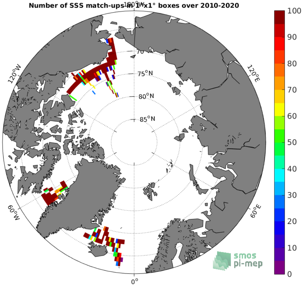
Figure 4: Number of SSS match-ups between TSG (SAMOS) SSS and the SMOS SSS L3 v317 - 10 Days - 25 km (CATDS-CPDC) SSS product for the Arctic Ocean Pi-MEP region over 1°x1° boxes and for the full satellite product period.
