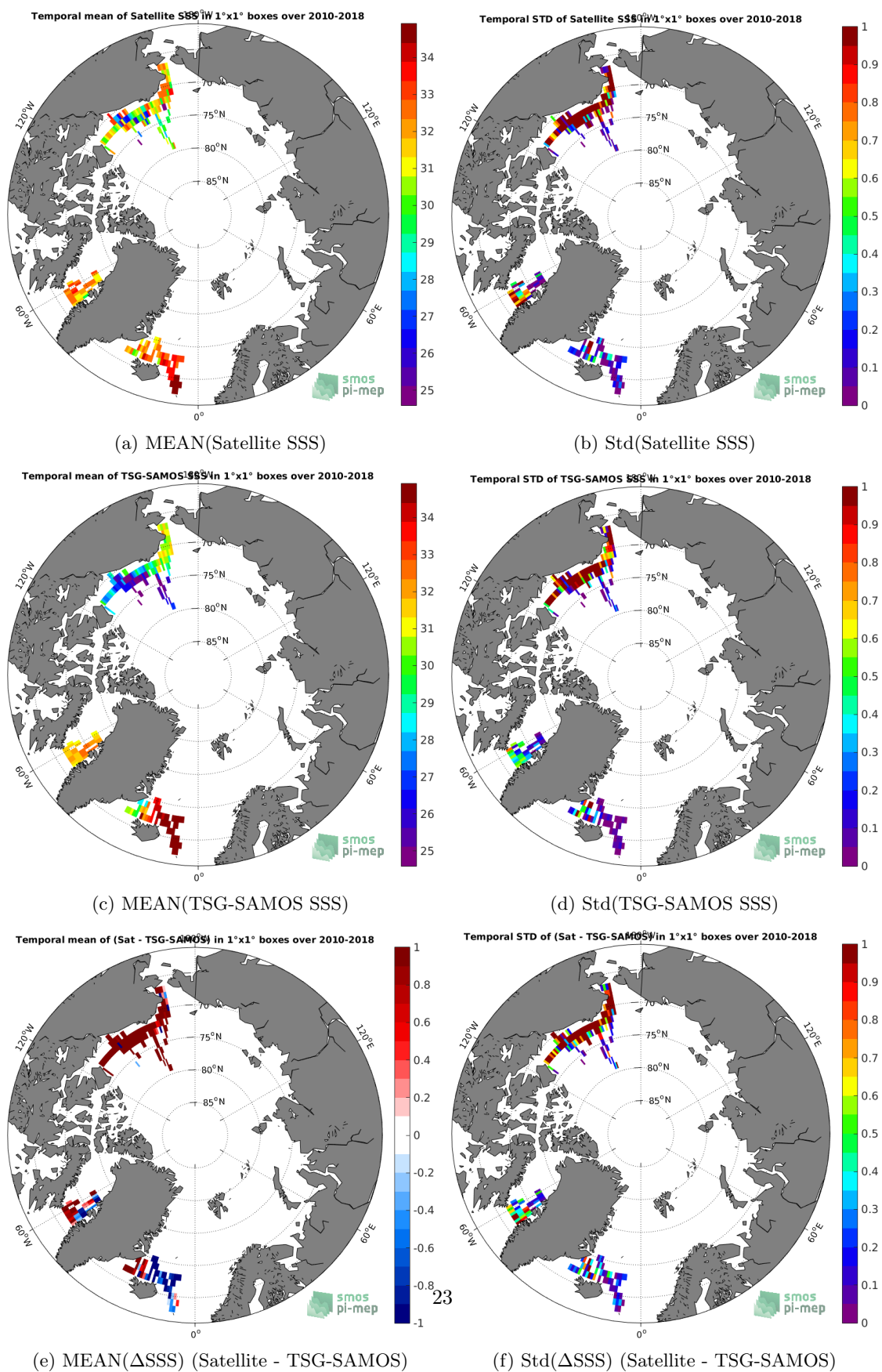
Figure 6: Temporal mean (left) and Std (right) of SSS from SMOS L3 v317 - 10 Days - 25 km (CATDS-CPDC) (top), TSG-SAMOS (middle), and of \Delta SSS (Satellite - TSG-SAMOS). Only match-up pairs are used to generate these maps.
