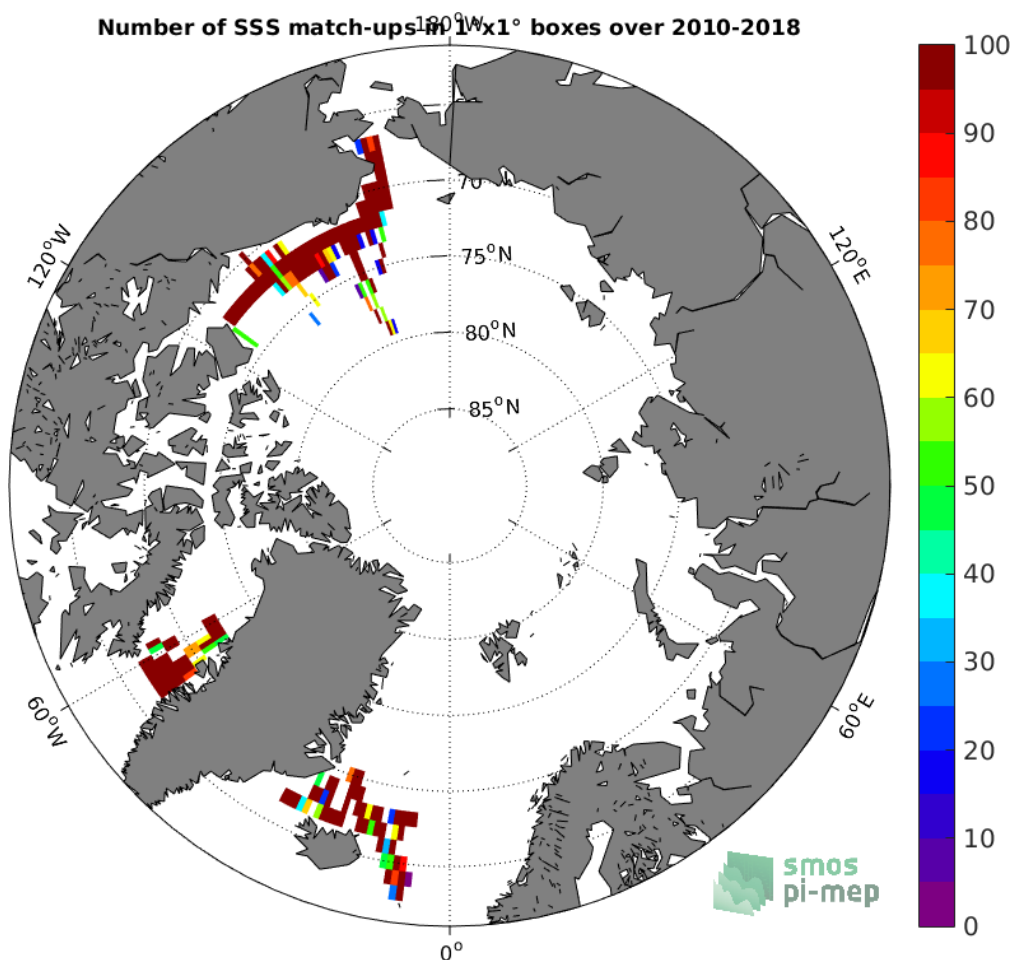
Figure 4: Number of SSS match-ups between TSG-SAMOS SSS and the SMOS L3 v317 - 10 Days - 25 km (CATDS-CPDC) SSS product for the Arctic Ocean Pi-MEP region over 1°x1° boxes and for the full satellite product period.
