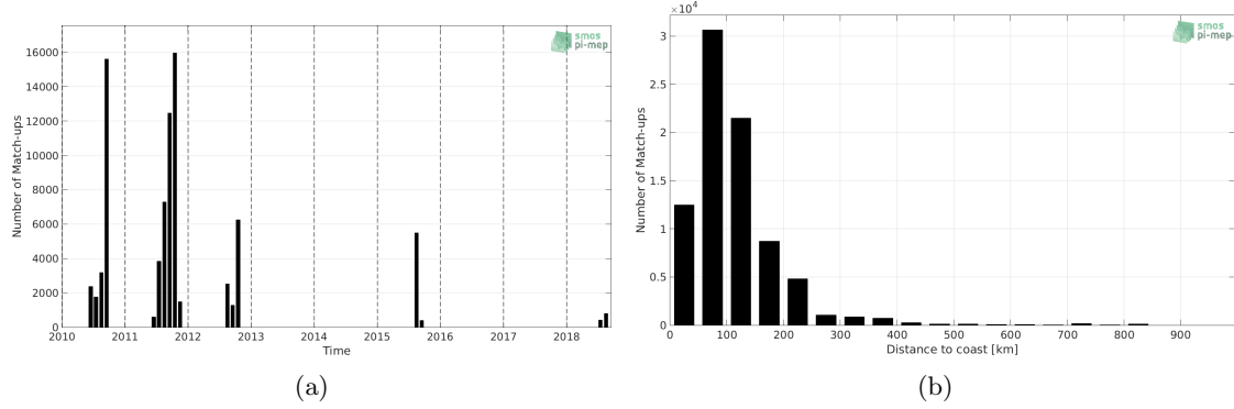
Figure 1: Number of match-ups between TSG-SAMOS and SMOS L3 v317 - 10 Days - 25 km (CATDS-CPDC) SSS as a function of time (a) and as function of the distance to coast (b) over the Arctic Ocean Pi-MEP region and for the full satellite product period.
