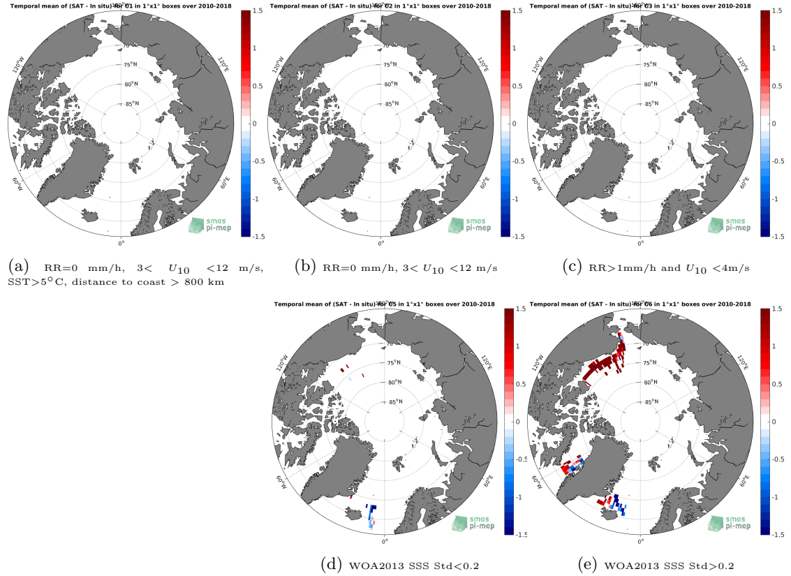
Figure 12: Temporal mean gridded over spatial boxes of size 1^{\circ}\times 1^{\circ} of \Delta\text{SSS} (SMOS L3 v317 - 10 Days - 25 km (CATDS-CPDC) - TSG-SAMOS) for 5 different subdatasets corresponding to: \text{RR}=0 mm/h, 3 < U_{10} < 12 m/s, \text{SST} > 5^{\circ}\text{C} , distance to coast > 800 km (a), \text{RR}=0 mm/h, 3 < U_{10} < 12 m/s (b), \text{RR} > 1 mm/h and U_{10} < 4 m/s (c), WOA2013 SSS Std < 0.2 (d), WOA2013 SSS Std > 0.2 (e).
