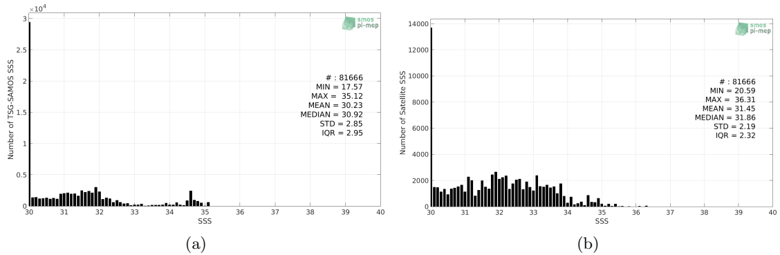
Figure 2: Histograms of SSS from TSG-SAMOS (a) and SMOS L3 v317 - 10 Days - 25 km (CATDS-CPDC) (b) considering all match-up pairs per bins of 0.1 over the Arctic Ocean Pi-MEP region and for the full satellite product period.
