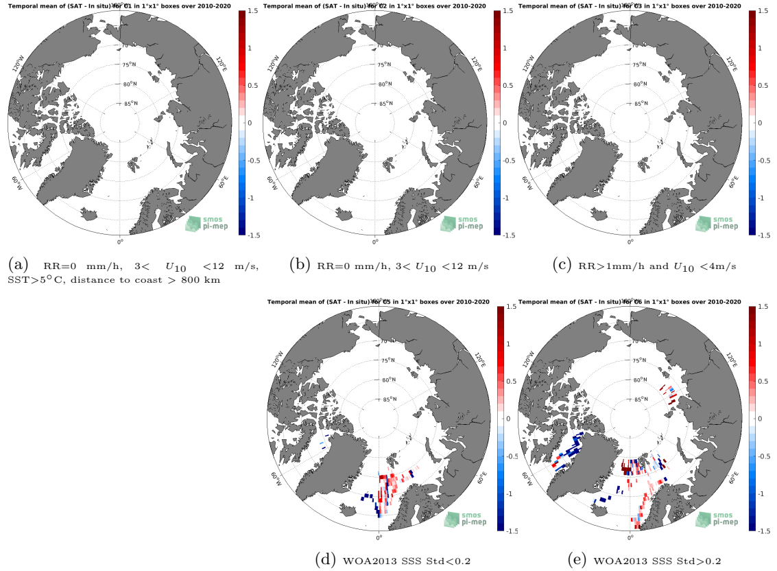
Figure 12: Temporal mean gridded over spatial boxes of size 1^{\circ} \times 1^{\circ} of \Delta\text{SSS} (SMOS SSS L3 v317 - 10 Days - 25 km (CATDS-CPDC) - TSG (Polarstern)) for 5 different subdatasets corresponding to: RR=0 mm/h, 3 < U_{10} < 12 m/s, SST > 5^{\circ}\text{C} , distance to coast > 800 km (a), RR=0 mm/h, 3 < U_{10} < 12 m/s (b), RR > 1 mm/h and U_{10} < 4 m/s (c), WOA2013 SSS Std < 0.2 (d), WOA2013 SSS Std > 0.2 (e).
