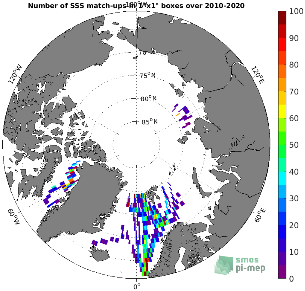
Figure 4: Number of SSS match-ups between TSG (Polarstern) SSS and the SMOS SSS L3 v317 - 10 Days - 25 km (CATDS-CPDC) SSS product for the Arctic Ocean Pi-MEP region over 1^\circ \times 1^\circ boxes and for the full satellite product period.
