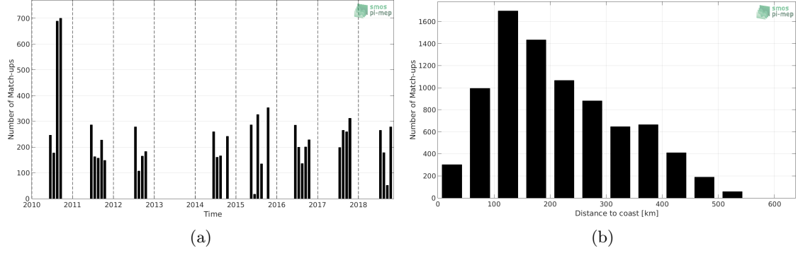
Figure 1: Number of match-ups between TSG (Polarstern) and SMOS SSS L3 v317 - 10 Days - 25 km (CATDS-CPDC) SSS as a function of time (a) and as function of the distance to coast (b) over the Arctic Ocean Pi-MEP region and for the full satellite product period.
