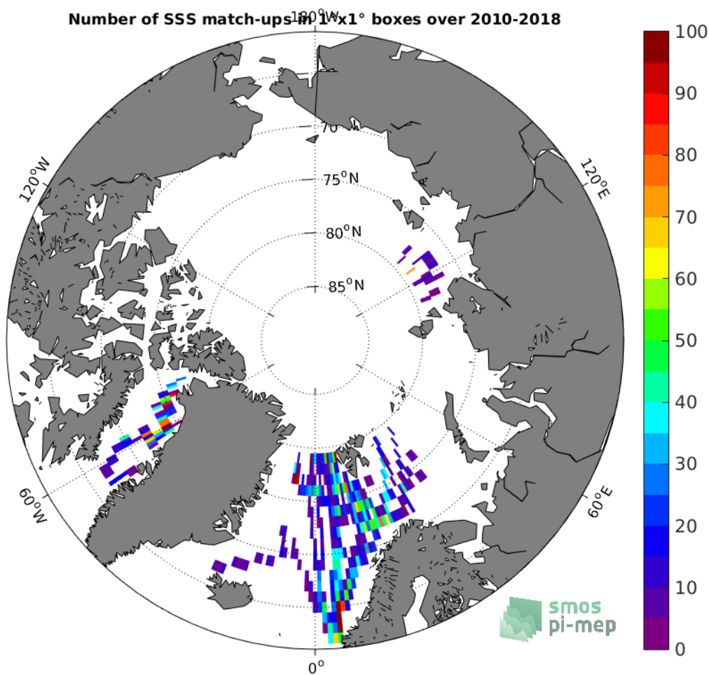
Figure 4: Number of SSS match-ups between TSG-POLARSTERN SSS and the SMOS-L3-CATDS-CPDC-V317-10DAYS-25KM SSS product for the Arctic Ocean Pi-MEP region over 1^\circ \times 1^\circ boxes and for the full satellite product period.
