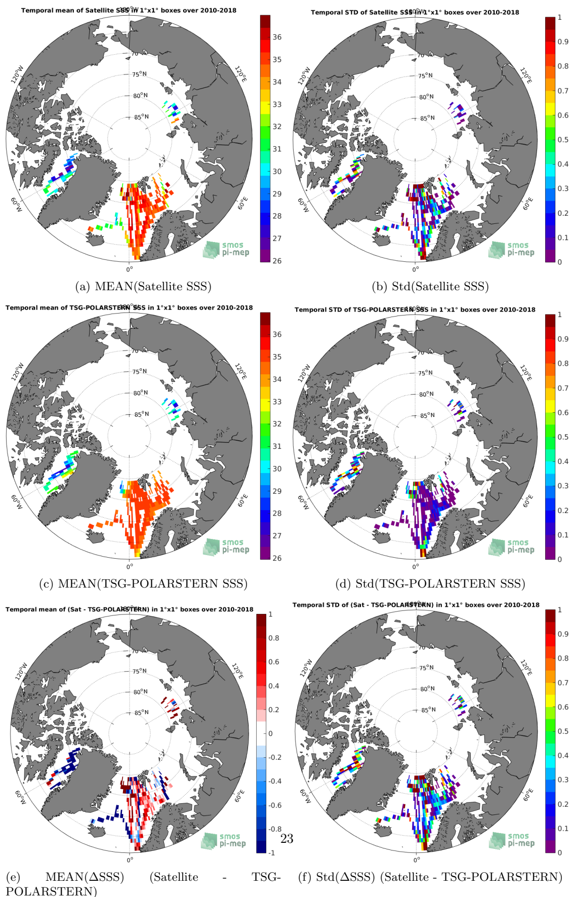
Figure 6: Temporal mean (left) and Std (right) of SSS from SMOS-L3-CATDS-CPDC-V317-10DAYS-25KM (top), TSG-POLARSTERN (middle), and of \Delta SSS (Satellite - TSG-POLARSTERN). Only match-up pairs are used to generate these maps.
