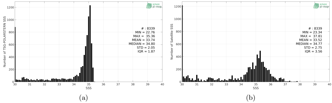
Figure 2: Histograms of SSS from TSG-POLARSTERN (a) and SMOS-L3-CATDS-CPDC-V317-10DAYS-25KM (b) considering all match-up pairs per bins of 0.1 over the Arctic Ocean Pi-MEP region and for the full satellite product period.
