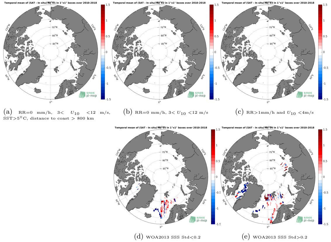
Figure 12: Temporal mean gridded over spatial boxes of size 1^\circ \times 1^\circ of \Delta SSS (SMOS-L3-CATDS-CPDC-V317-10DAYS-25KM - TSG-POLARSTERN) for 5 different subdatasets corresponding to: RR=0 mm/h, 3 < U_{10} < 12 m/s, SST > 5^\circ C , distance to coast > 800 km (a), RR=0 mm/h, 3 < U_{10} < 12 m/s (b), RR > 1 mm/h and U_{10} < 4 m/s (c), WOA2013 SSS Std < 0.2 (d), WOA2013 SSS Std > 0.2 (e).
