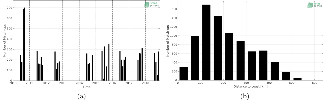
Figure 1: Number of match-ups between TSG-POLARSTERN and SMOS-L3-CATDS-CPDC-V317-10DAYS-25KM SSS as a function of time (a) and as function of the distance to coast (b) over the Arctic Ocean Pi-MEP region and for the full satellite product period.
