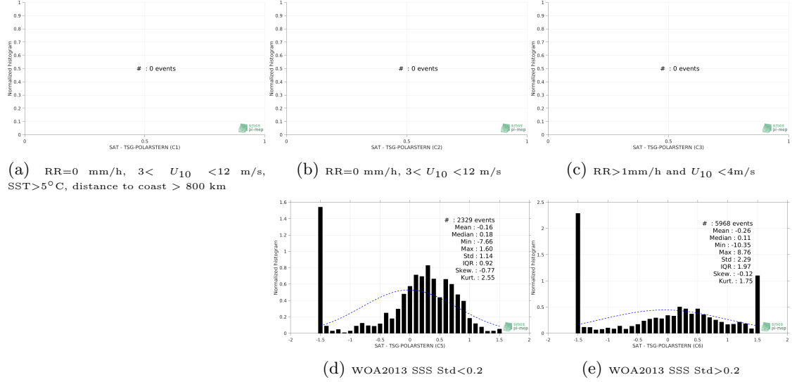
Figure 13: Normalized histogram of \Delta\text{SSS} (SMOS-L3-CATDS-CPDC-V317-10DAYS-25KM - TSG-POLARSTERN) for 5 different subdatasets corresponding to: RR=0 mm/h, 3 < U_{10} < 12 m/s, SST > 5^\circ\text{C} , distance to coast > 800 km (a), RR=0 mm/h, 3 < U_{10} < 12 m/s (b), RR > 1 mm/h and U_{10} < 4 m/s (c), WOA2013 SSS Std < 0.2 (d), WOA2013 SSS Std > 0.2 (e).
