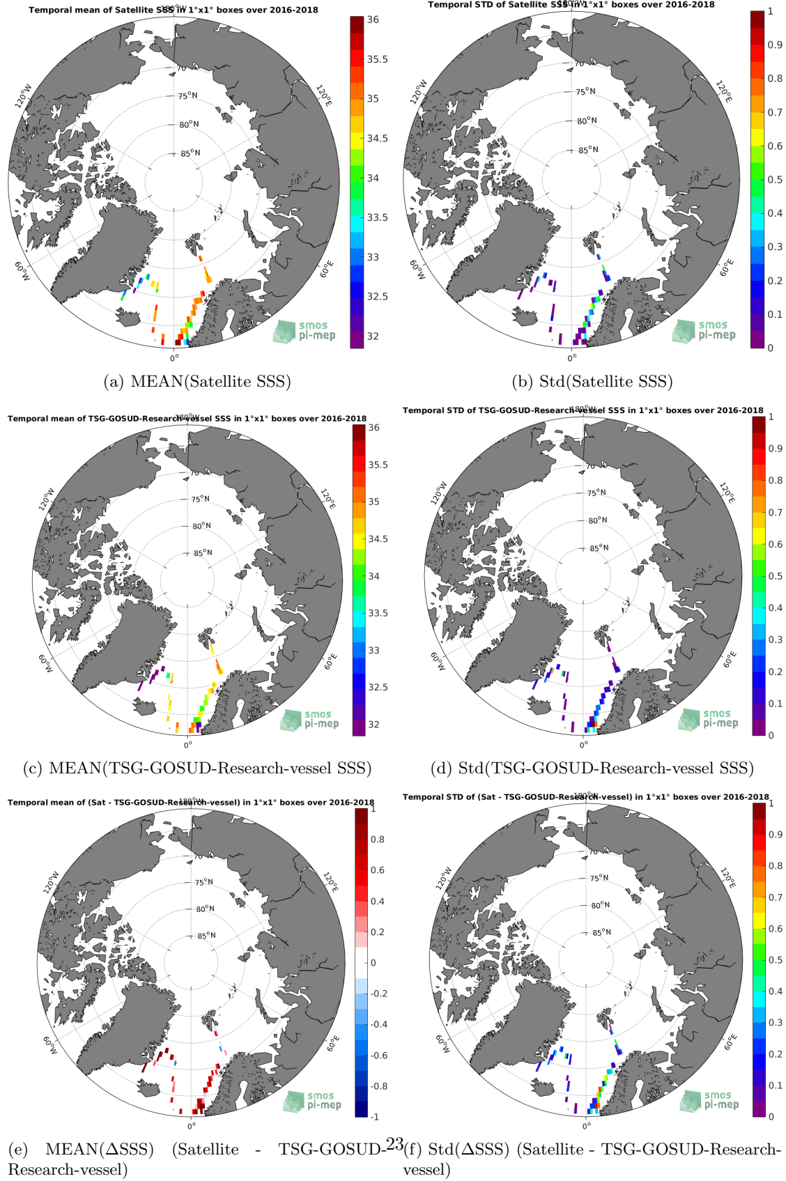
Figure 6: Temporal mean (left) and Std (right) of SSS from SMOS L3 v317 - 10 Days - 25 km (CATDS-CPDC) (top), TSG-GOSUD-Research-vessel (middle), and of \Delta SSS (Satellite - TSG-GOSUD-Research-vessel). Only match-up pairs are used to generate these maps.
