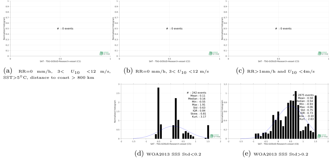
Figure 13: Normalized histogram of \Delta\text{SSS} (SMOS L3 v317 - 10 Days - 25 km (CATDS-CPDC) - TSG-GOSUD-Research-vessel) for 5 different subdatasets corresponding to: RR=0 mm/h, 3 < U_{10} < 12 m/s, SST >5^{\circ}\text{C} , distance to coast > 800 km (a), RR=0 mm/h, 3 < U_{10} < 12 m/s (b), RR>1\text{mm/h} and U_{10} < 4\text{m/s} (c), WOA2013 SSS Std <0.2 (d), WOA2013 SSS Std >0.2 (e).
