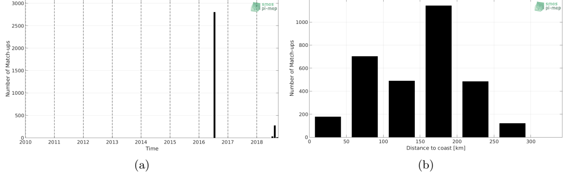
Figure 1: Number of match-ups between TSG-GOSUD-Research-vessel and SMOS L3 v317 - 10 Days - 25 km (CATDS-CPDC) SSS as a function of time (a) and as function of the distance to coast (b) over the Arctic Ocean Pi-MEP region and for the full satellite product period.
