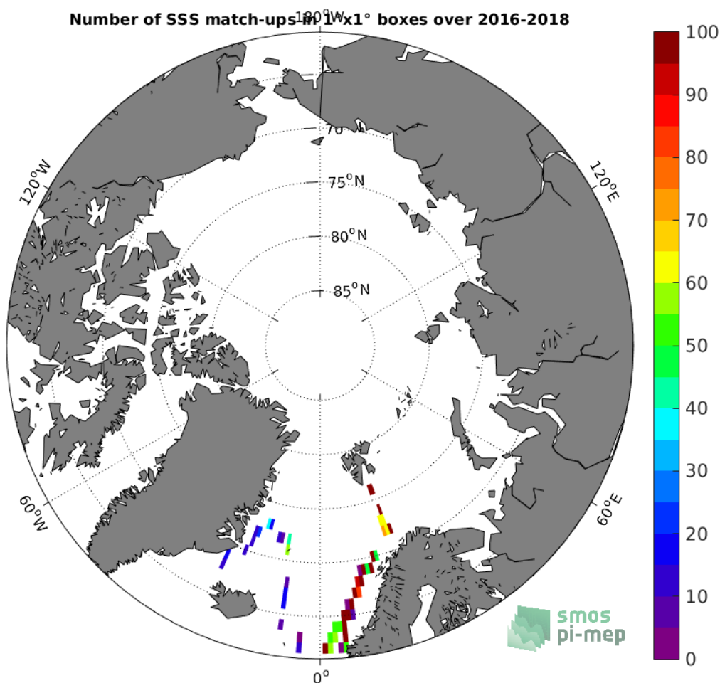
Figure 4: Number of SSS match-ups between TSG-GOSUD-Research-vessel SSS and the SMOS-L3-CATDS-CPDC-V317-10DAYS-25KM SSS product for the Arctic Ocean Pi-MEP region over 1^\circ \times 1^\circ boxes and for the full satellite product period.
