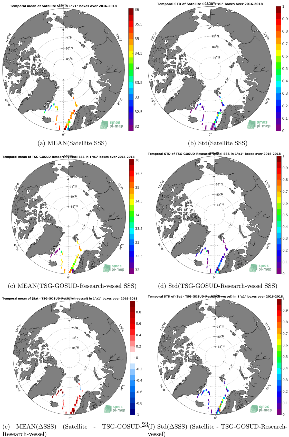
Figure 6: Temporal mean (left) and Std (right) of SSS from SMOS-L3-CATDS-CPDC-V317-10DAYS-25KM (top), TSG-GOSUD-Research-vessel (middle), and of \Delta SSS (Satellite - TSG-GOSUD-Research-vessel). Only match-up pairs are used to generate these maps.
