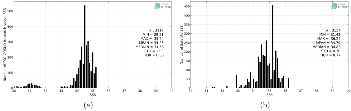
Figure 2: Histograms of SSS from TSG-GOSUD-Research-vessel (a) and SMOS-L3-CATDS-CPDC-V317-10DAYS-25KM (b) considering all match-up pairs per bins of 0.1 over the Arctic Ocean Pi-MEP region and for the full satellite product period.
