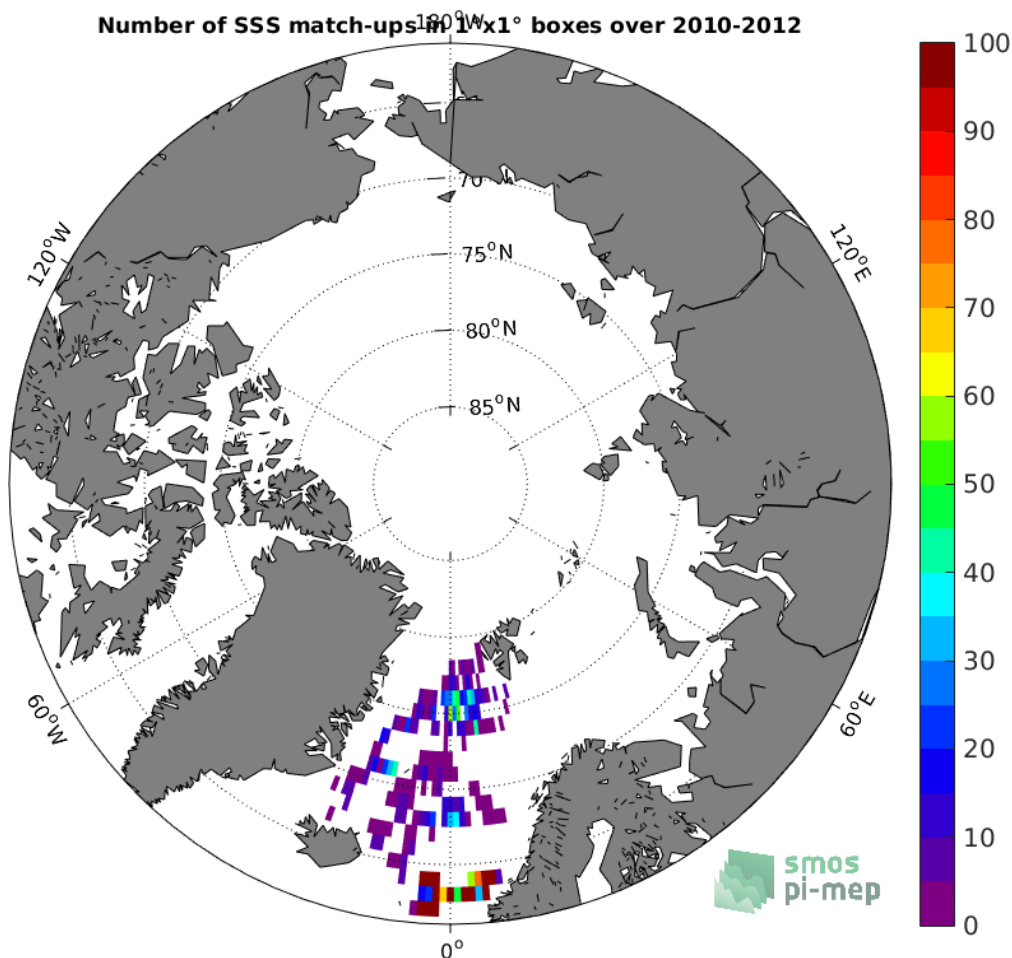
Figure 3: Number of SSS match-ups between Surface drifters SSS and the SMOS SSS L3 v317 - 10 Days - 25 km (CATDS-CPDC) SSS product for the Arctic Ocean Pi-MEP region over 1°x1° boxes and for the full satellite product period.
