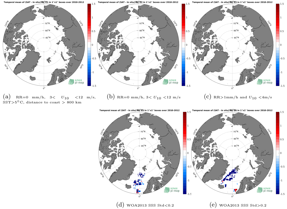
Figure 11: Temporal mean gridded over spatial boxes of size 1^{\circ}\times 1^{\circ} of \Delta\text{SSS} (SMOS L3 v317 - 10 Days - 25 km (CATDS-CPDC) - Surface drifters) for 5 different subdatasets corresponding to: \text{RR}=0 mm/h, 3 < U_{10} < 12 m/s, \text{SST} > 5^{\circ}\text{C} , distance to coast > 800 km (a), \text{RR}=0 mm/h, 3 < U_{10} < 12 m/s (b), \text{RR} > 1 mm/h and U_{10} < 4 m/s (c), WOA2013 SSS Std < 0.2 (d), WOA2013 SSS Std > 0.2 (e).
