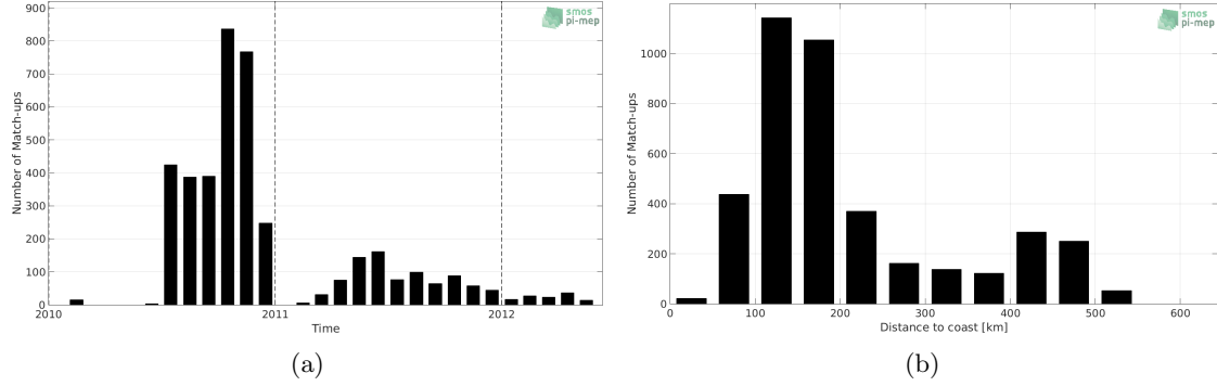
Figure 1: Number of match-ups between Surface drifters and SMOS L3 v317 - 10 Days - 25 km (CATDS-CPDC) SSS as a function of time (a) and as function of the distance to coast (b) over the Arctic Ocean Pi-MEP region and for the full satellite product period.
