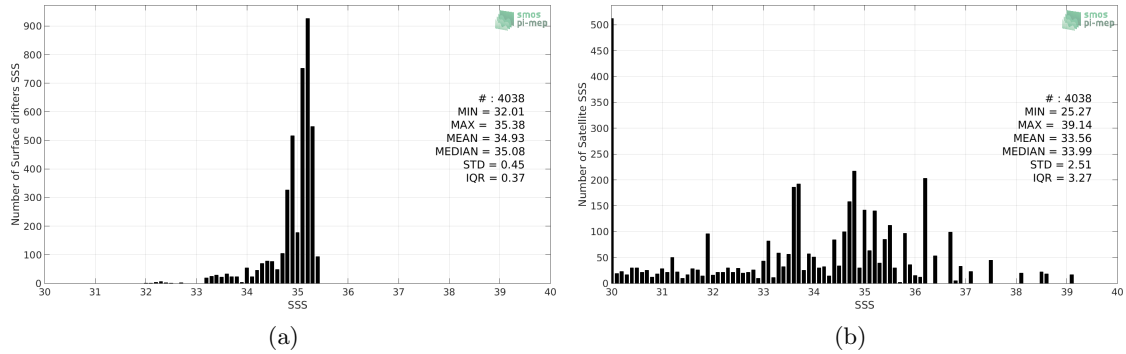
Figure 2: Histograms of SSS from Surface drifters (a) and SMOS L3 v317 - 10 Days - 25 km (CATDS-CPDC) (b) considering all match-up pairs per bins of 0.1 over the Arctic Ocean Pi-MEP region and for the full satellite product period.
