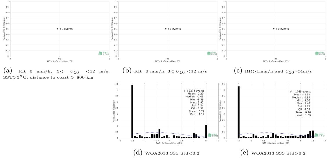
Figure 12: Normalized histogram of \Delta\text{SSS} (SMOS L3 v317 - 10 Days - 25 km (CATDS-CPDC) - Surface drifters) for 5 different subdatasets corresponding to: RR=0 mm/h, 3 < U_{10} < 12 m/s, SST > 5^{\circ}\text{C} , distance to coast > 800 km (a), RR=0 mm/h, 3 < U_{10} < 12 m/s (b), RR > 1 mm/h and U_{10} < 4 m/s (c), WOA2013 SSS Std < 0.2 (d), WOA2013 SSS Std > 0.2 (e).
