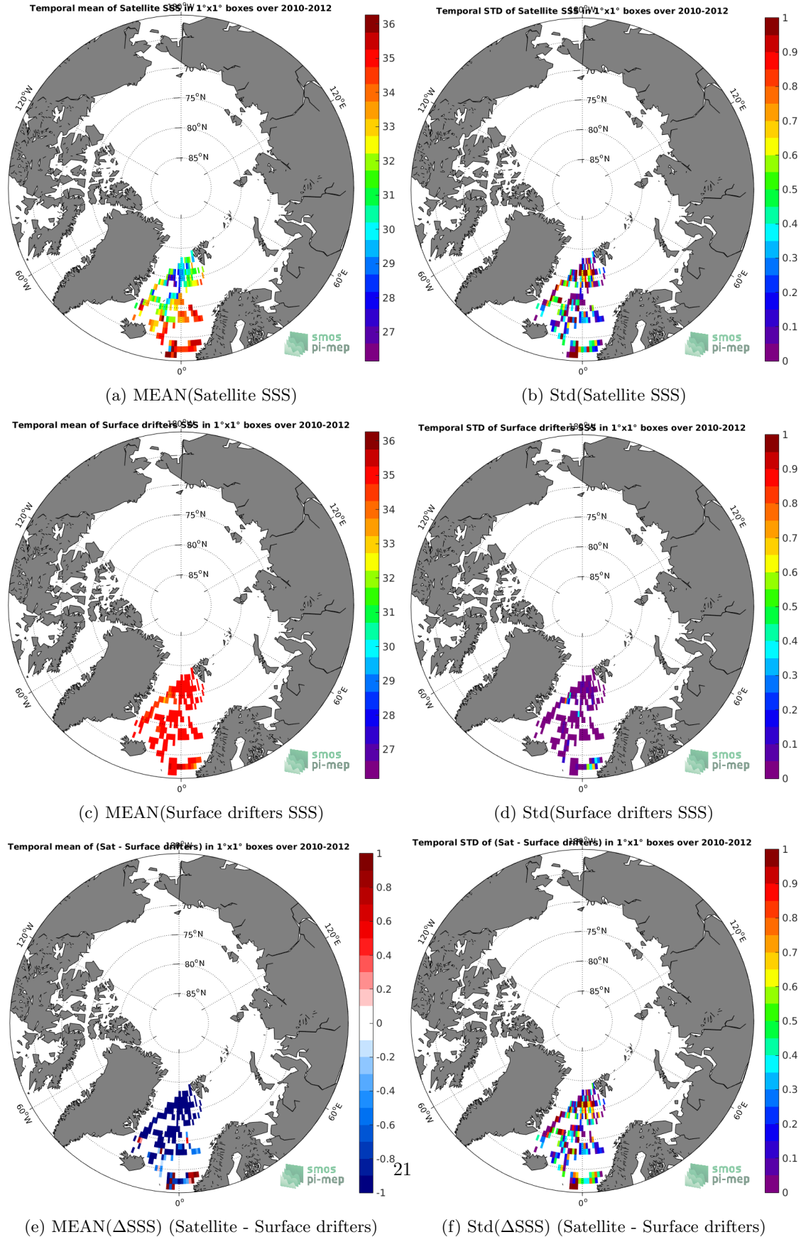
Figure 5: Temporal mean (left) and Std (right) of SSS from SMOS L3 v317 - 10 Days - 25 km (CATDS-CPDC) (top), Surface drifters (middle), and of \Delta SSS (Satellite - Surface drifters). Only match-up pairs are used to generate these maps.
