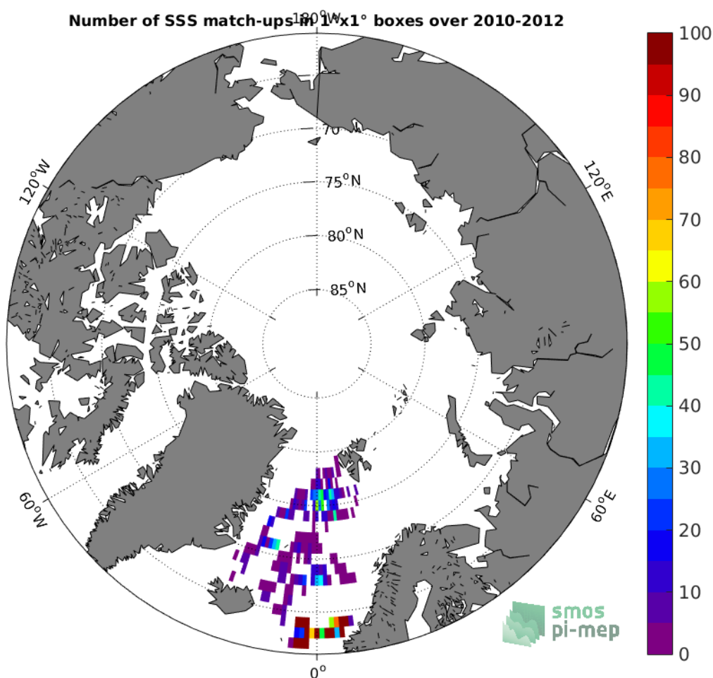
Figure 3: Number of SSS match-ups between Surface drifters SSS and the SMOS L3 v317 - 10 Days - 25 km (CATDS-CPDC) SSS product for the Arctic Ocean Pi-MEP region over 1°x1° boxes and for the full satellite product period.
