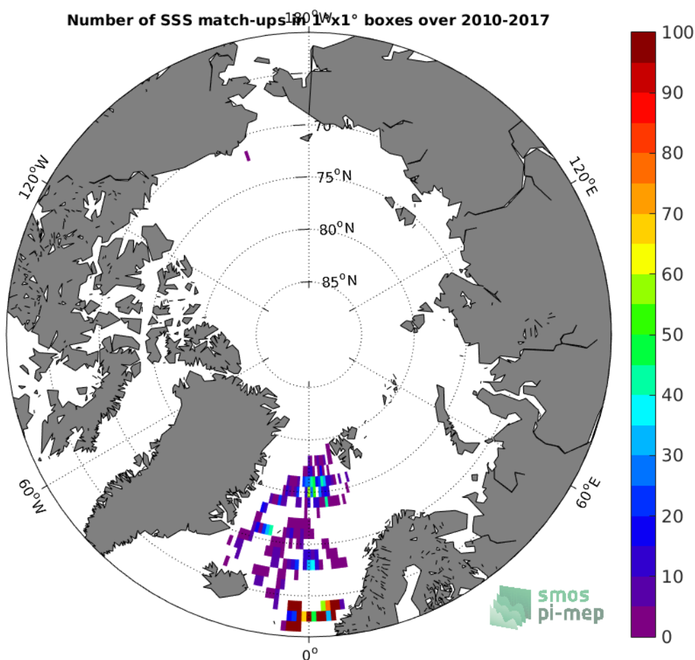
Figure 3: Number of SSS match-ups between Surface drifters SSS and the SMOS-L3-CATDS-CPDC-V317-10DAYS-25KM SSS product for the Arctic Ocean Pi-MEP region over 1^\circ \times 1^\circ boxes and for the full satellite product period.
