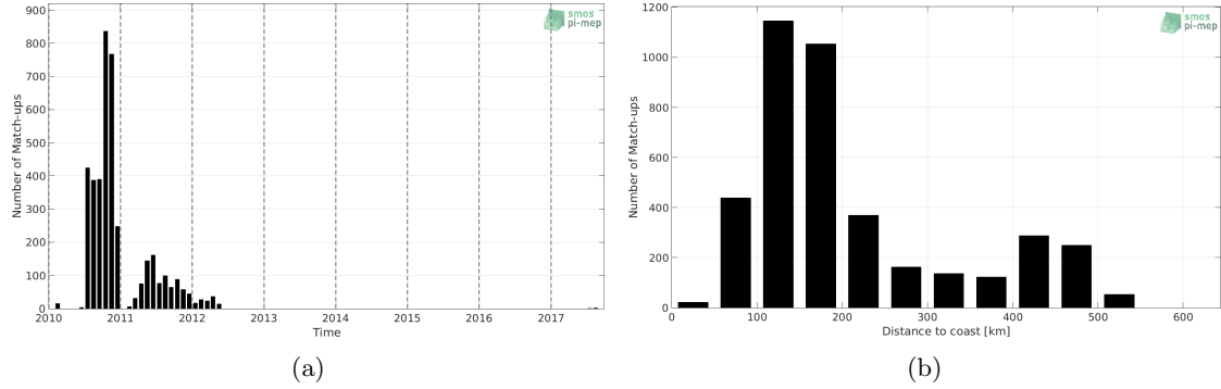
Figure 1: Number of match-ups between Surface drifters and SMOS-L3-CATDS-CPDC-V317-10DAYS-25KM SSS as a function of time (a) and as function of the distance to coast (b) over the Arctic Ocean Pi-MEP region and for the full satellite product period.
