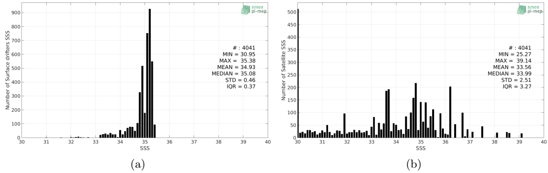
Figure 2: Histograms of SSS from Surface drifters (a) and SMOS-L3-CATDS-CPDC-V317-10DAYS-25KM (b) considering all match-up pairs per bins of 0.1 over the Arctic Ocean Pi-MEP region and for the full satellite product period.
