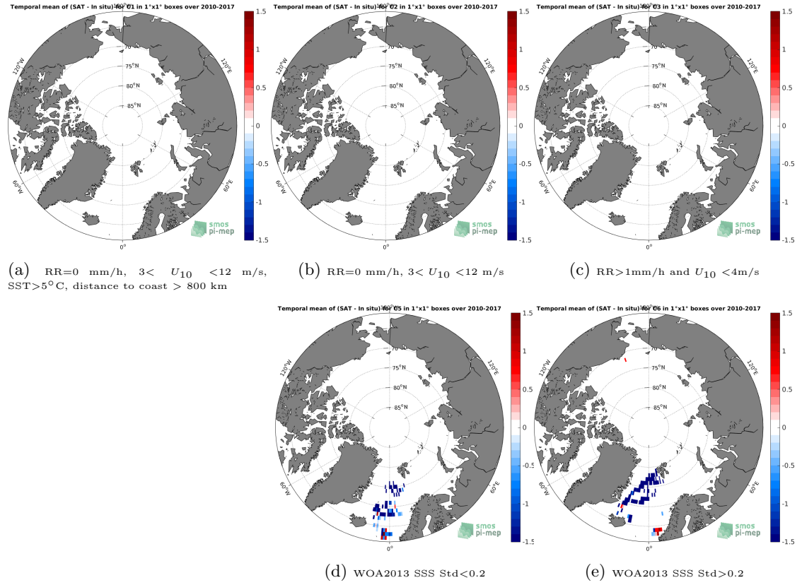
Figure 11: Temporal mean gridded over spatial boxes of size 1^\circ \times 1^\circ of \Delta SSS (SMOS-L3-CATDS-CPDC-V317-10DAYS-25KM - Surface drifters) for 5 different subdatasets corresponding to: RR=0 mm/h, 3 < U_{10} < 12 m/s, SST > 5^\circ\text{C} , distance to coast > 800 km (a), RR=0 mm/h, 3 < U_{10} < 12 m/s (b), RR > 1 mm/h and U_{10} < 4 m/s (c), WOA2013 SSS Std < 0.2 (d), WOA2013 SSS Std > 0.2 (e).
