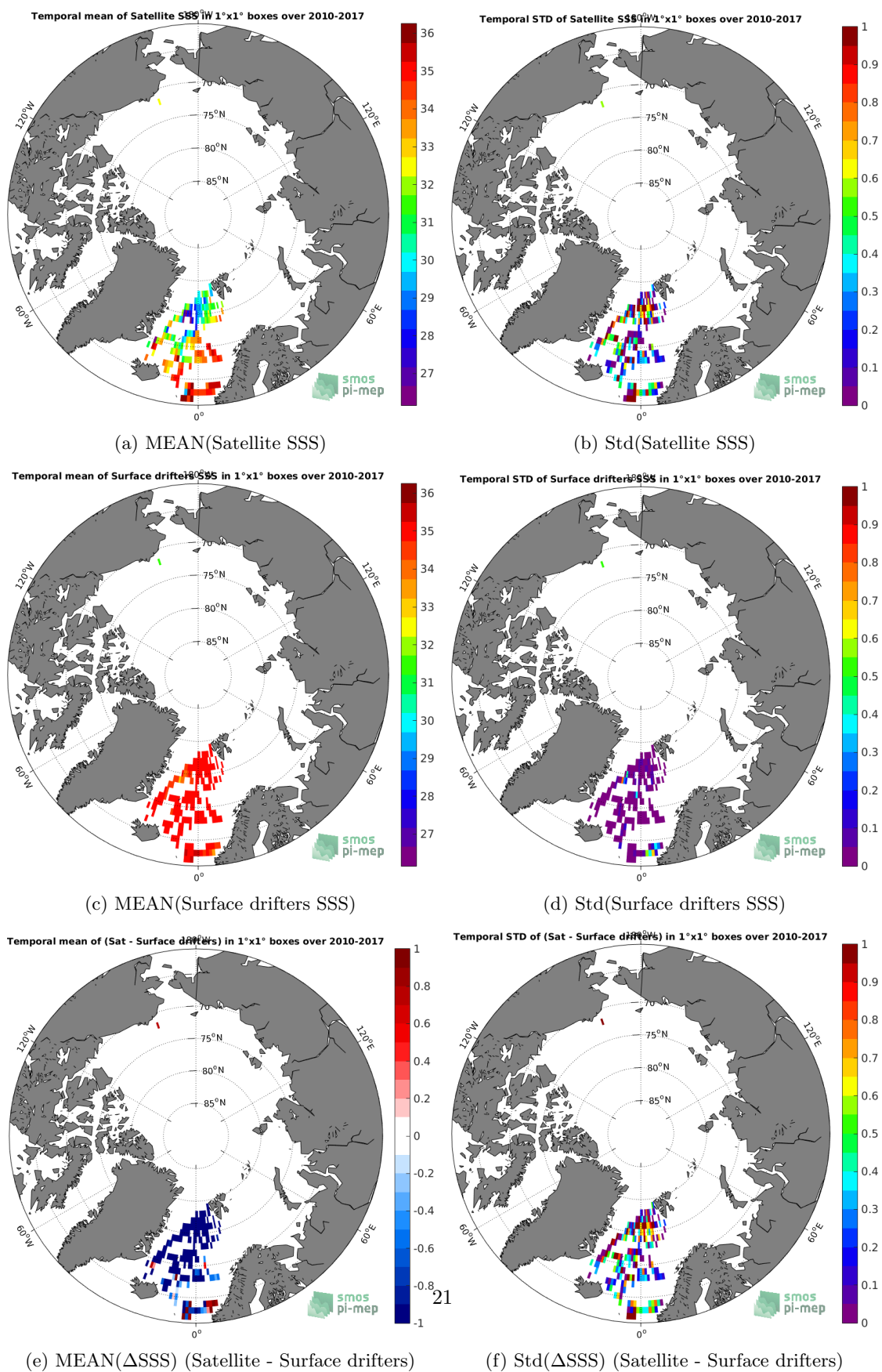
Figure 5: Temporal mean (left) and Std (right) of SSS from SMOS-L3-CATDS-CPDC-V317-10DAYS-25KM (top), Surface drifters (middle), and of \Delta SSS (Satellite - Surface drifters). Only match-up pairs are used to generate these maps.
