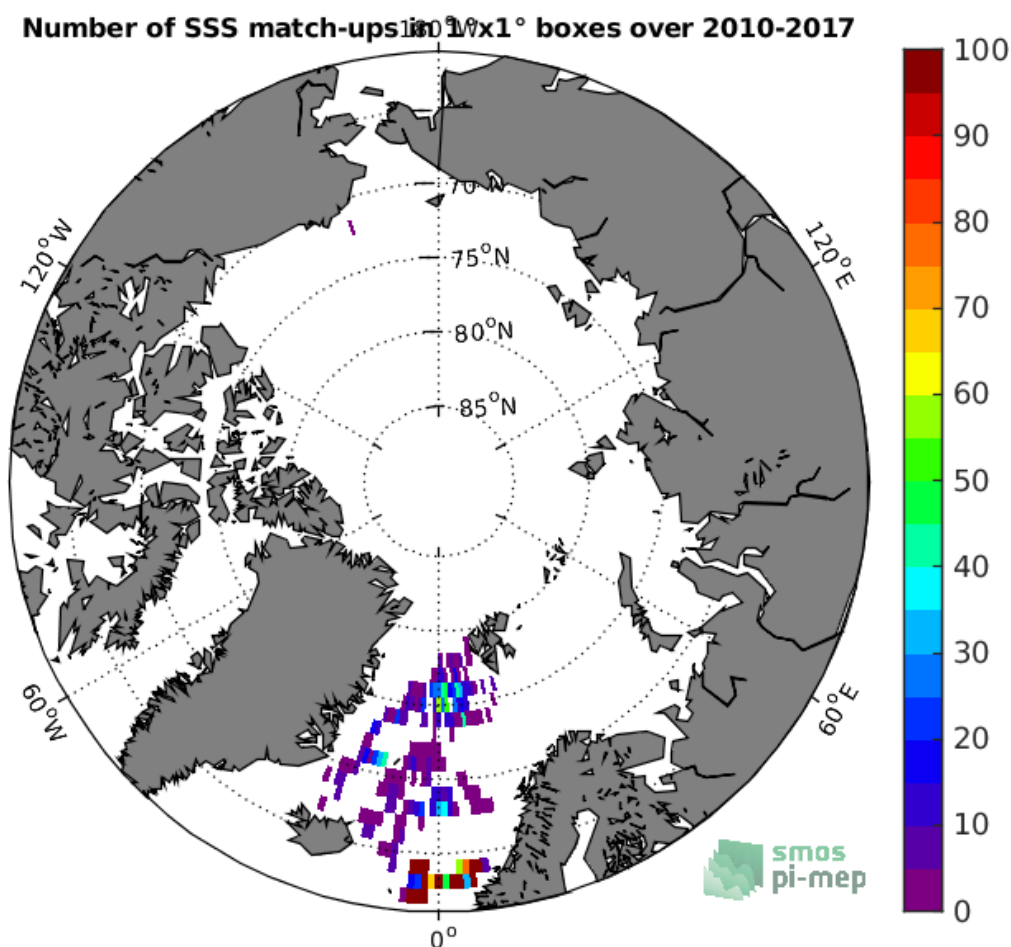
Figure 3: Number of SSS match-ups between Surface drifters SSS and the SMOS-L3-CATDS-CPDC-V317-10DAYS-25KM SSS product for the Arctic Ocean Pi-MEP region over 1°x1° boxes and for the full satellite product period.
