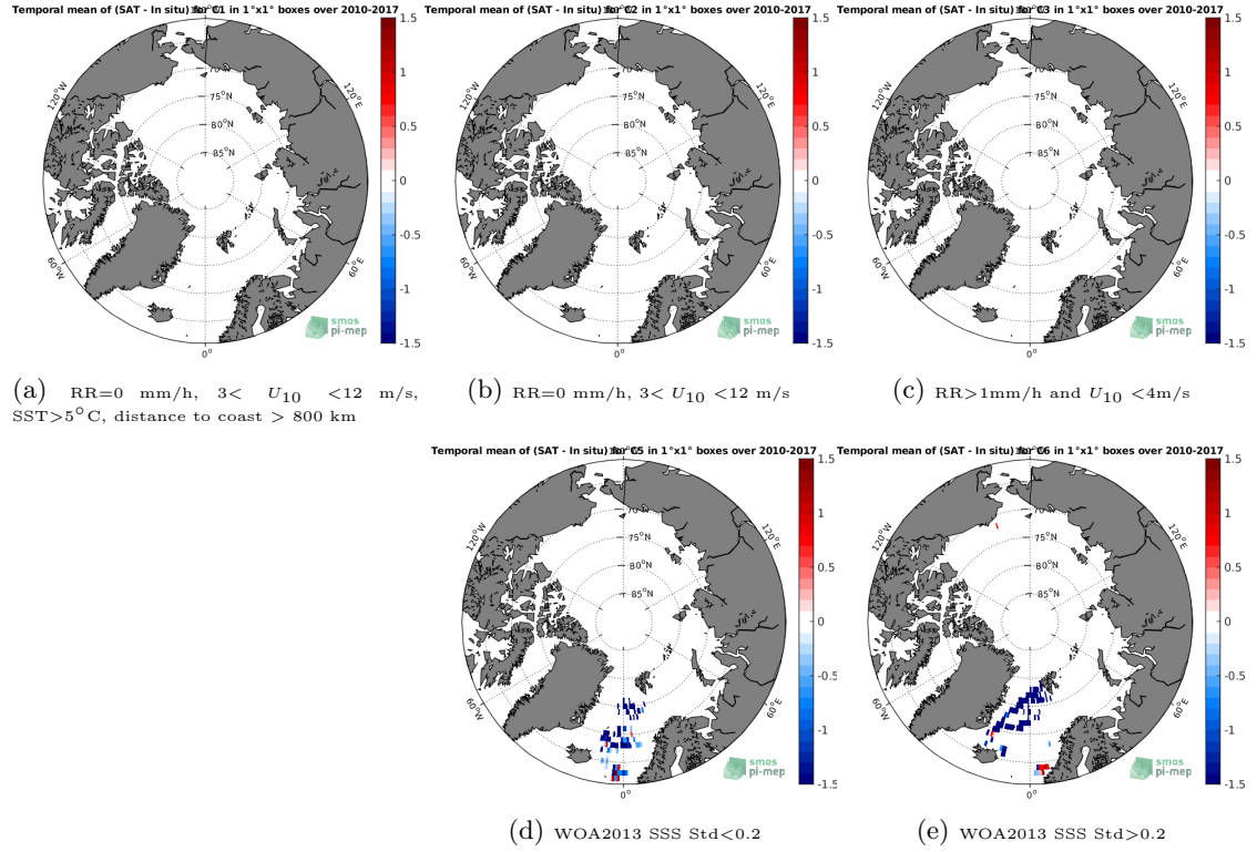
Figure 11: Temporal mean gridded over spatial boxes of size 1^\circ \times 1^\circ of \Delta SSS (SMOS-L3-CATDS-CPDC-V317-10DAYS-25KM - Surface drifters) for 5 different subdatasets corresponding to: RR=0 mm/h, 3 < U_{10} < 12 m/s, SST > 5^\circ C , distance to coast > 800 km (a), RR=0 mm/h, 3 < U_{10} < 12 m/s (b), RR > 1 mm/h and U_{10} < 4 m/s (c), WOA2013 SSS Std < 0.2 (d), WOA2013 SSS Std > 0.2 (e).
