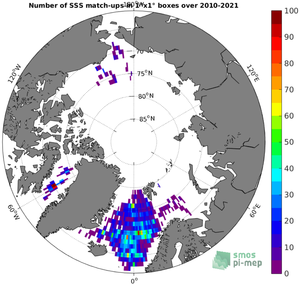
Figure 4: Number of SSS match-ups between Argo SSS and the SMOS SSS L3 v317 - 10 Days - 25 km (CATDS-CPDC) SSS product for the Arctic Ocean Pi-MEP region over 1^\circ \times 1^\circ boxes and for the full satellite product period.
