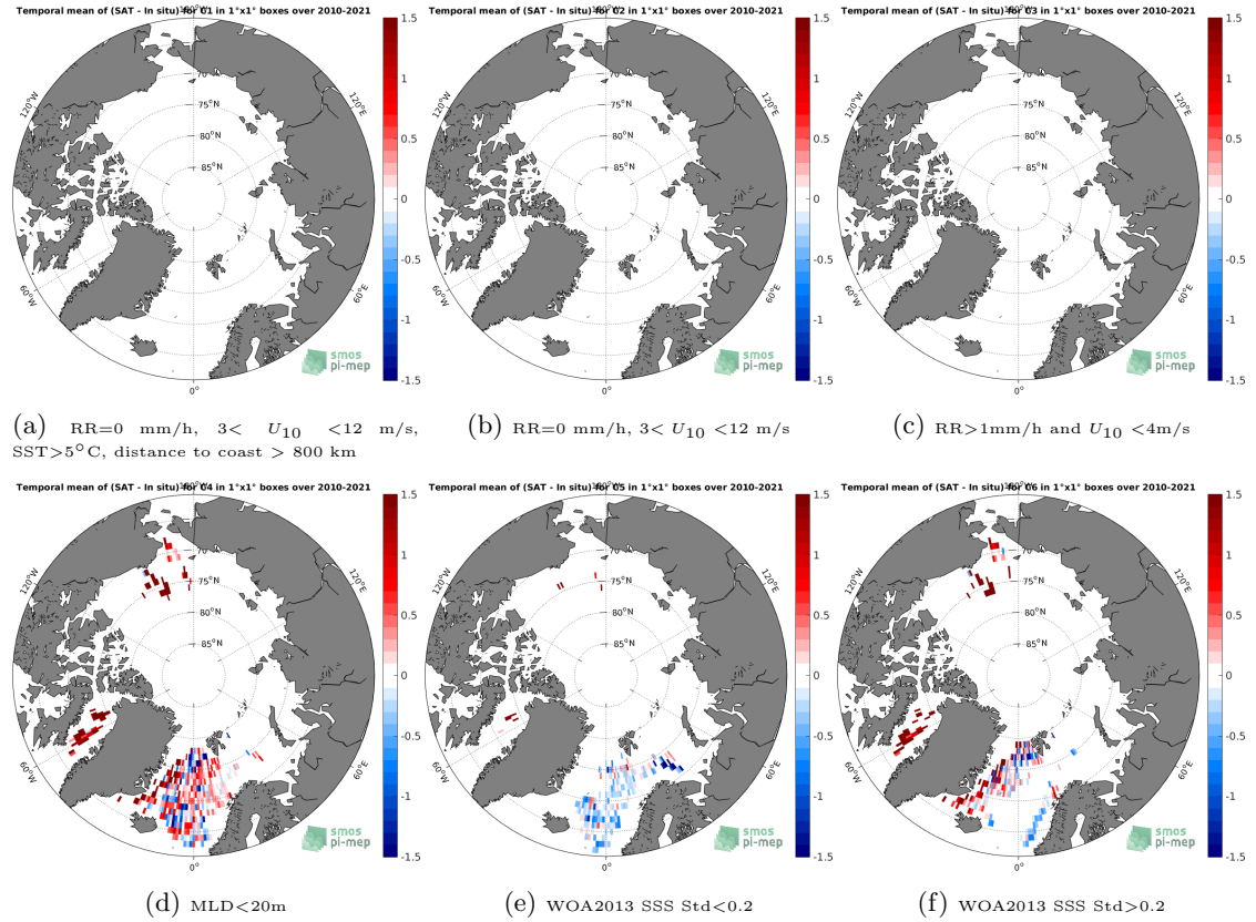
Figure 12: Temporal mean gridded over spatial boxes of size 1^{\circ} \times 1^{\circ} of \Delta\text{SSS} (SMOS SSS L3 v317 - 10 Days - 25 km (CATDS-CPDC) - Argo) for 6 different subdatasets corresponding to: RR=0 mm/h, 3 < U_{10} < 12 m/s, SST > 5^{\circ}\text{C} , distance to coast > 800 km (a), RR=0 mm/h, 3 < U_{10} < 12 m/s (b), RR > 1 mm/h and U_{10} < 4 m/s (c), MLD < 20 m (d), WOA2013 SSS Std < 0.2 (e), WOA2013 SSS Std > 0.2 (f).
