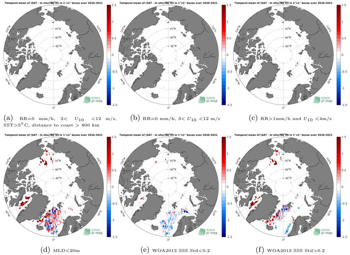
Figure 12: Temporal mean gridded over spatial boxes of size 1^{\circ}\times 1^{\circ} of \Delta\text{SSS} (SMOS SSS L3 v317 - 10 Days - 25 km (CATDS-CPDC) - Argo) for 6 different subdatasets corresponding to: RR=0 mm/h, 3 < U_{10} < 12 m/s, SST > 5^{\circ}\text{C} , distance to coast > 800 km (a), RR=0 mm/h, 3 < U_{10} < 12 m/s (b), RR > 1 mm/h and U_{10} < 4 m/s (c), MLD < 20\text{m} (d), WOA2013 SSS Std < 0.2 (e), WOA2013 SSS Std > 0.2 (f).
