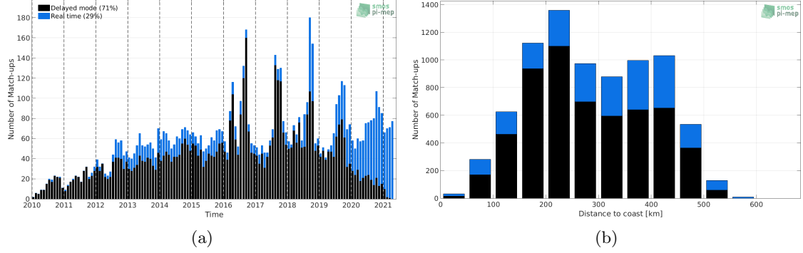
Figure 1: Number of match-ups between Argo and SMOS SSS L3 v317 - 10 Days - 25 km (CATDS-CPDC) SSS as a function of time (a) and as function of the distance to coast (b) over the Arctic Ocean Pi-MEP region and for the full satellite product period.
