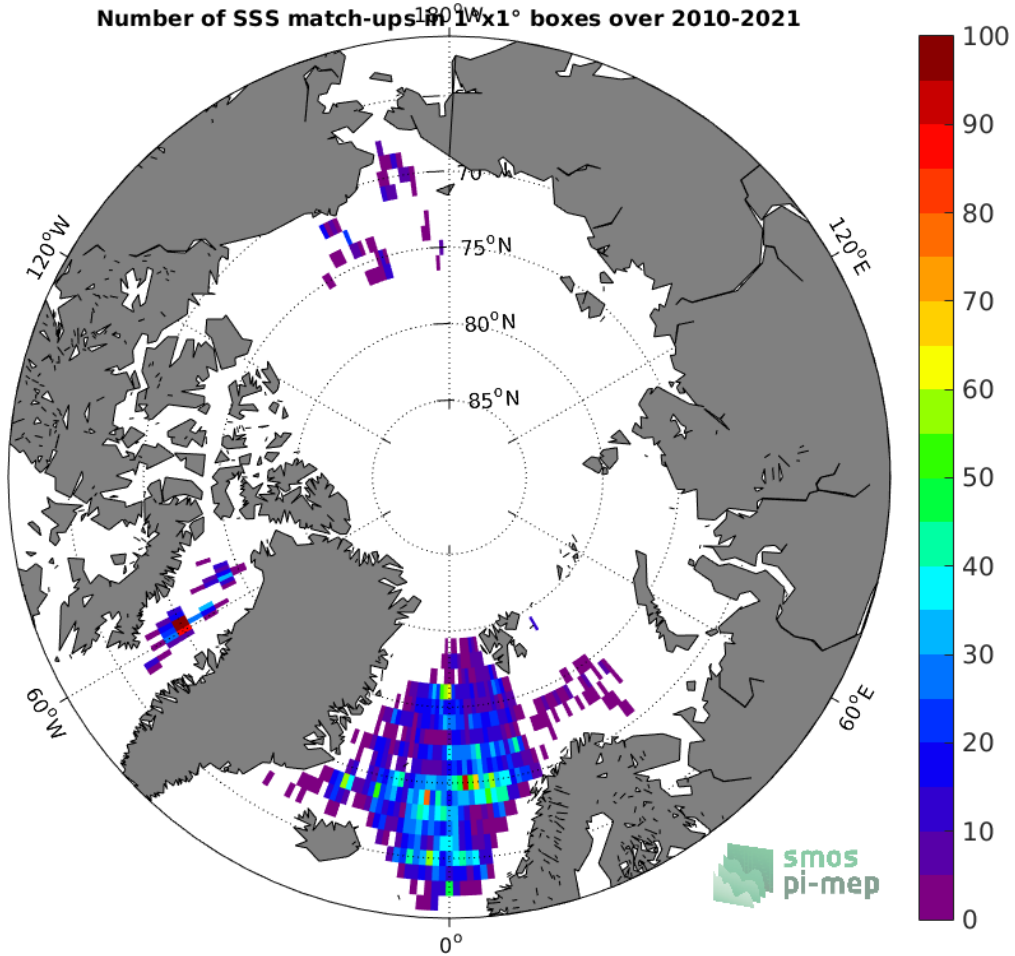
Figure 4: Number of SSS match-ups between Argo SSS and the SMOS SSS L3 v317 - 10 Days - 25 km (CATDS-CPDC) SSS product for the Arctic Ocean Pi-MEP region over 1°x1° boxes and for the full satellite product period.
