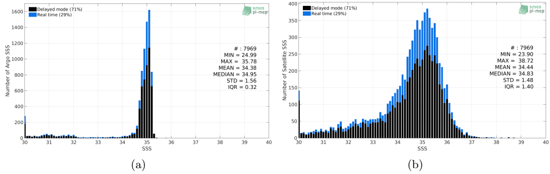
Figure 2: Histograms of SSS from Argo (a) and SMOS SSS L3 v317 - 10 Days - 25 km (CATDS-CPDC) (b) considering all match-up pairs per bins of 0.1 over the Arctic Ocean Pi-MEP region and for the full satellite product period.
