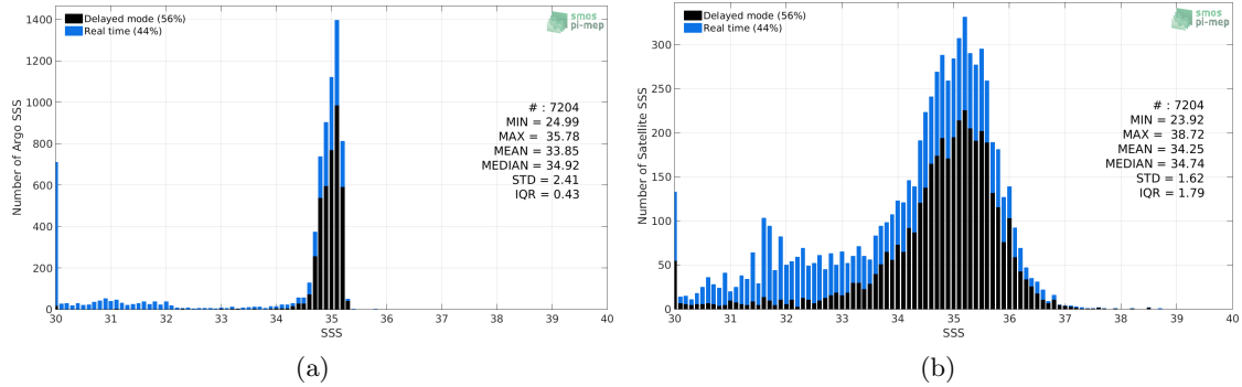
Figure 2: Histograms of SSS from Argo (a) and SMOS L3 v317 - 10 Days - 25 km (CATDS-CPDC) (b) considering all match-up pairs per bins of 0.1 over the Arctic Ocean Pi-MEP region and for the full satellite product period.
