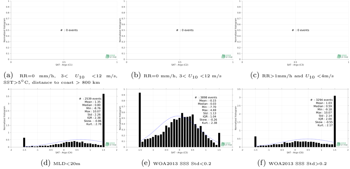
Figure 13: Normalized histogram of \Delta SSS (SMOS L3 v317 - 10 Days - 25 km (CATDS-CPDC) - Argo) for 6 different subdatasets corresponding to: RR=0 mm/h, 3 < U_{10} < 12 m/s, SST > 5^\circ\text{C} , distance to coast > 800 km (a), RR=0 mm/h, 3 < U_{10} < 12 m/s (b), RR > 1\text{mm/h} and U_{10} < 4\text{m/s} (c), MLD < 20\text{m} (d), WOA2013 SSS Std < 0.2 (e), WOA2013 SSS Std > 0.2 (f).
