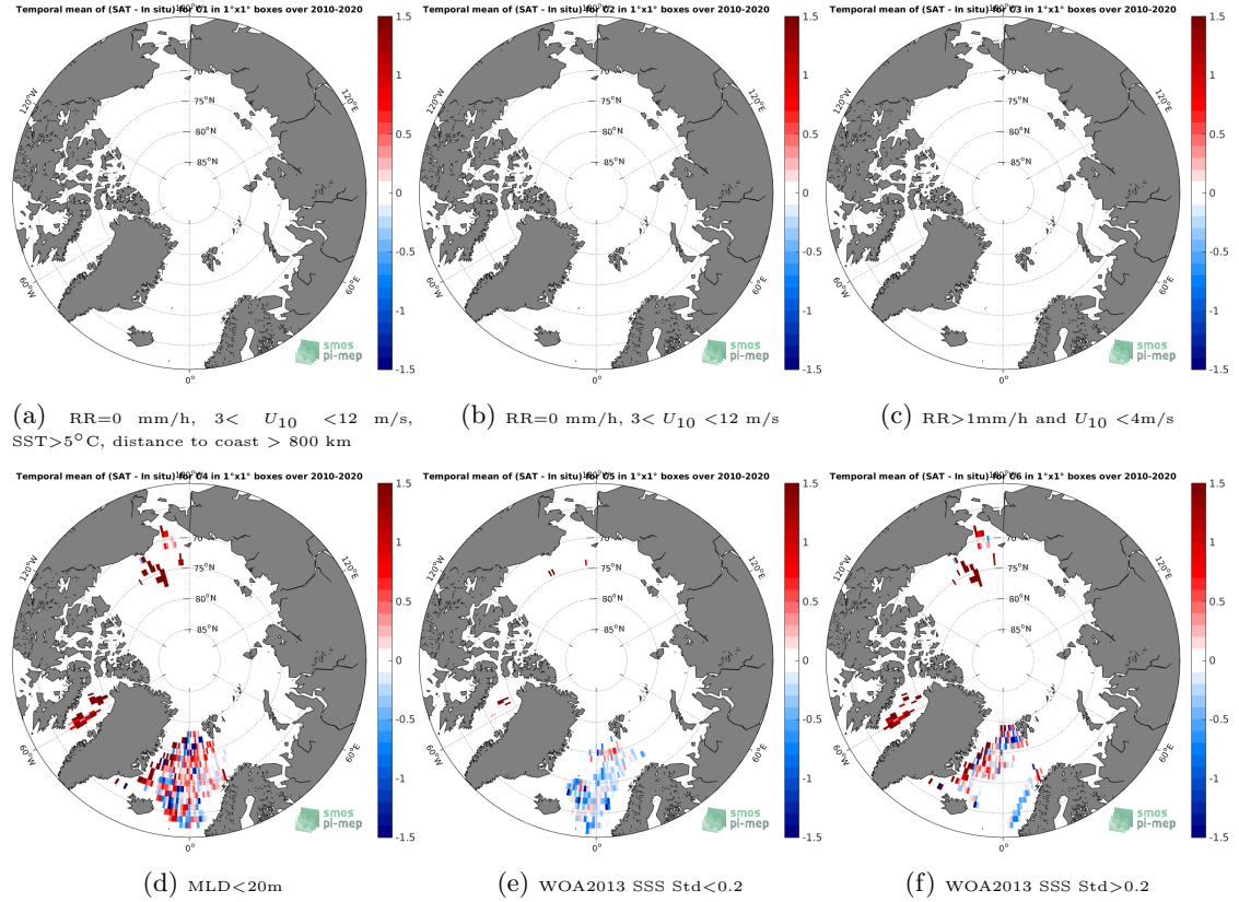
Figure 12: Temporal mean gridded over spatial boxes of size 1^{\circ}\times 1^{\circ} of \Delta\text{SSS} (SMOS L3 v317 - 10 Days - 25 km (CATDS-CPDC) - Argo) for 6 different subdatasets corresponding to: RR=0 mm/h, 3 < U_{10} < 12 m/s, SST >5^{\circ}\text{C} , distance to coast > 800 km (a), RR=0 mm/h, 3 < U_{10} < 12 m/s (b), RR >1 mm/h and U_{10} < 4 m/s (c),MLD <20 m (d),WOA2013 SSS Std <0.2 (e),WOA2013 SSS Std >0.2 (f).
