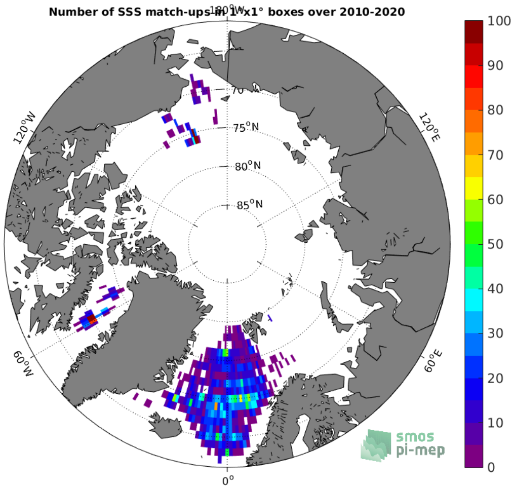
Figure 4: Number of SSS match-ups between Argo SSS and the SMOS L3 v317 - 10 Days - 25 km (CATDS-CPDC) SSS product for the Arctic Ocean Pi-MEP region over 1^\circ \times 1^\circ boxes and for the full satellite product period.
