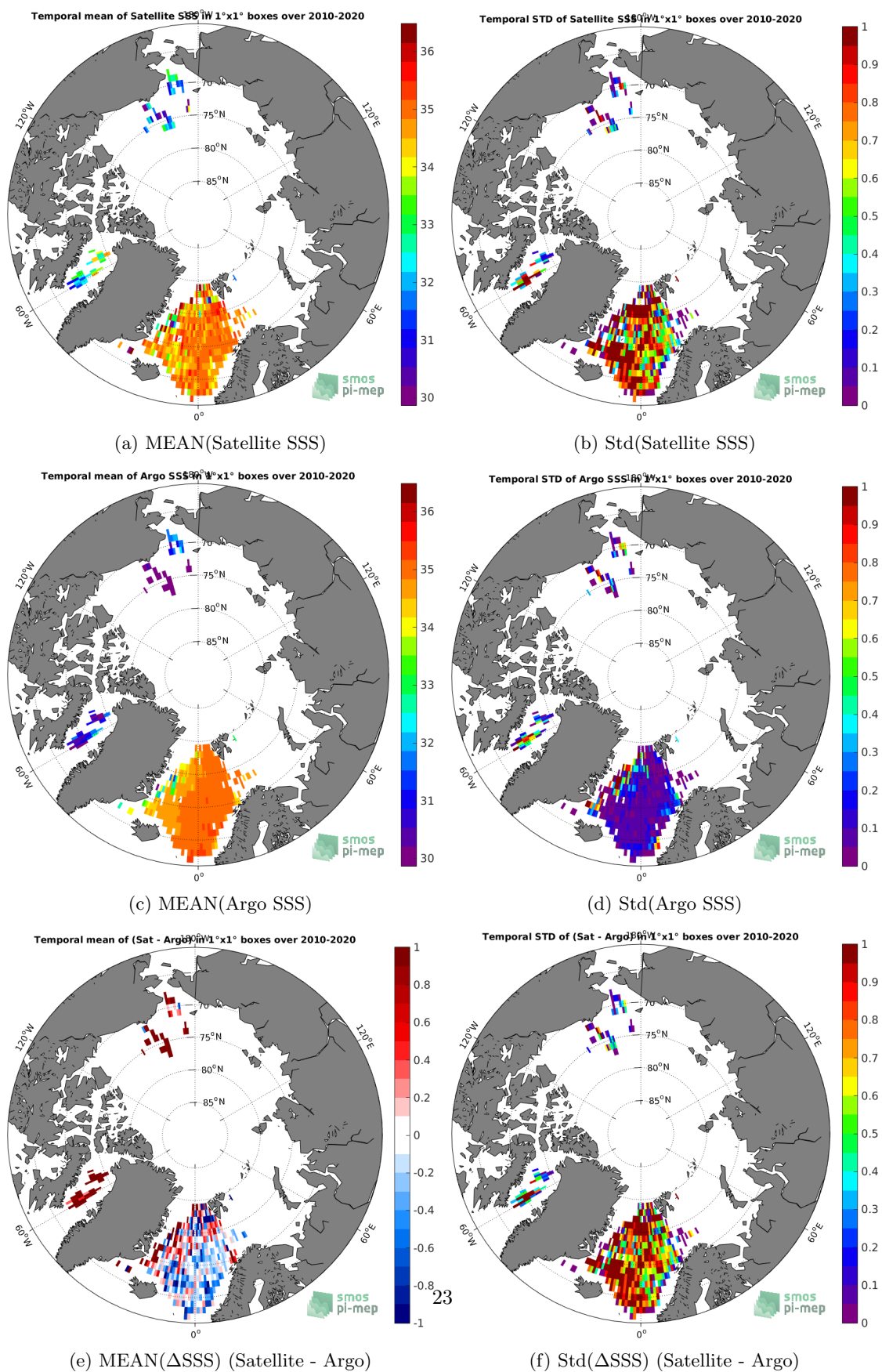
Figure 6: Temporal mean (left) and Std (right) of SSS from SMOS L3 v317 - 10 Days - 25 km (CATDS-CPDC) (top), Argo (middle), and of ΔSSS (Satellite - Argo). Only match-up pairs are used to generate these maps.
