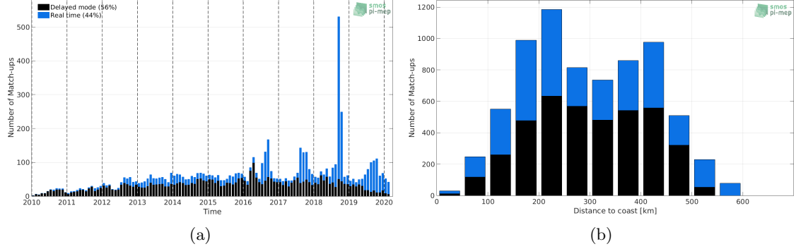
Figure 1: Number of match-ups between Argo and SMOS L3 v317 - 10 Days - 25 km (CATDS-CPDC) SSS as a function of time (a) and as function of the distance to coast (b) over the Arctic Ocean Pi-MEP region and for the full satellite product period.
