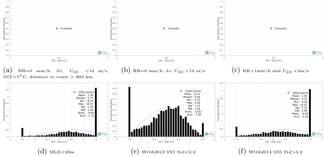
Figure 13: Normalized histogram of \Delta SSS (SMOS-L3-CATDS-CPDC-V317-10DAYS-25KM - Argo) for 6 different subdatasets corresponding to: RR=0 mm/h, 3 < U_{10} < 12 m/s, SST > 5^\circ\text{C} , distance to coast > 800 km (a), RR=0 mm/h, 3 < U_{10} < 12 m/s (b), RR > 1\text{mm/h} and U_{10} < 4\text{m/s} (c), MLD < 20\text{m} (d), WOA2013 SSS Std < 0.2 (e), WOA2013 SSS Std > 0.2 (f).
