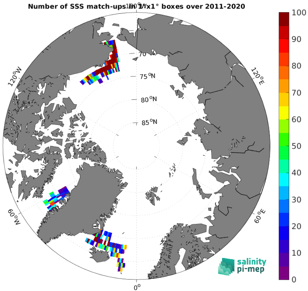
Figure 5: Number of SSS match-ups between TSG (SAMOS) SSS and the SMOS SSS L3 v2 - 9-Days (BEC) SSS product for the Arctic Ocean Pi-MEP region over 1^\circ \times 1^\circ boxes and for the full satellite product period.
