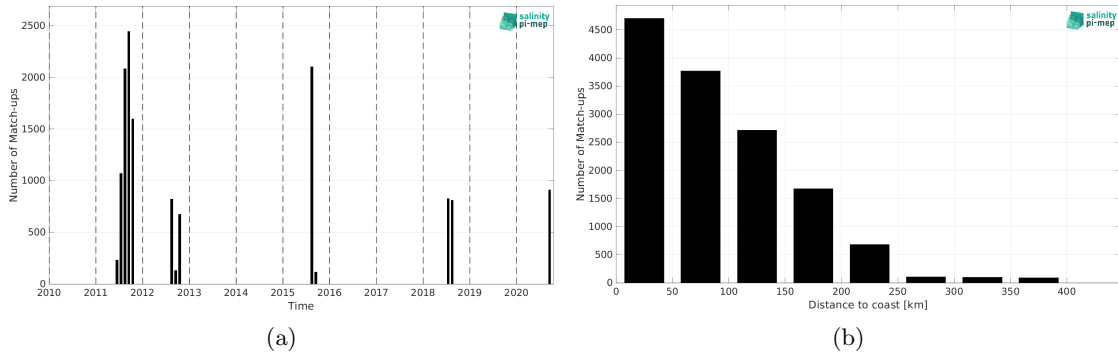
Figure 2: Number of match-ups between TSG (SAMOS) and SMOS SSS L3 v2 - 9-Days (BEC) SSS as a function of time (a) and as function of the distance to coast (b) over the Arctic Ocean Pi-MEP region and for the full satellite product period.
