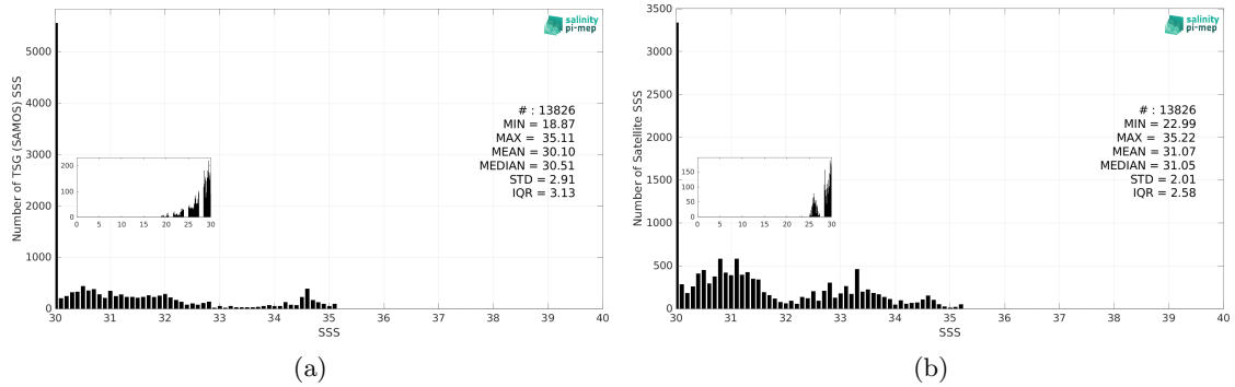
Figure 3: Histograms of SSS from TSG (SAMOS) (a) and SMOS SSS L3 v2 - 9-Days (BEC) (b) considering all match-up pairs per bins of 0.1 over the Arctic Ocean Pi-MEP region and for the full satellite product period.
