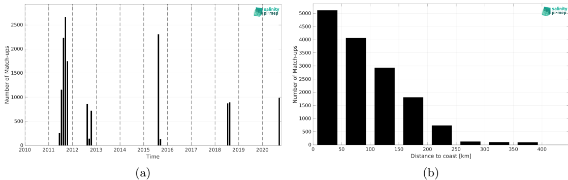
Figure 1: Number of match-ups between TSG (SAMOS) and SMOS SSS L3 v2 - 9-Days (BEC) SSS as a function of time (a) and as function of the distance to coast (b) over the Arctic Ocean Pi-MEP region and for the full satellite product period.
