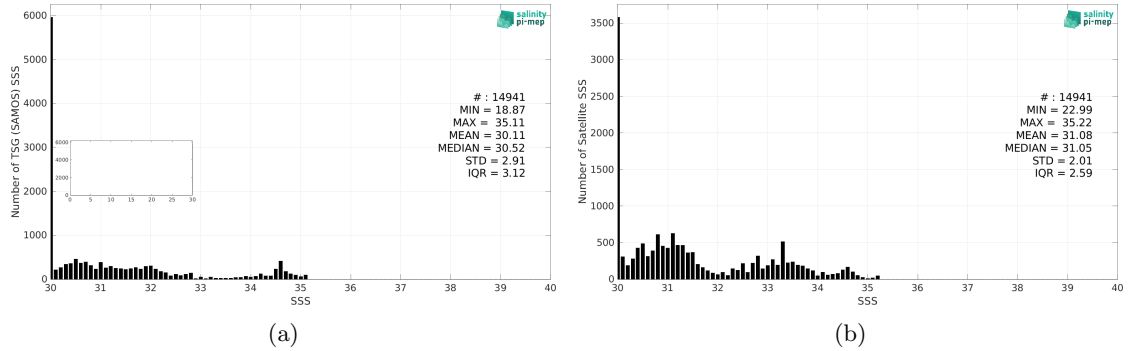
Figure 2: Histograms of SSS from TSG (SAMOS) (a) and SMOS SSS L3 v2 - 9-Days (BEC) (b) considering all match-up pairs per bins of 0.1 over the Arctic Ocean Pi-MEP region and for the full satellite product period.
