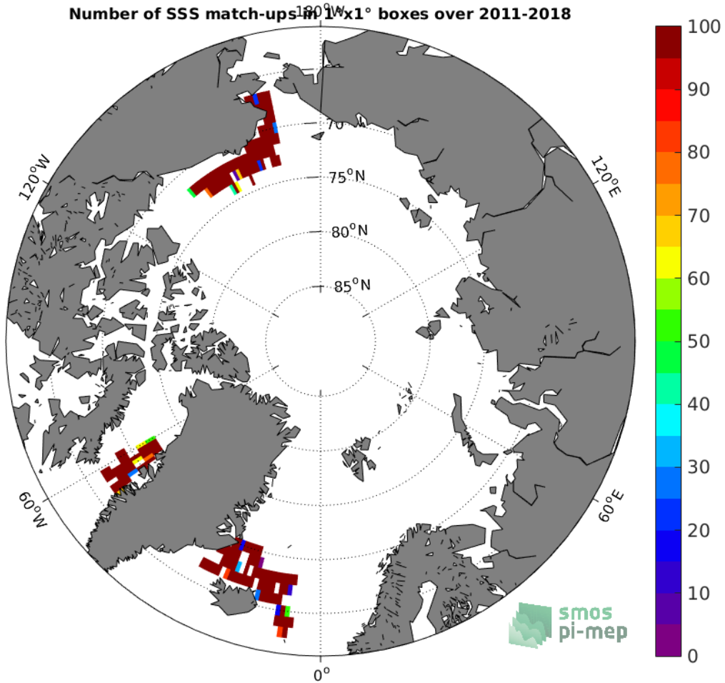
Figure 4: Number of SSS match-ups between TSG (SAMOS) SSS and the SMOS SSS L3 v2 - 9-Days (BEC) SSS product for the Arctic Ocean Pi-MEP region over 1^\circ \times 1^\circ boxes and for the full satellite product period.
